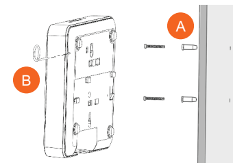
Figure 3. Flat surface mounting
