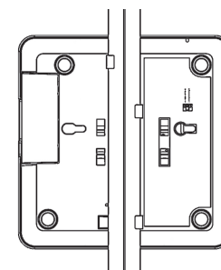
Figure 9. Locking the integrated bracket to the T-bar
