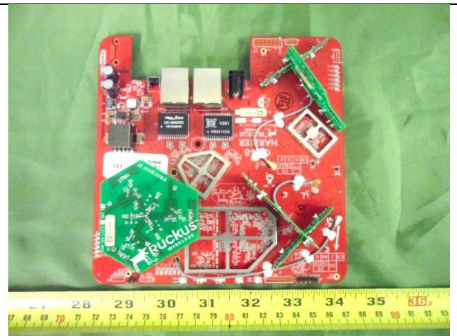
EUT– Top View without Shielding
