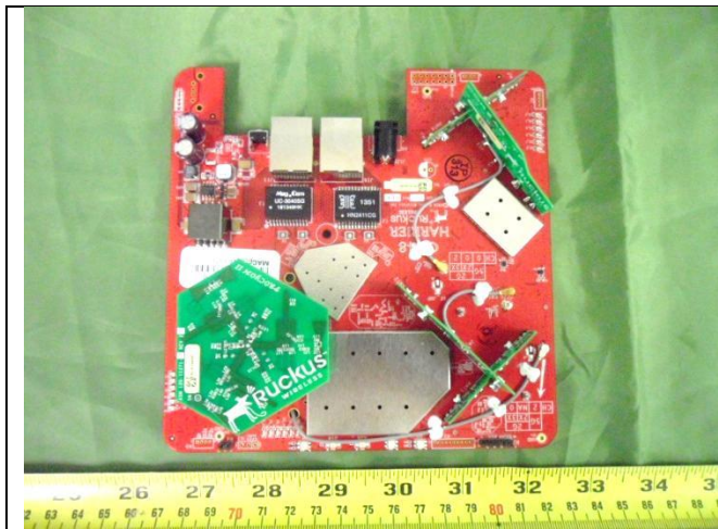
EUT – Top View with Shielding
