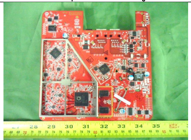
EUT– Bottom View without Shielding
