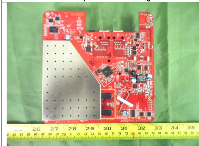
EUT – Bottom View with Shielding
