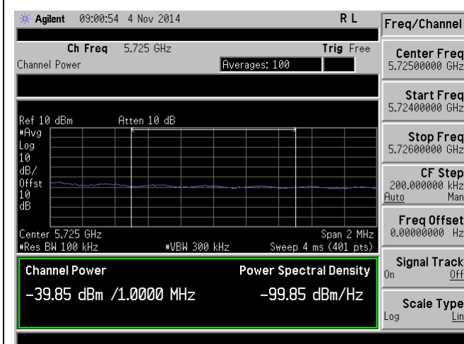
Band Edge-5725M-802.11a@5700M-Chain2
