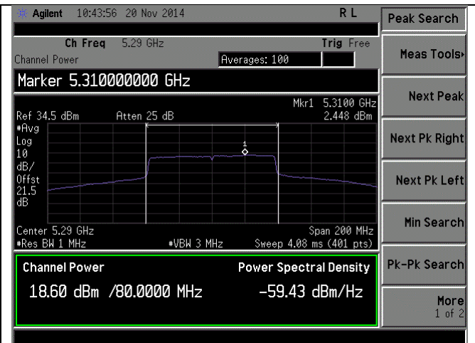
PSD-802.11ac-80M-5290M-chain1
