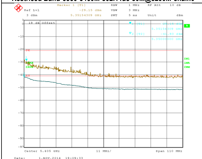
Restrictd Band-5350-5460M-802.11ac-80M@5290M-chain2
