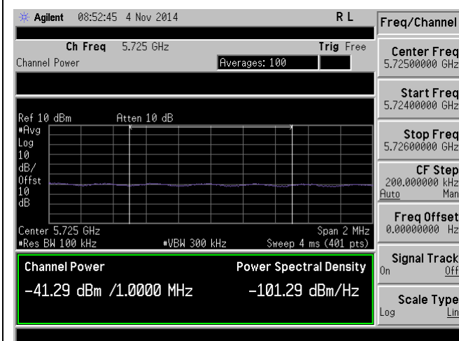
Band Edge-5725M-802.11n-40M@5670M-Chain2
