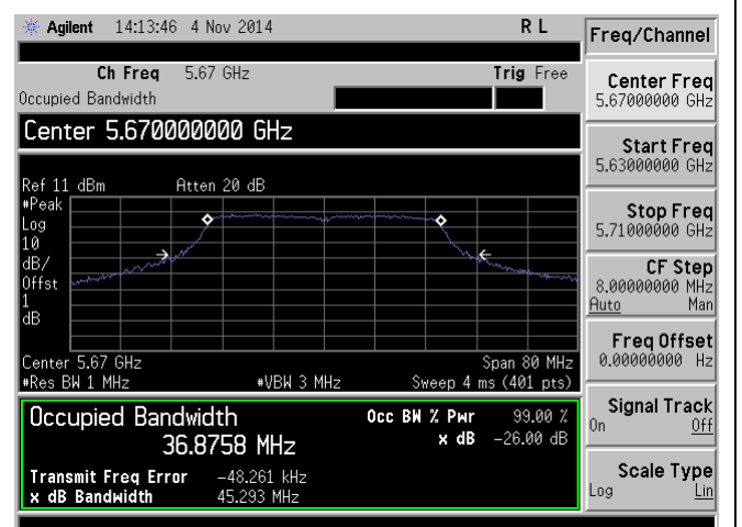
26dB BW -802.11n-40M 5670MHz
