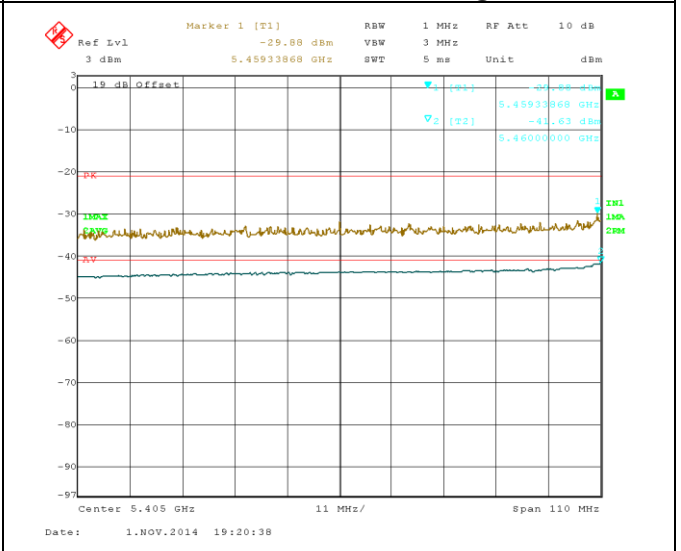
Restrictd Band-5350-5460M-802.11n-40M@5510M-chain2
