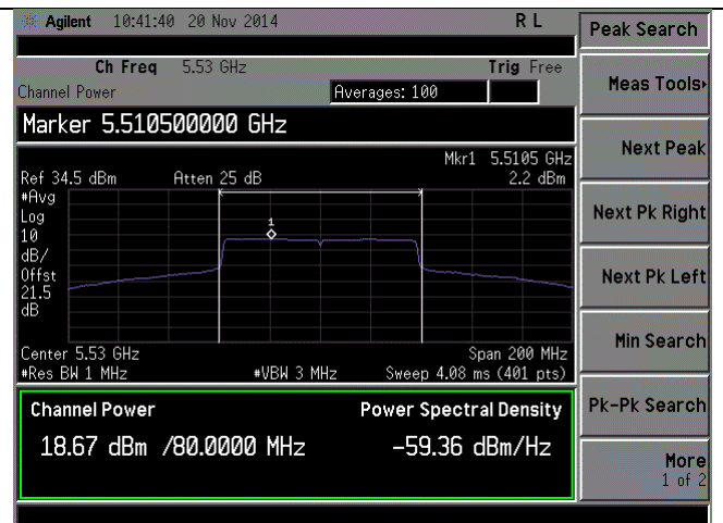
PSD-802.11ac-80M-5530M-chain0
