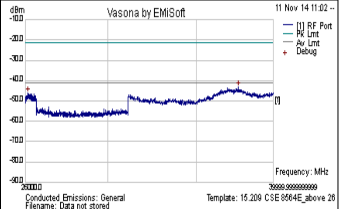
CSE-802.11n-40M-5310MHz-above 26GHz-chain2
