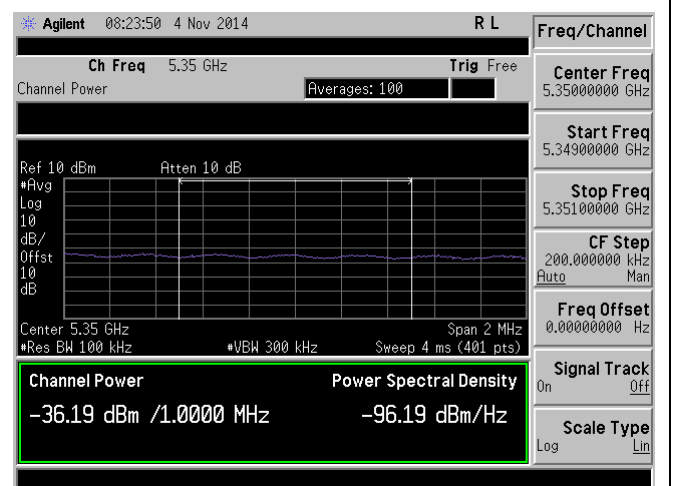
Band Edge-5350M-802.11n-20M@5320M-Chain2
