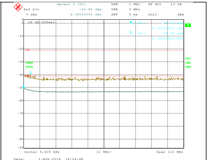
Restrictd Band-5350-5460M-802.11n-40M@5310M-chain1
