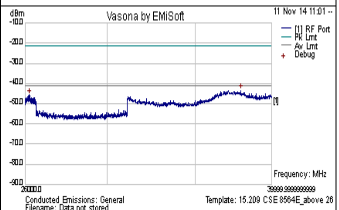
CSE-802.11n-40M-5310MHz-above 26GHz-chain1
