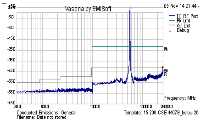
CSE-802.11ac-80M-5610MHz-below 26GHz-chain1
