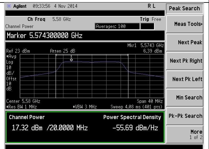
PSD-802.11a-5580M-chain0
