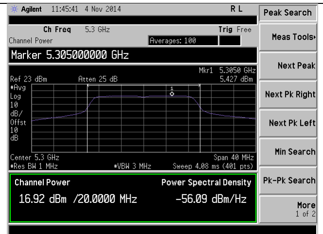
PSD-802.11n-20M-5300M-chain1
