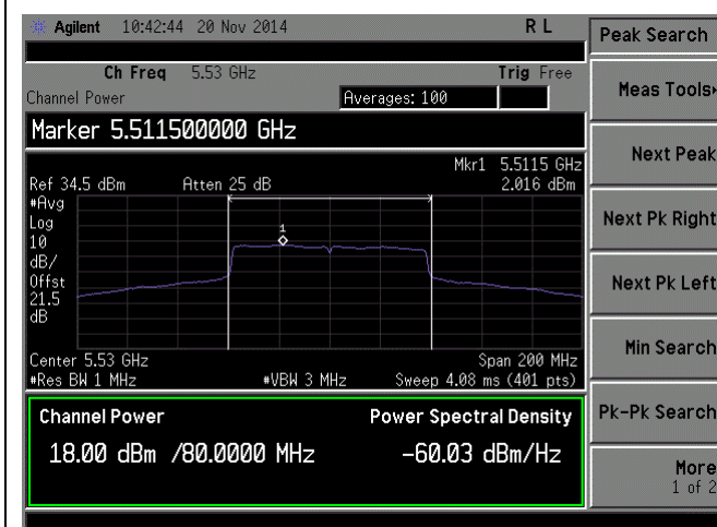
PSD-802.11ac-80M-5530M-chain1
