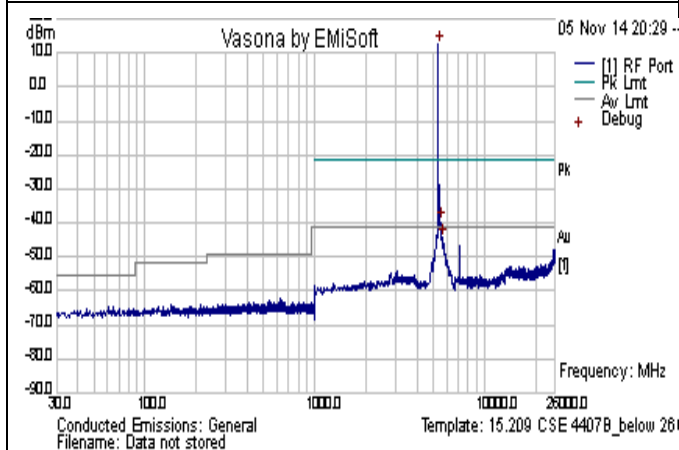
CSE-802.11a 5320MHz-below 26GHz-chain2
