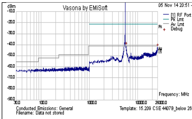
CSE-802.11n-20M-5500MHz-below 26GHz-chain0
