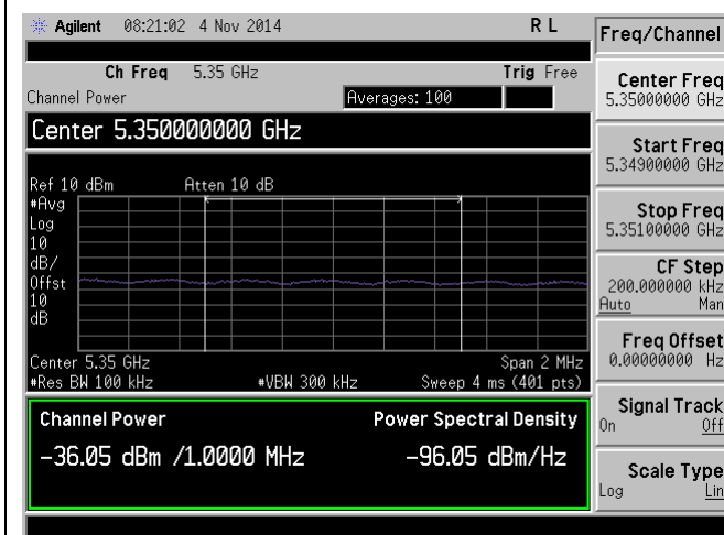
Band Edge-5350M-802.11n-20M@5320M-Chain1
