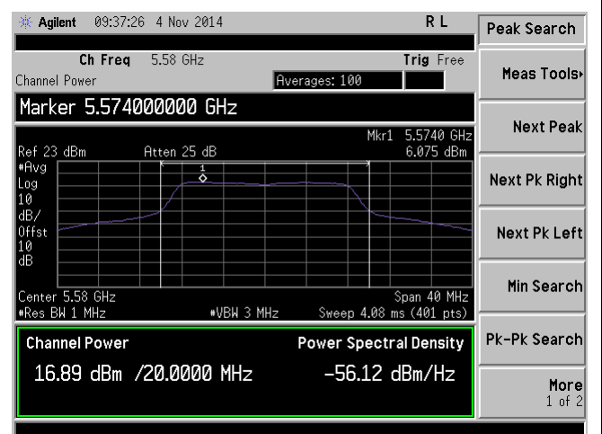
PSD-802.11a-5580M-chain2
