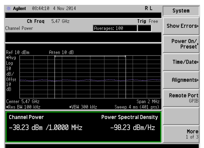
Band Edge-5470M-802.11n-40M@5510M-Chain2
