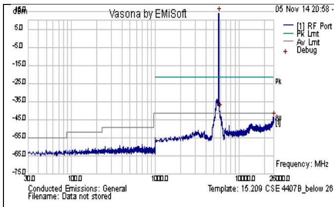
CSE-802.11n-20M-5700MHz-below 26GHz-chain0
