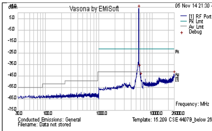
CSE-802.11n-40M-5590MHz-below 26GHz-chain0
