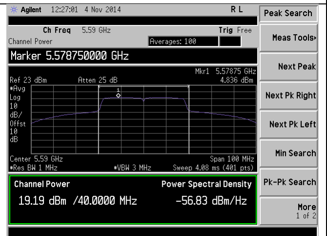
PSD-802.11n-40M-5590M-chain0
