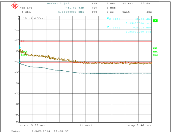
Restrictd Band-5350-5460M-802.11ac-80M@5290M-chain1
