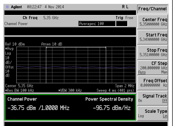
Band Edge-5350M-802.11n-20M@5320M-Chain0
