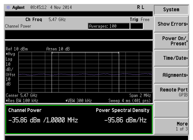
Band Edge-5470M-802.11n-40M@5510M-Chain0
