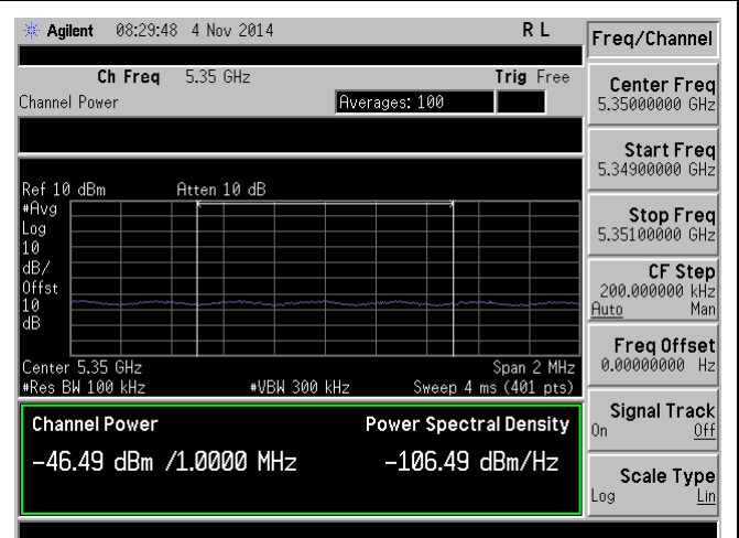
Band Edge-5350M-802.11ac-80M@5290M-Chain2
