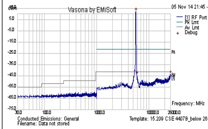
CSE-802.11ac-80M-5610MHz-below 26GHz-chain2
