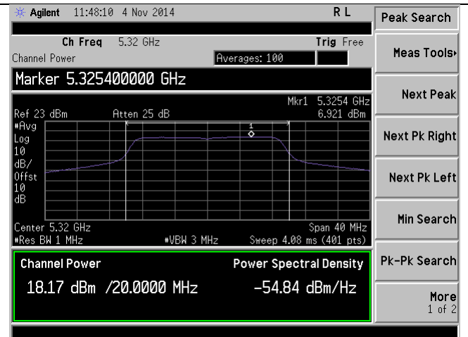
PSD-802.11n-20M-5320M-chain0
