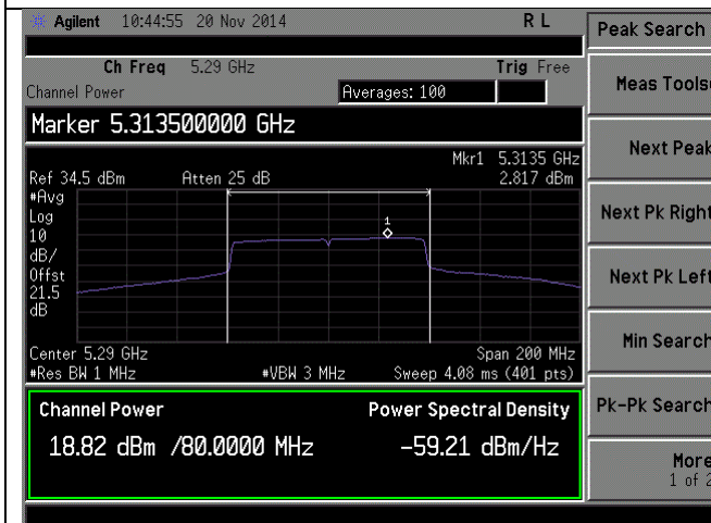
PSD-802.11ac-80M-5290M-chain2
