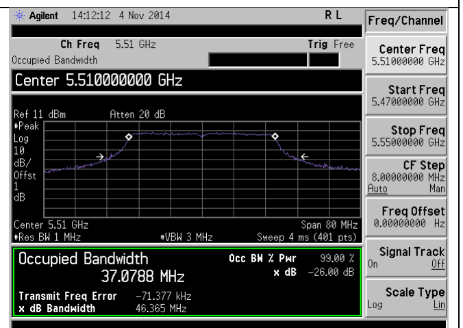
26dB BW -802.11n-40M 5510MHz
