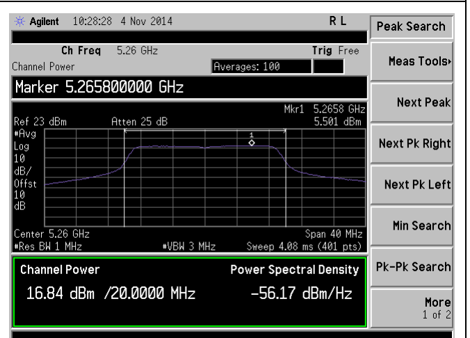
PSD-802.11n-20M-5260M-chain2
