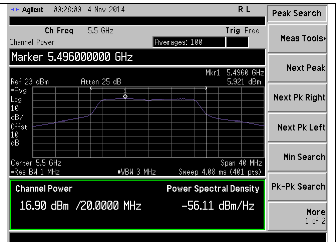
PSD-802.11a-5500M-chain1
