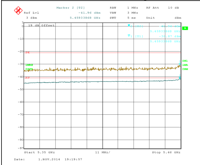
Restrictd Band-5350-5460M-802.11n-40M@5510M-chain1
