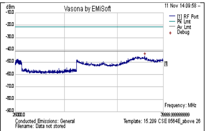
CSE-802.11n-40M-5270MHz-above 26GHz-chain0
