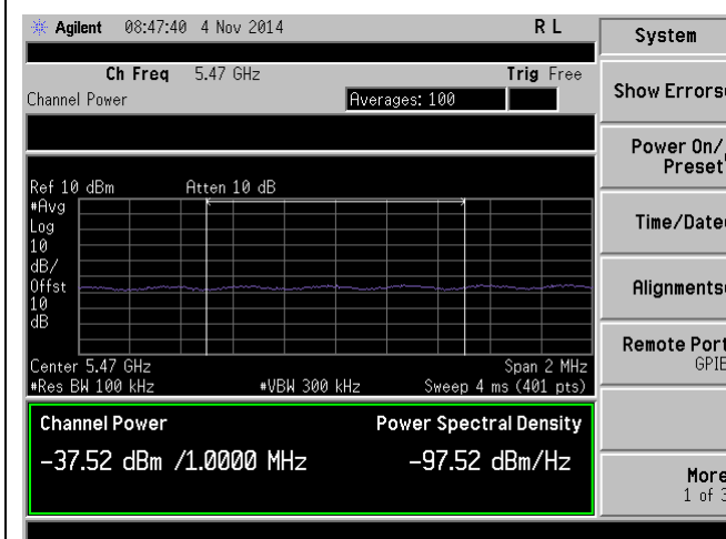
Band Edge-5470M-802.11ac-80M@5530M-Chain2
