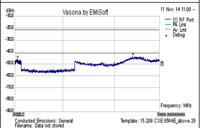
CSE-802.11n-40M-5270MHz-above 26GHz-chain2
