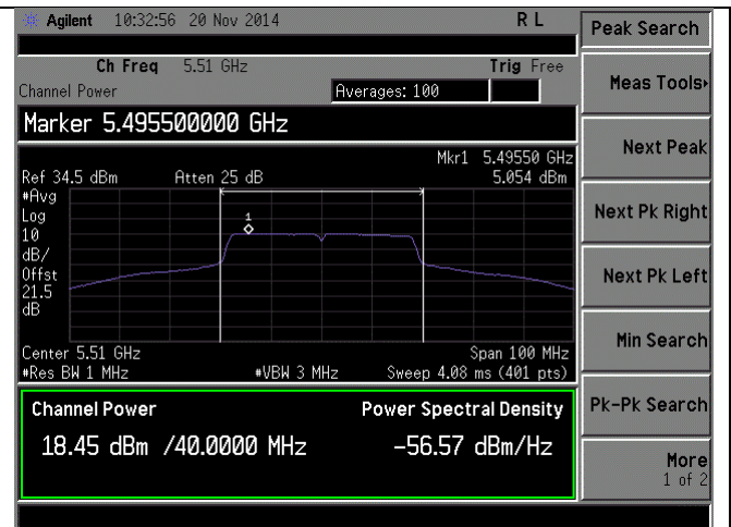
PSD-802.11n-40M-5510M-chain1
