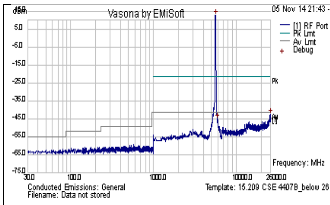
CSE-802.11ac-80M-5610MHz-below 26GHz-chain0
