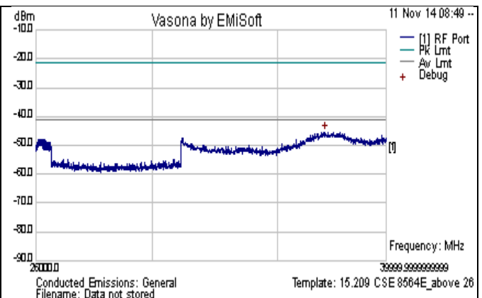
CSE-802.11n-20M-5500MHz-above 26GHz-chain0
