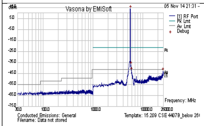
CSE-802.11n-40M-5590MHz-below 26GHz-chain1
