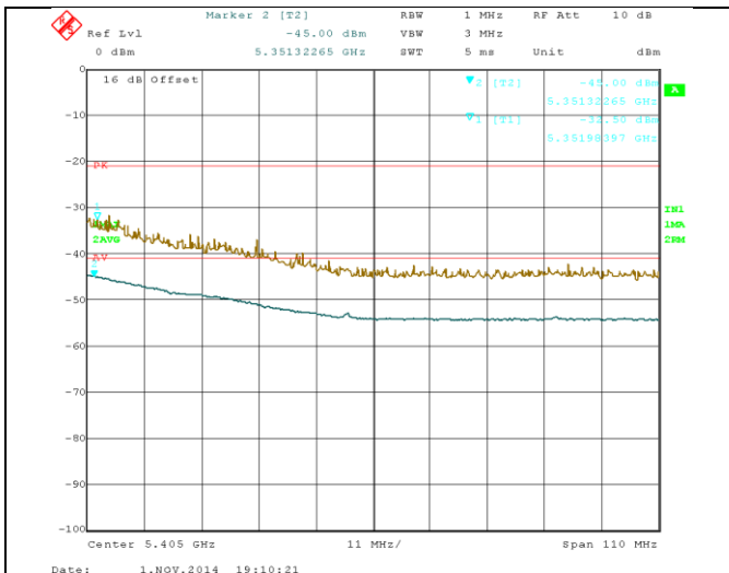
Restrictd Band-5350-5460M-802.11ac-80M@5290M-chain0
