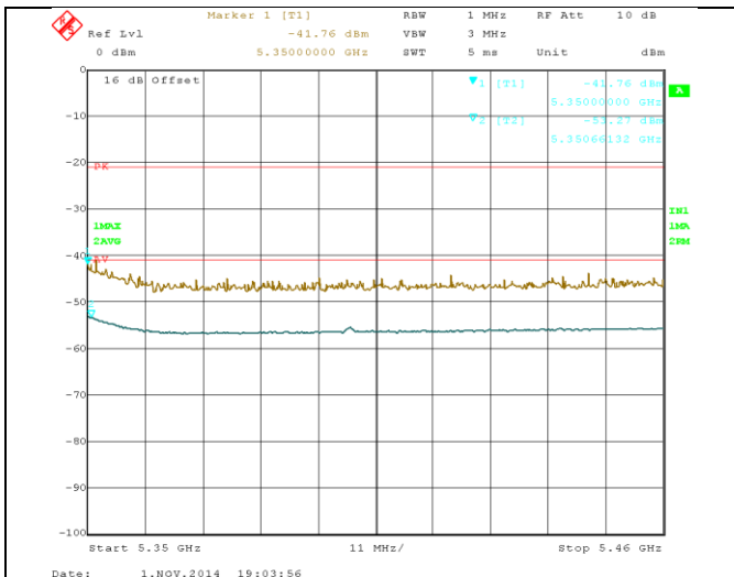
Restrictd Band-5350-5460M-802.11n-40M@5310M-chain0
