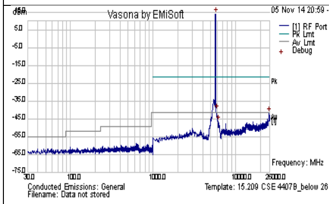
CSE-802.11n-20M-5700MHz-below 26GHz-chain1
