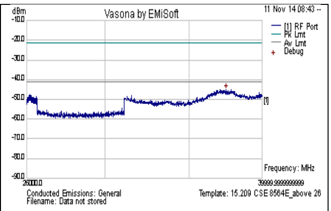
CSE-802.11n-20M-5260MHz-above 26GHz-chain0
