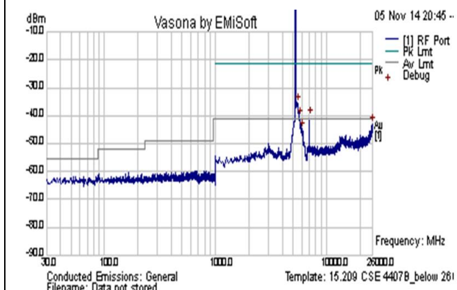
CSE-802.11n-20M-5300MHz-below 26GHz-chain2
