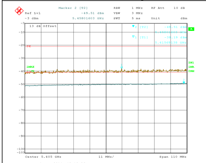
Restrictd Band-5350-5460M-802.11a@5500M-chain1
