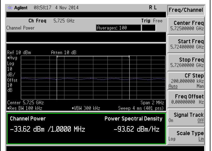
Band Edge-5725M-802.11ac-80M@5610M-Chain0
