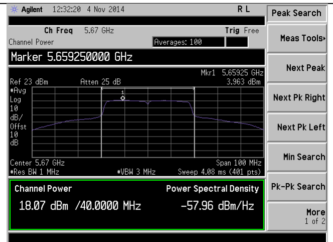
PSD-802.11n-40M-5670M-chain1
