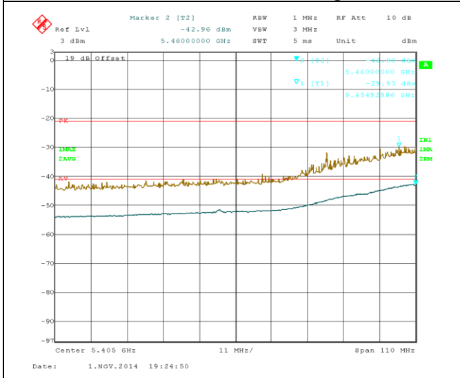
Restrictd Band-5350-5460M-802.11ac-80M@5530M-chain1
