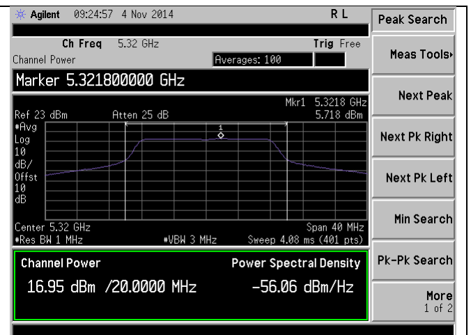
PSD-802.11a-5320M-chain1
