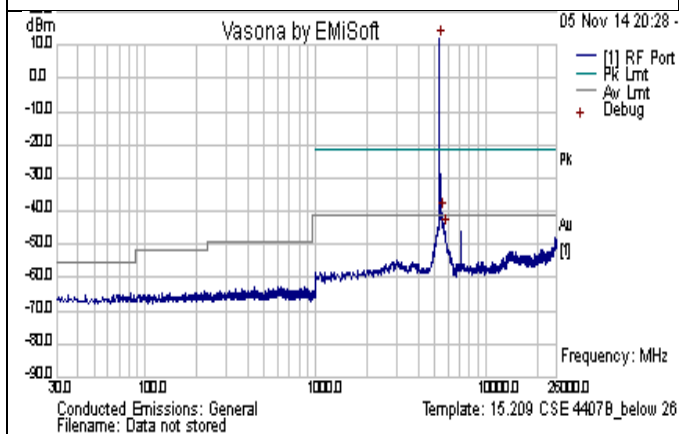
CSE-802.11a 5320MHz-below 26GHz-chain1
