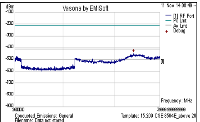
CSE-802.11n-20M-5580MHz-above 26GHz-chain0
