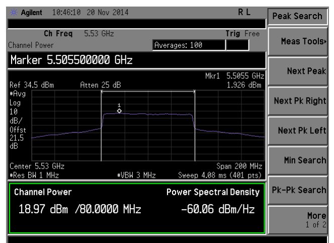
PSD-802.11ac-80M-5530M-chain2
