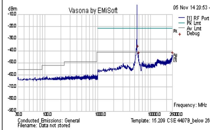
CSE-802.11n-20M-5500MHz-below 26GHz-chain2
