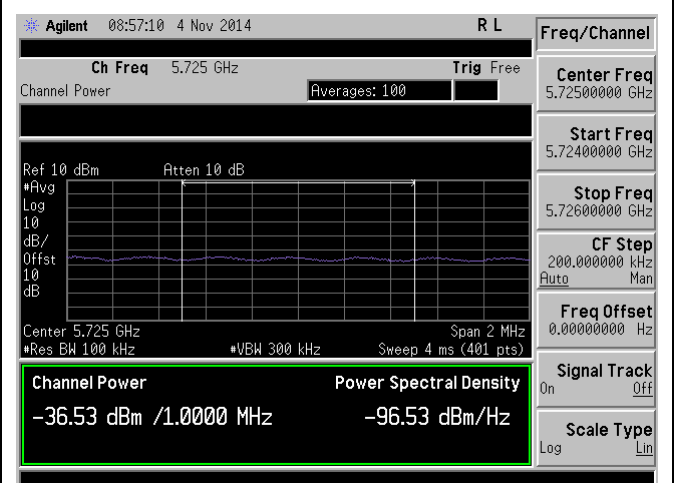
Band Edge-5725M-802.11ac-80M@5610M-Chain2
