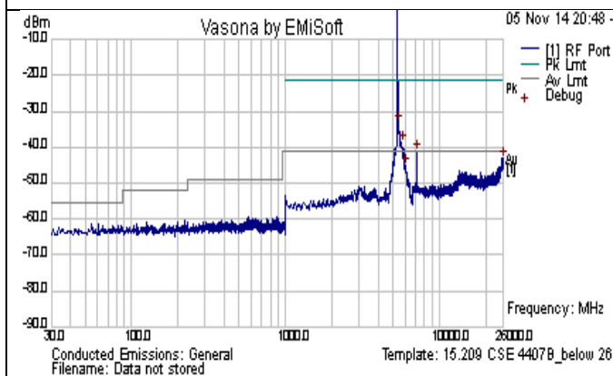
CSE-802.11n-20M-5320MHz-below 26GHz-chain1
