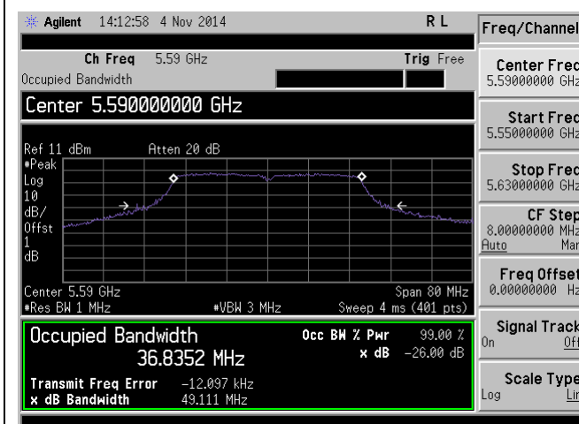
26dB BW -802.11n-40M 5590MHz
