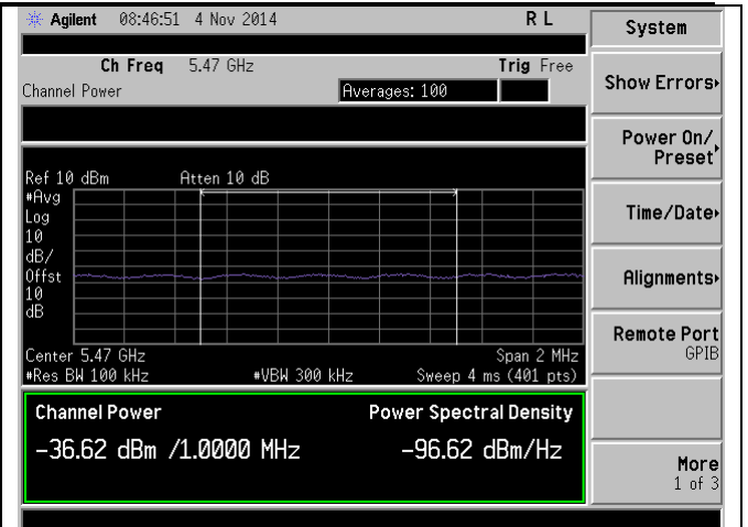
Band Edge-5470M-802.11ac-80M@5530M-Chain1
