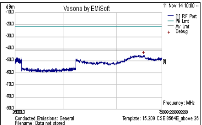
CSE-802.11n-40M-5310MHz-above 26GHz-chain0
