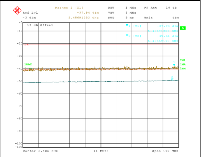
Restrictd Band-5350-5460M-802.11a@5500M-chain2
