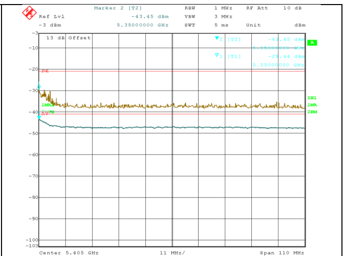
Restrictd Band-5350-5460M-802.11a@5320M-chain1
