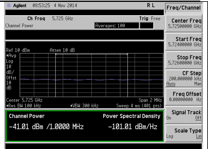
Band Edge-5725M-802.11n-40M@5670M-Chain1
