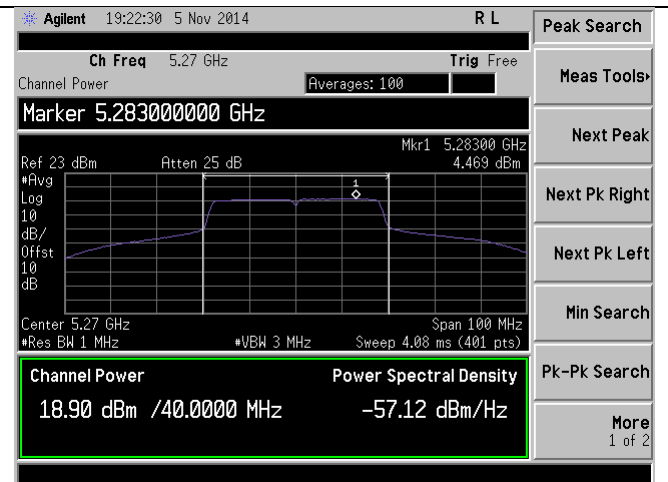
PSD-802.11n-40M-5270M-chain1
