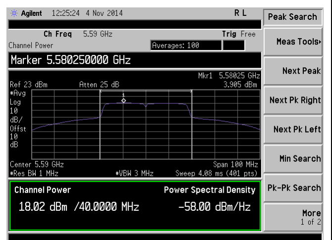
PSD-802.11n-40M-5590M-chain2
