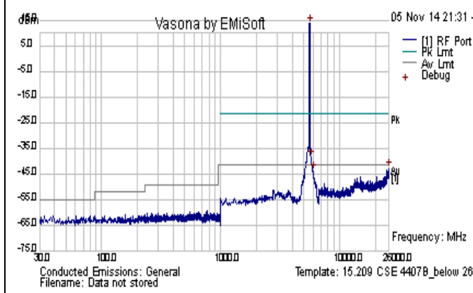
CSE-802.11n-40M-5590MHz-below 26GHz-chain2
