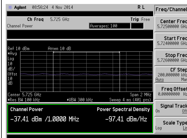
Band Edge-5725M-802.11ac-80M@5610M-Chain1
