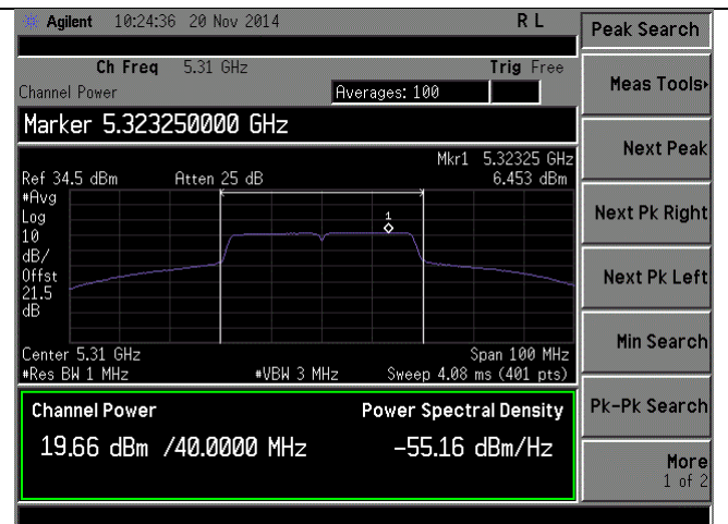
PSD-802.11n-40M-5310M-chain0
