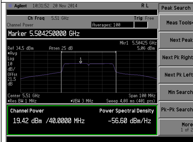
PSD-802.11n-40M-5510M-chain2
