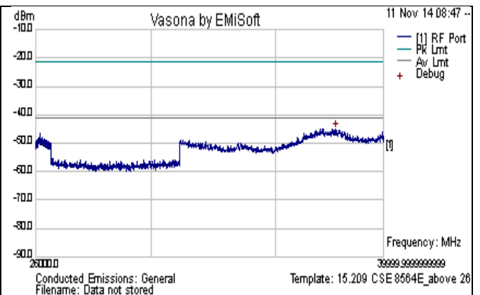
CSE-802.11n-20M-5320MHz-above 26GHz-chain0
