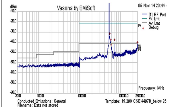
CSE-802.11n-20M-5320MHz-below 26GHz-chain2
