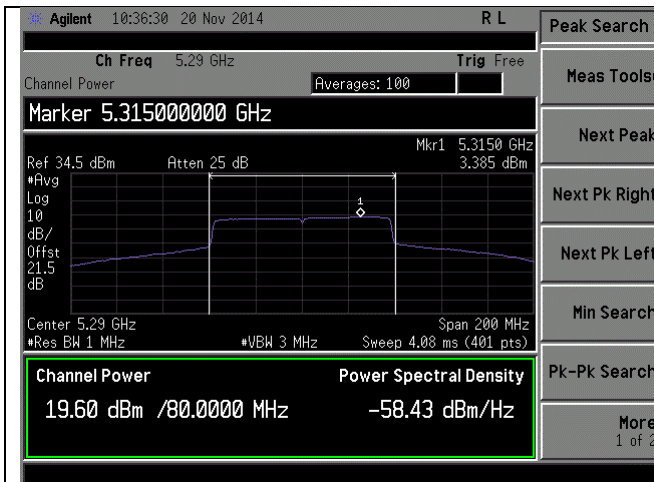
PSD-802.11ac-80M-5290M-chain0
