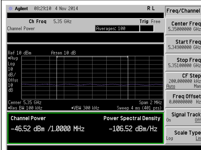
Band Edge-5350M-802.11ac-80M@5290M-Chain1
