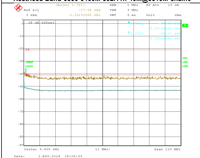
Restrictd Band-5350-5460M-802.11n-40M@5310M-chain2
