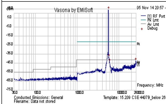
CSE-802.11n-20M-5580MHz-below 26GHz-chain2
