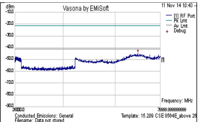
CSE-802.11ac-80M-5610MHz-above 26GHz-chain0
