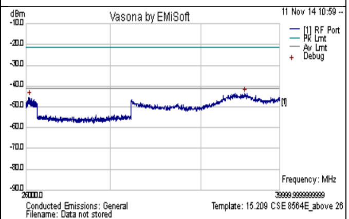
CSE-802.11n-40M-5270MHz-above 26GHz-chain1
