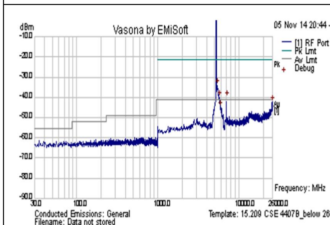
CSE-802.11n-20M-5260MHz-below 26GHz-chain1
