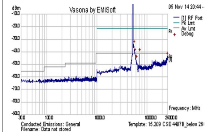
CSE-802.11n-40M-5270MHz-below 26GHz-chain1
