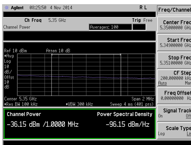
Band Edge-5350M-802.11n-40M@5310M-Chain2
