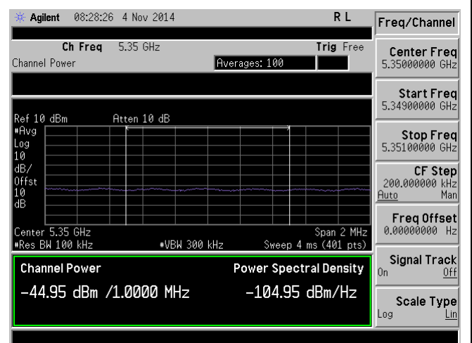
Band Edge-5350M-802.11ac-80M@5290M-Chain0
