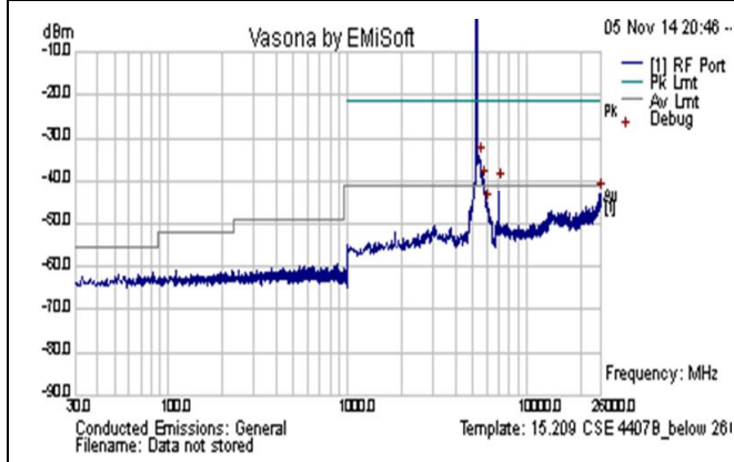
CSE-802.11n-40M-5310MHz-below 26GHz-chain2
