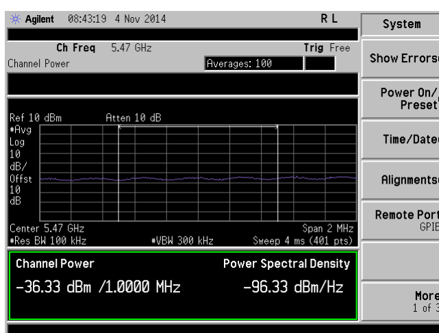
Band Edge-5470M-802.11n-40M@5510M-Chain1
