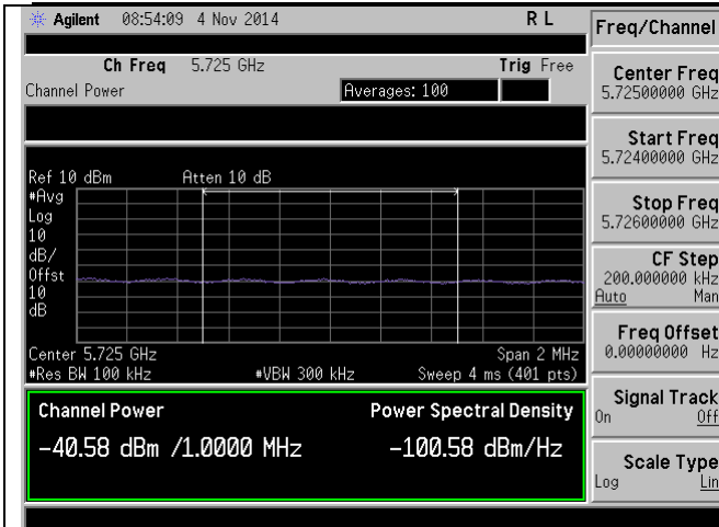
Band Edge-5725M-802.11n-40M@5670M-Chain0
