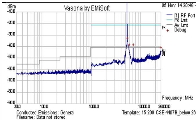
CSE-802.11n-20M-5320MHz-below 26GHz-chain0
