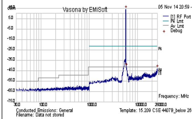
CSE-802.11n-20M-5700MHz-below 26GHz-chain2
