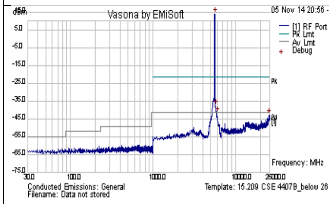
CSE-802.11n-20M-5580MHz-below 26GHz-chain1
