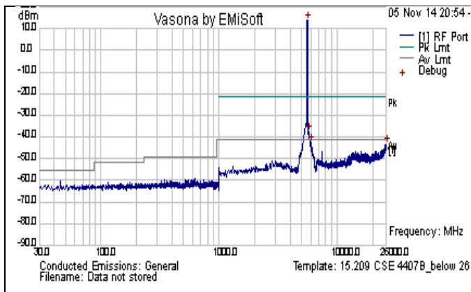
CSE-802.11n-20M-5580MHz-below 26GHz-chain0
