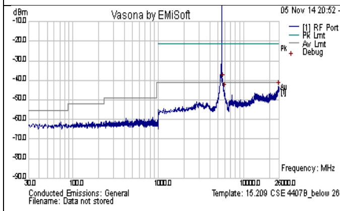
CSE-802.11n-20M-5500MHz-below 26GHz-chain1
