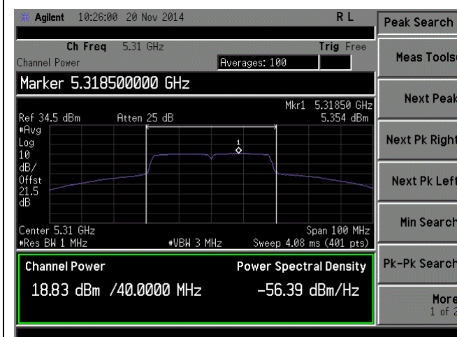
PSD-802.11n-40M-5310M-chain1
