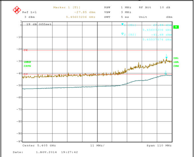
Restrictd Band-5350-5460M-802.11ac-80M@5530M-chain2
