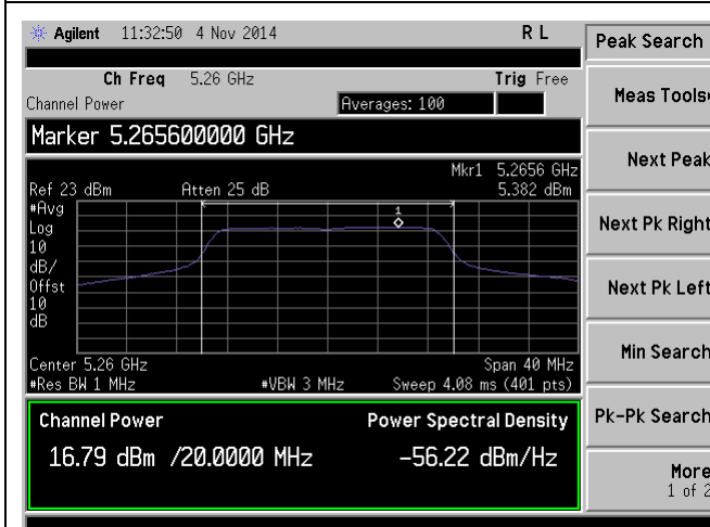
PSD-802.11n-20M-5260M-chain1
