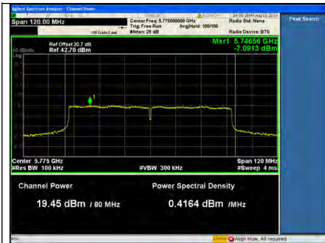
PSD-5.8G-802.11ac-80M Mid-chain0
