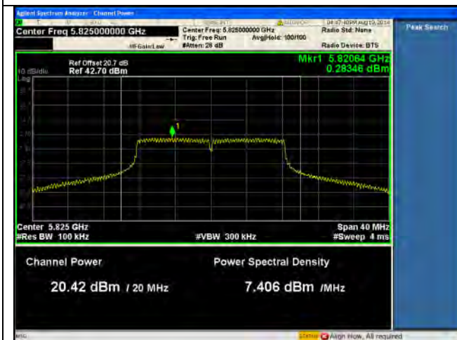
PSD-5.8G-802.11a High-chain2
