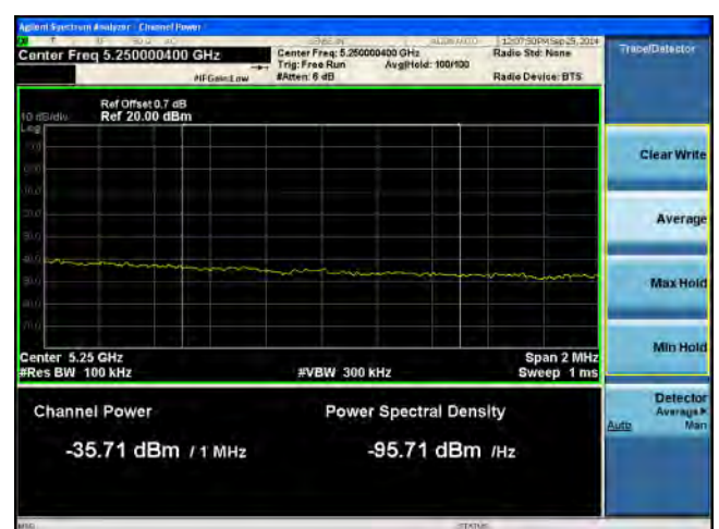
Band Edge-5.1G-802.11n-40M High-Chain2
