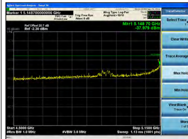
Lower Restricted Band-802.11ac-80-low-chain1
