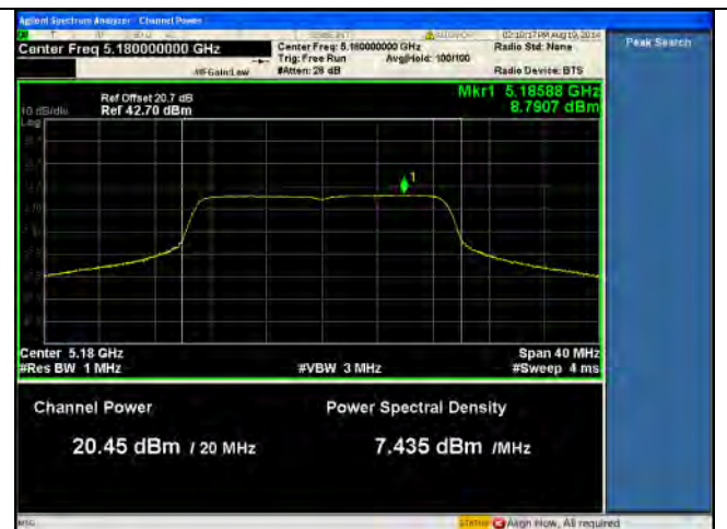
PSD-5.1G-802.11n-20M Low-chain0
