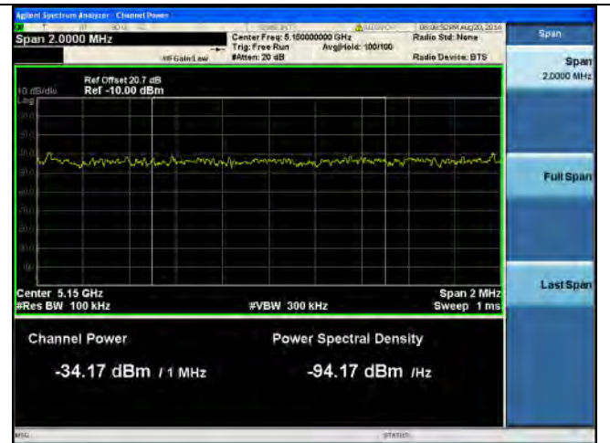
Band Edge-5.1G-802.11a Low-Chain1
