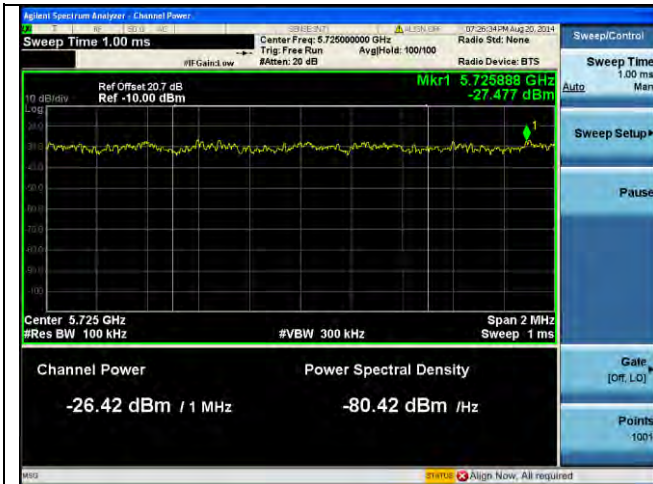
Band Edge-5.8G-802.11ac-80M Low-Chain0
