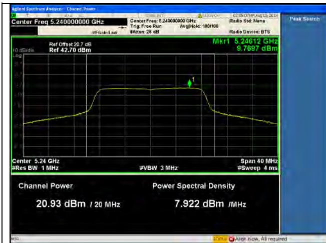
PSD-5.1G-802.11a High-chain0
