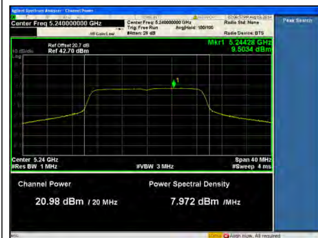
PSD-5.1G-802.11n-20M High-chain1
