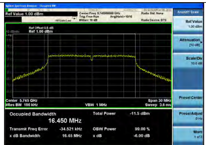
6dB BW -802.11a 5745MHz
