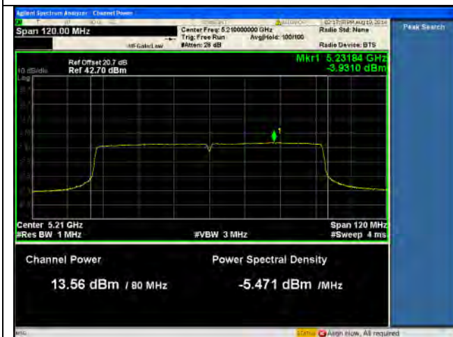
PSD-5.1G-802.11ac-80M Mid-chain2
