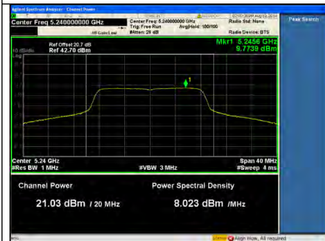
PSD-5.1G-802.11a High-chain2
