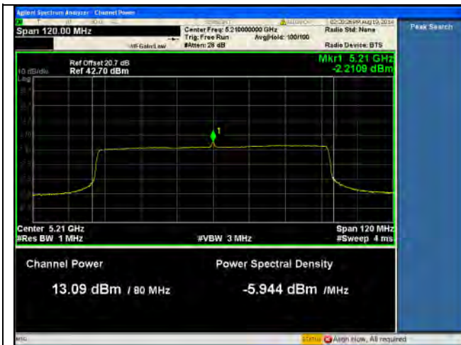
PSD-5.1G-802.11ac-80M Mid-chain0
