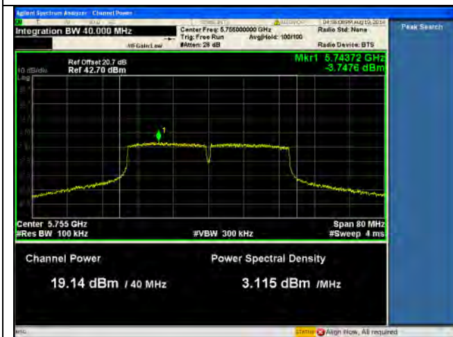
PSD-5.8G-802.11n-40M Low-chain2
