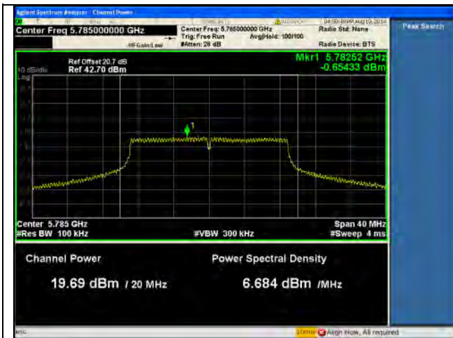
PSD-5.8G-802.11n-20M Mid-chain0
