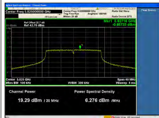
PSD-5.8G-802.11n-20M High-chain1
