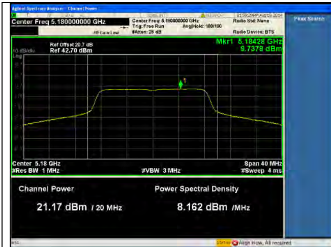
PSD-5.1G-802.11a Low-chain0
