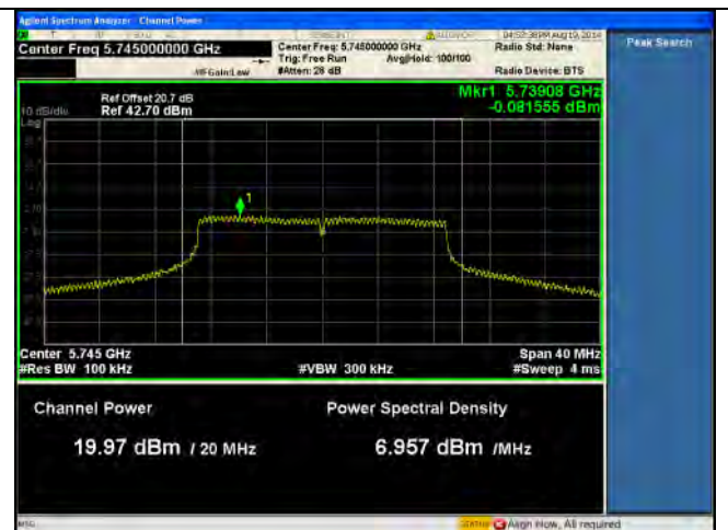
PSD-5.8G-802.11n-20M Low-chain0
