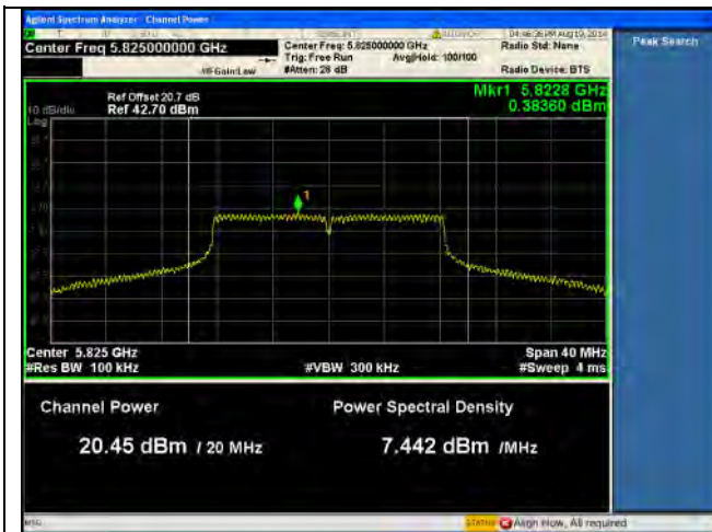
PSD-5.8G-802.11a High-chain0
