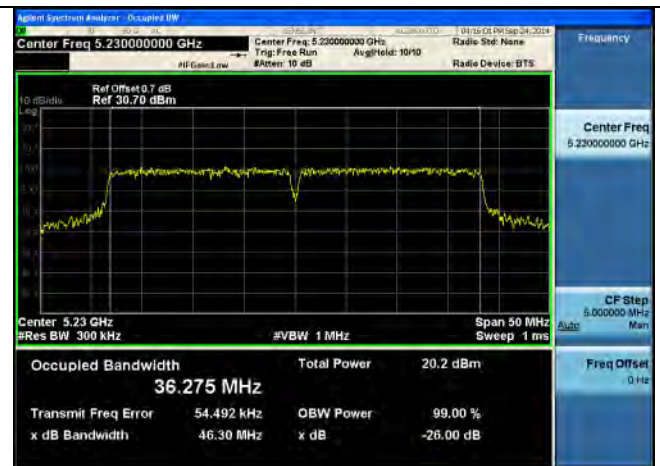
26dB BW -802.11n-40M 5230MHz
