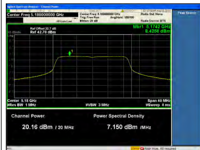
PSD-5.1G-802.11n-20M Low-chain1
