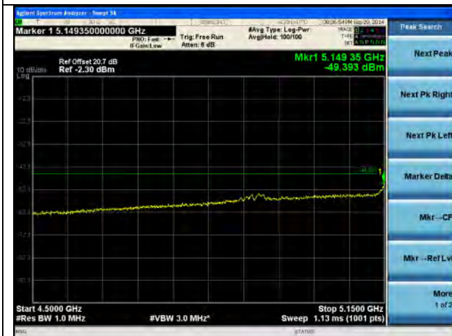
Lower Restrictd Band-802.11a-low-chain2
