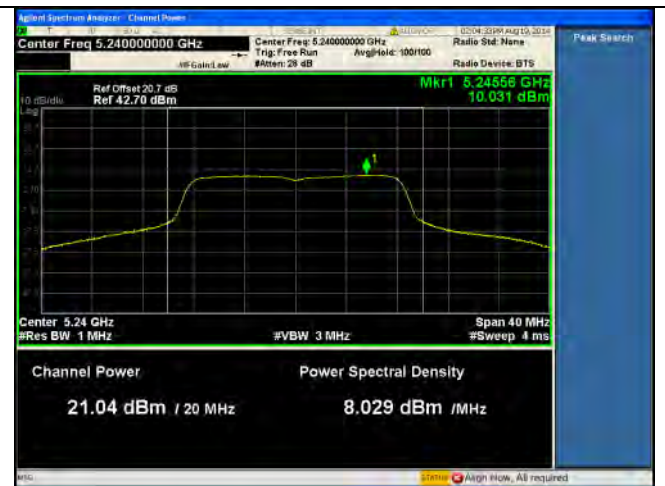
PSD-5.1G-802.11a High-chain1
