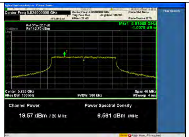
PSD-5.8G-802.11n-20M High-chain0
