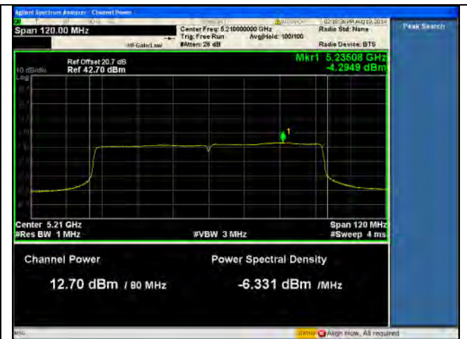
PSD-5.1G-802.11ac-80M Mid-chain1
