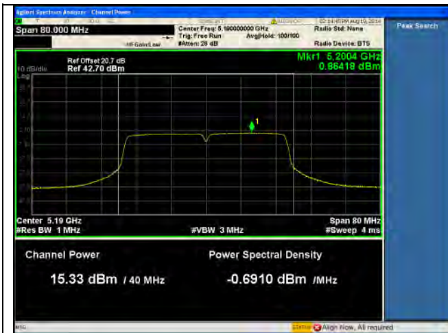
PSD-5.1G-802.11n-40M Low-chain0
