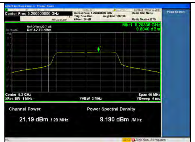
PSD-5.1G-802.11a Mid-chain0
