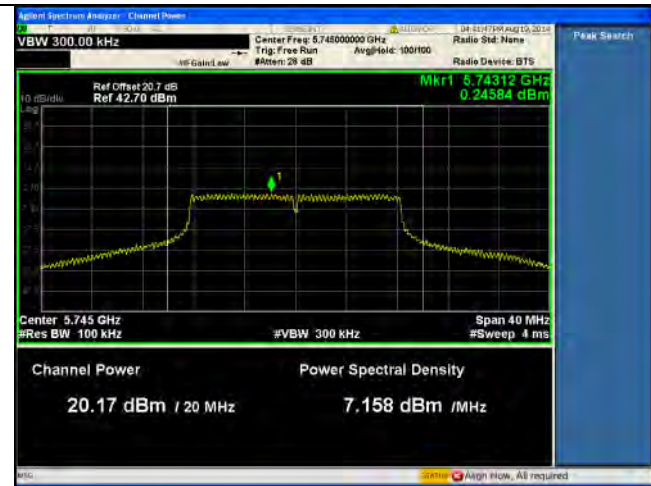
PSD-5.8G-802.11a Low-chain1
