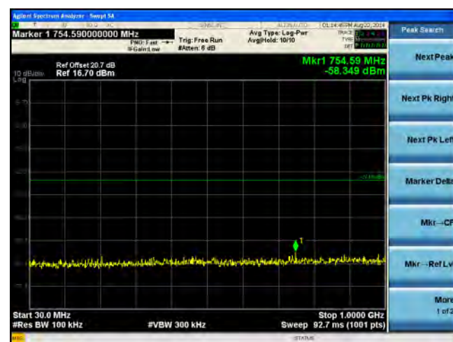
CSE-5.1GHz-Below 1GHz-802.11ac-80M Mid-chain2
