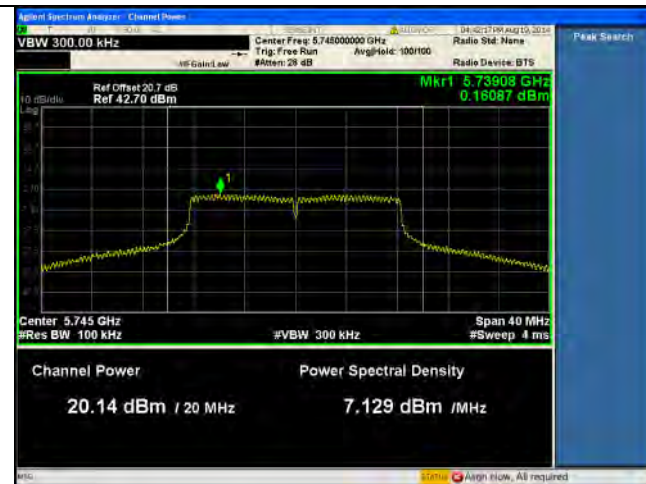
PSD-5.8G-802.11a Low-chain2
