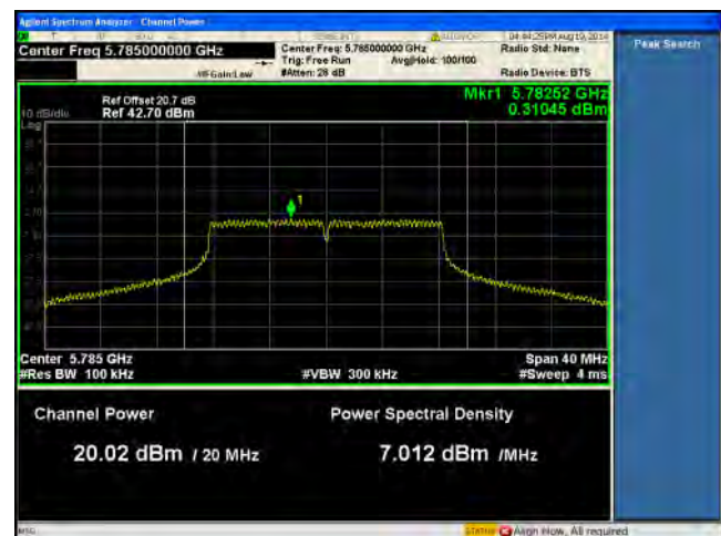
PSD-5.8G-802.11a Mid-chain2
