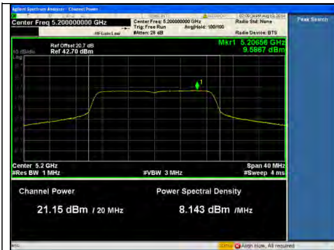
PSD-5.1G-802.11n-20M Mid-chain0
