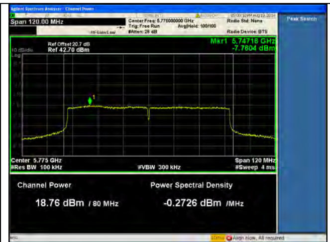
PSD-5.8G-802.11ac-80M Mid-chain1
