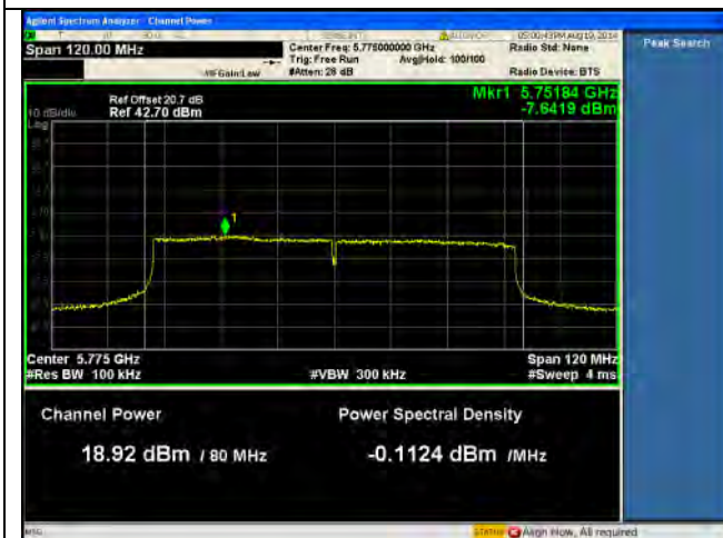
PSD-5.8G-802.11ac-80M Mid-chain2
