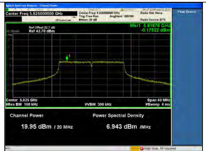
PSD-5.8G-802.11a High-chain1
