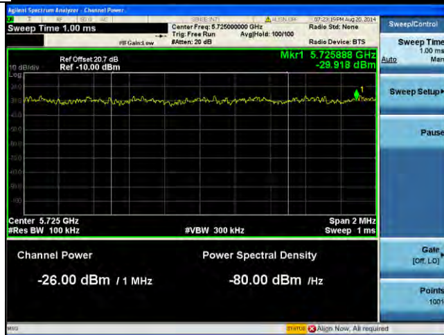
Band Edge-5.8G-802.11n-40M Low-Chain0
