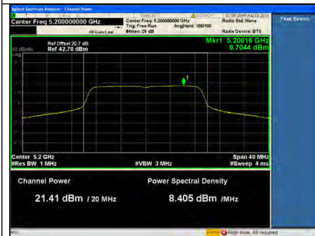
PSD-5.1G-802.11n-20M Mid-chain2
