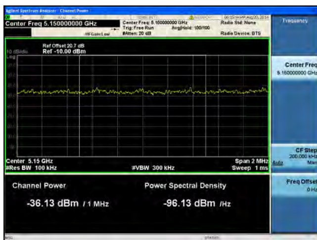
Band Edge-5.1G-802.11n-40M Low-Chain2
