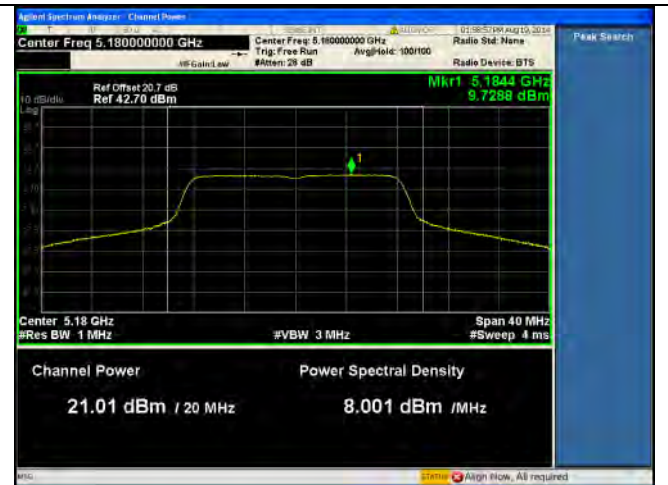
PSD-5.1G-802.11a Low-chain1
