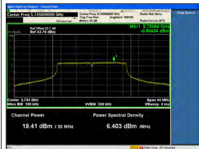
PSD-5.8G-802.11n-20M Low-chain1
