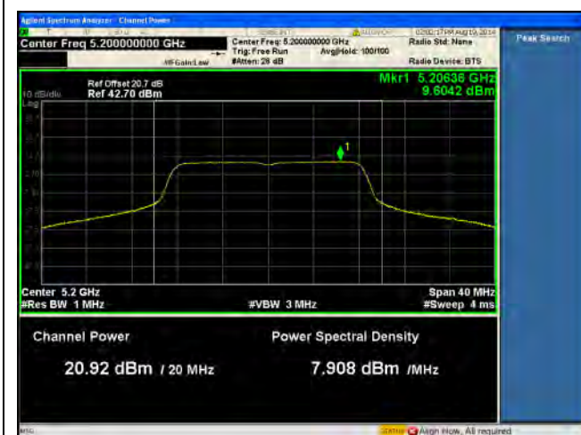
PSD-5.1G-802.11a Mid-chain1
