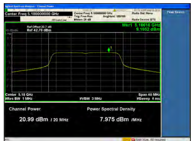
PSD-5.1G-802.11n-20M Low-chain2
