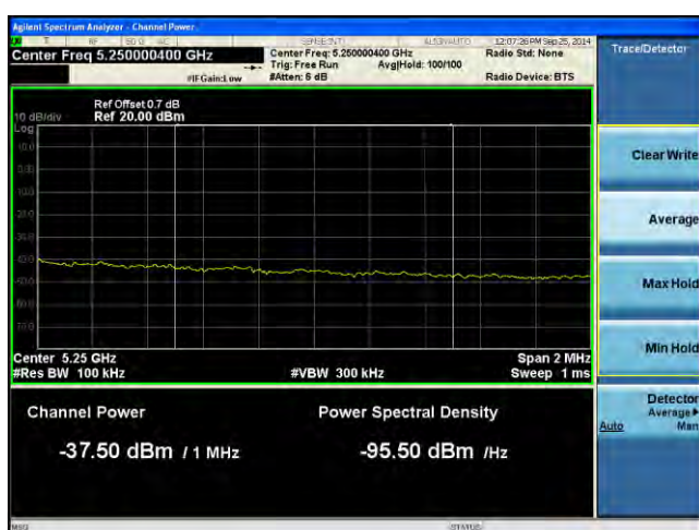
Band Edge-5.1G-802.11n-40M High-Chain1
