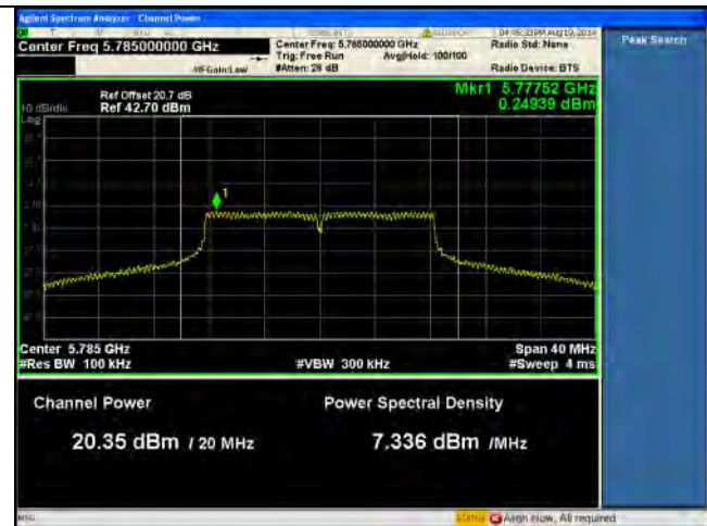
PSD-5.8G-802.11a Mid-chain0
