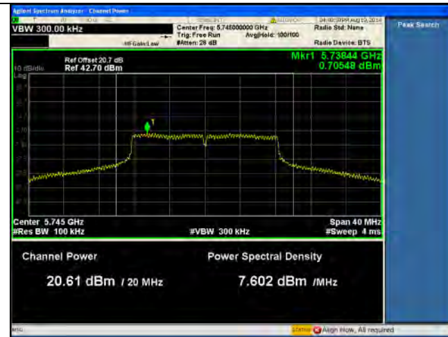
PSD-5.8G-802.11a Low-chain0
