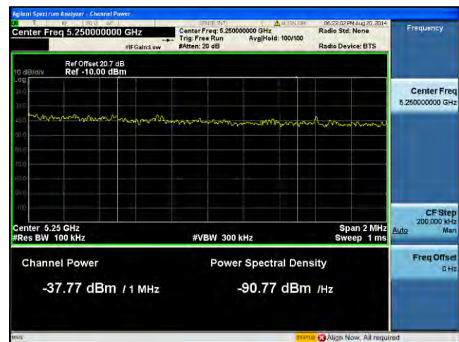
Band Edge-5.1G-802.11ac-80M High-Chain0
