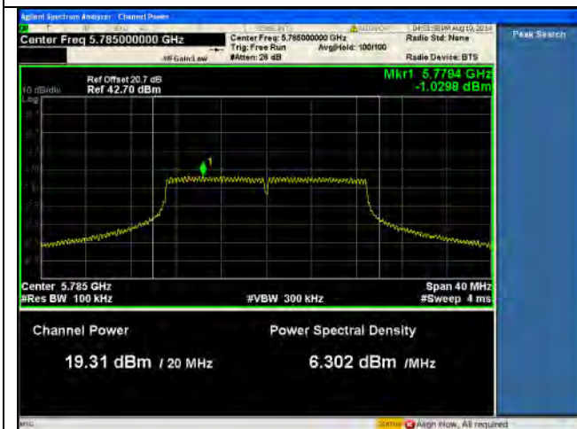
PSD-5.8G-802.11n-20M Mid-chain2
