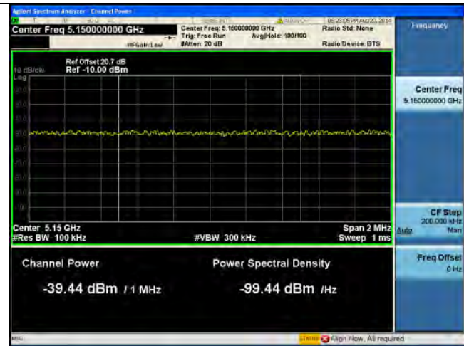
Band Edge-5.1G-802.11ac-80M Low-Chain1
