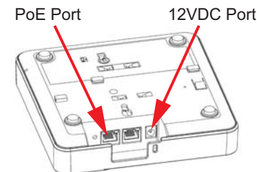
Figure 2: Bottom view
