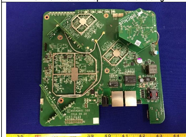
EUT Main Board - Top View without shielding
