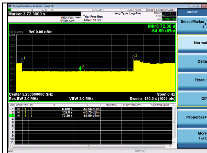
Initial CAC – VHT160 – 5250MHz
