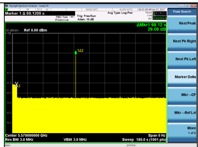
Radar at beginning of CAC – VHT160 – 5570MHz
