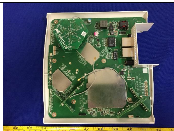
EUT Main Board - Top View
