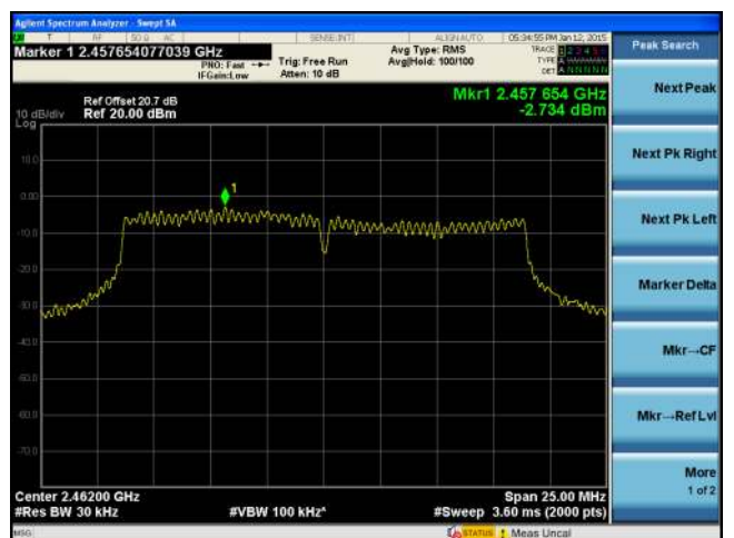
PSD-2.4G-802.11n-20M High-chain4
