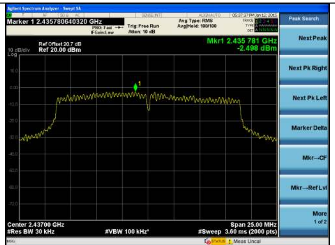
PSD-2.4G-802.11n-20M Mid-chain4
