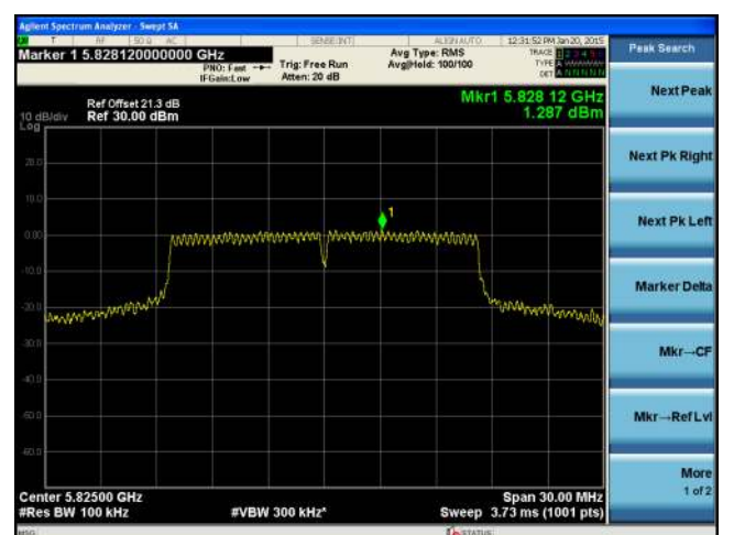
PSD-802.11a-5825M-chain4
