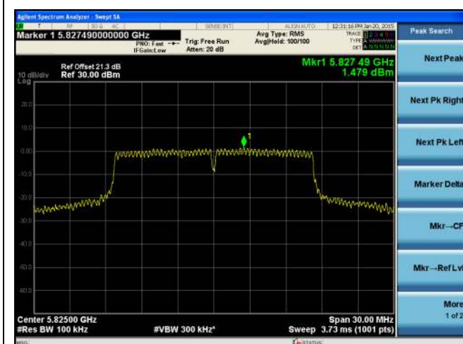
PSD-802.11a-5825M-chain3
