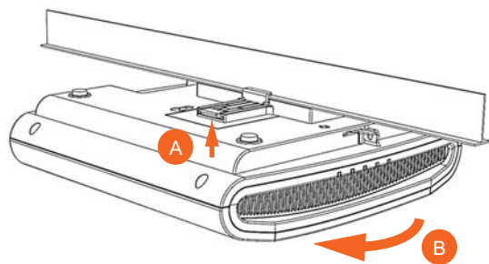
Figure 5. Removing the AP and T-bar bracket from the T-bar
