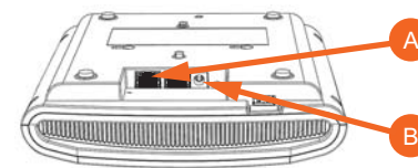
Figure 2. AP ports
