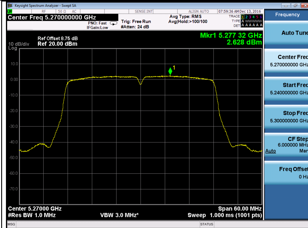
802.11n-HT40 5270M
