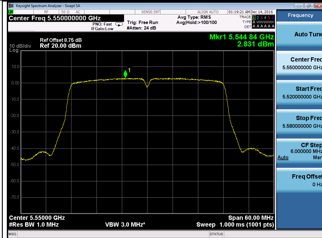
802.11n-HT40 5550M
