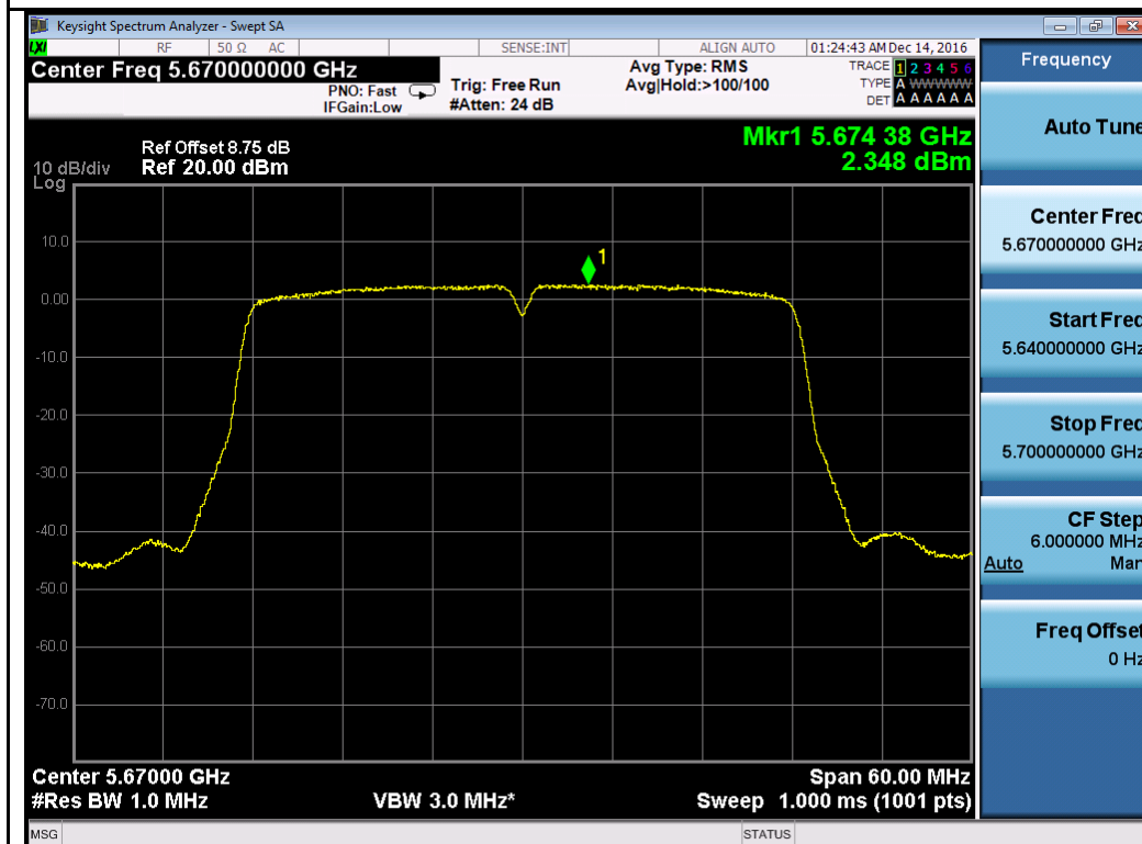
802.11n-HT40 5670M
