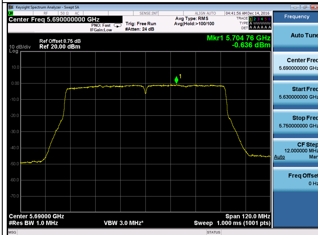
802.11ac-VHT80 5690M
