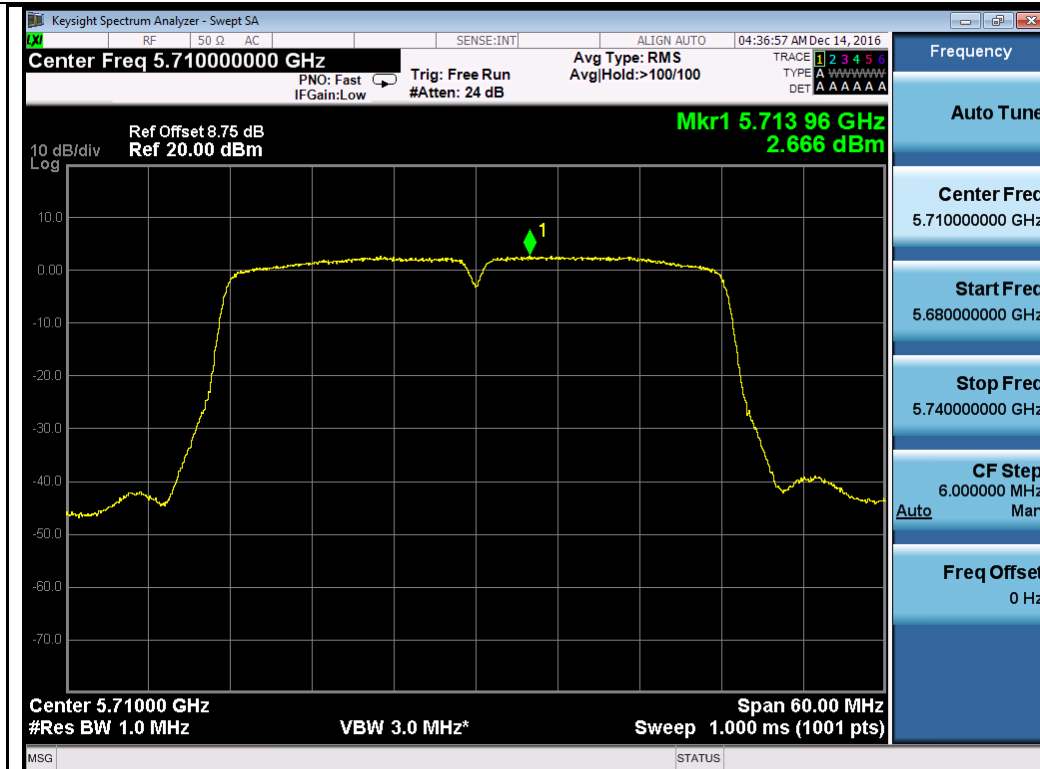
802.11n-HT40 5710M
