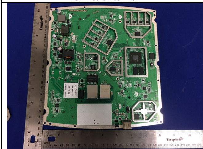
Main Board Shielding off Rear View
