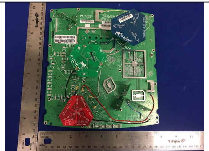
Main Board Shielding off Front View
