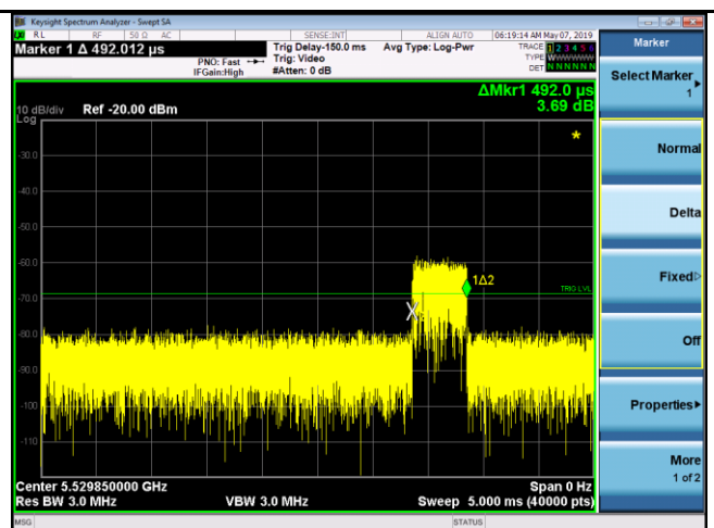
Pulse width after 200ms - 802.11ax-5530MHz (Type0)
