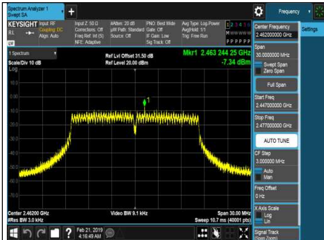
802.11g-2462MHz Chain 0
