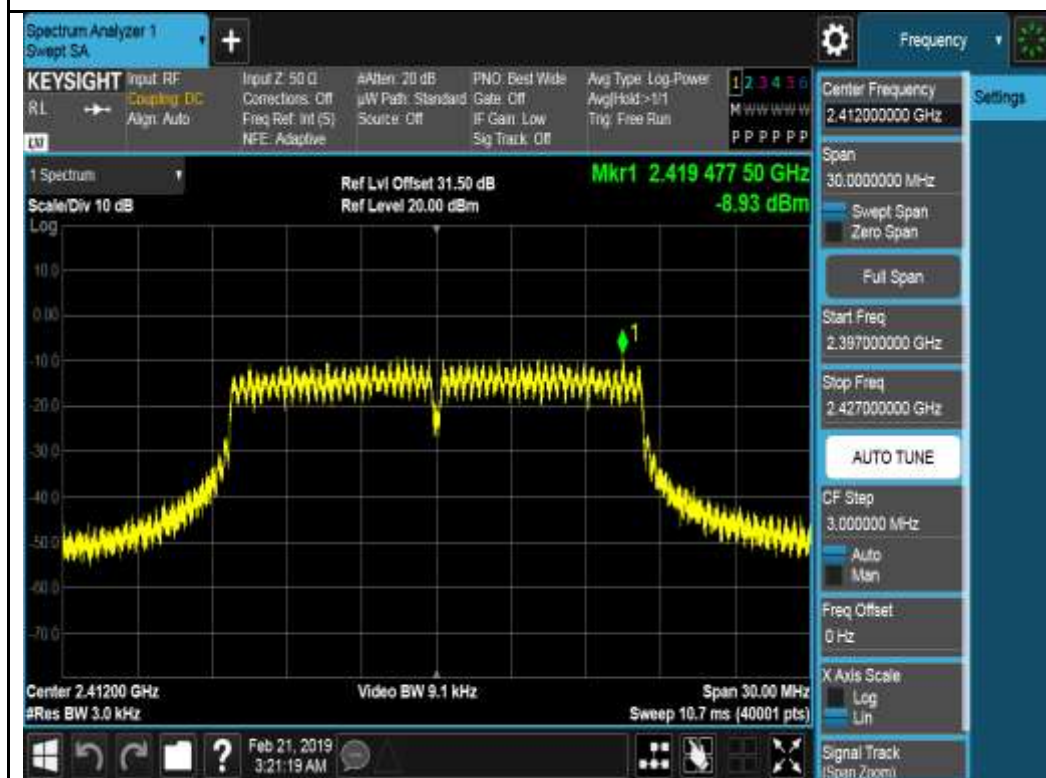
802.11g-2412MHz Chain 3
