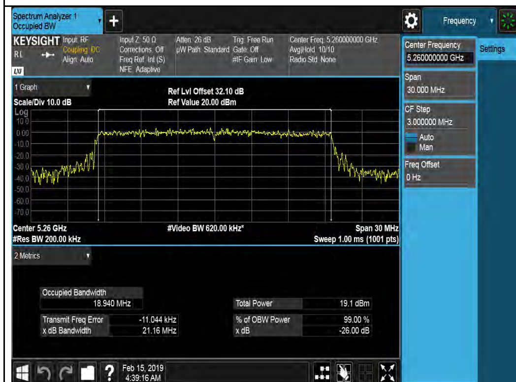
802.11ax-HT20-5260MHz
