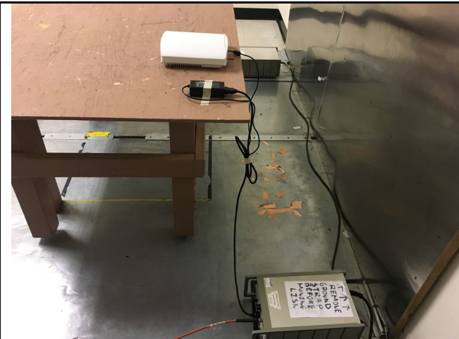
Conducted Emission – Side View
