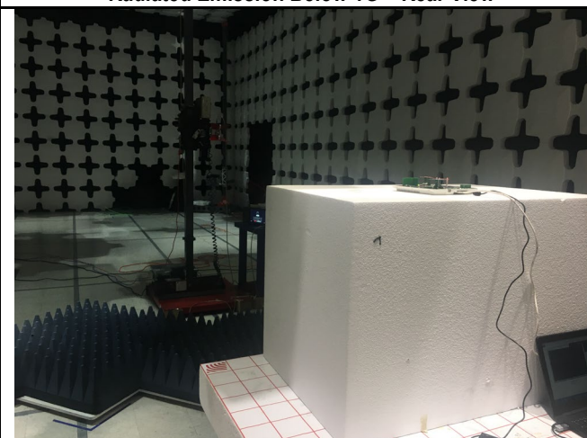
Radiated Emission Above 1G – Rear View
