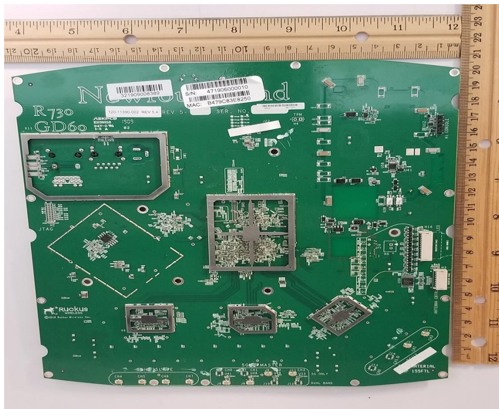
Picture 6: Back Side with Shields removed– AP board
