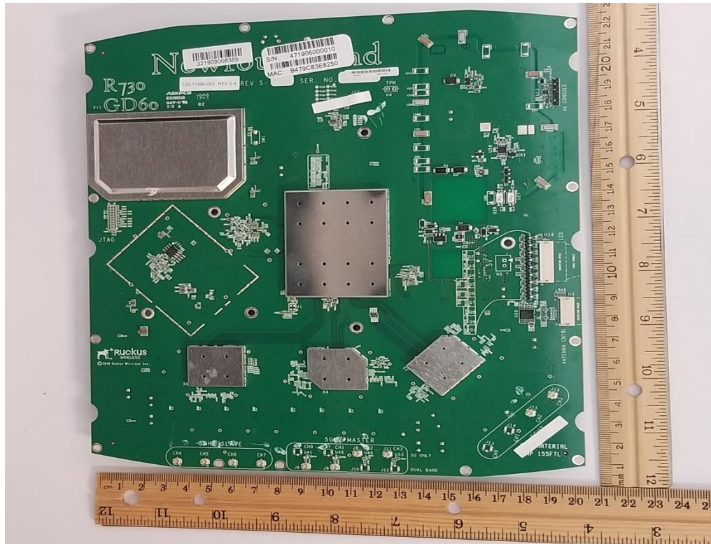
Picture 5: Back Side with Shields – AP board
