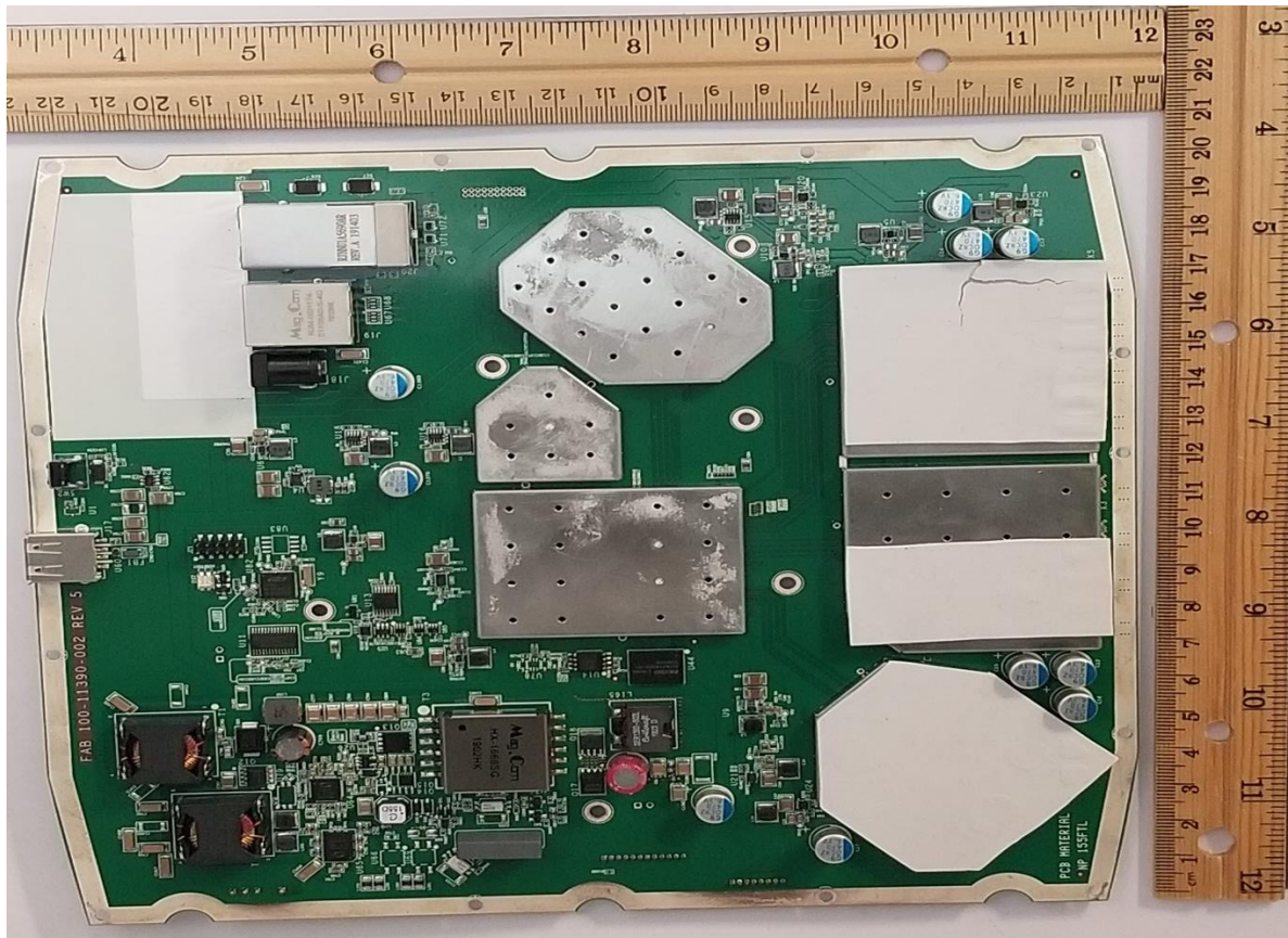
Picture 3: Top side with Shields – AP Board
