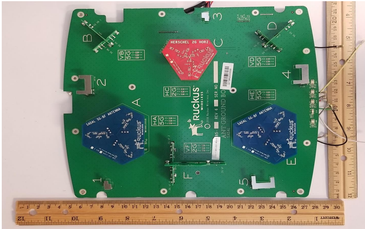
Picture 1: Front Antennas View
