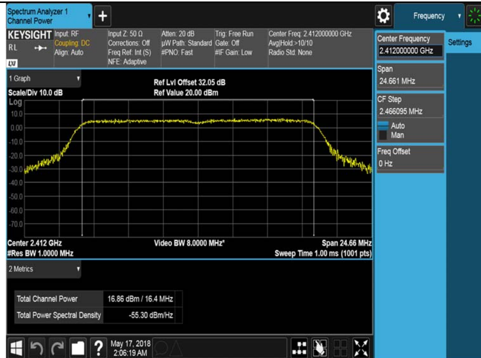
802.11g-2412MHz Chain 3
