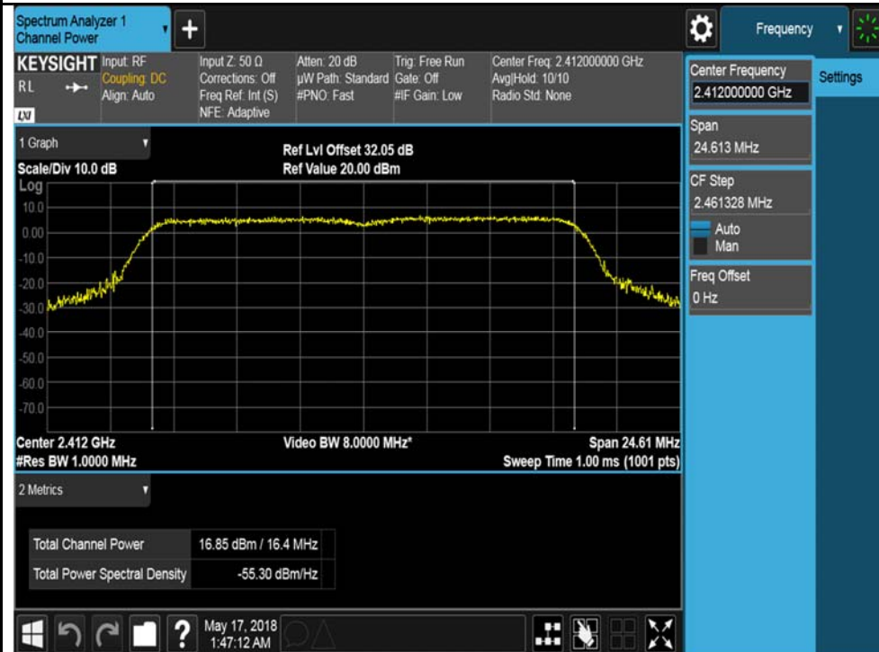
802.11g-2412MHz Chain 1
