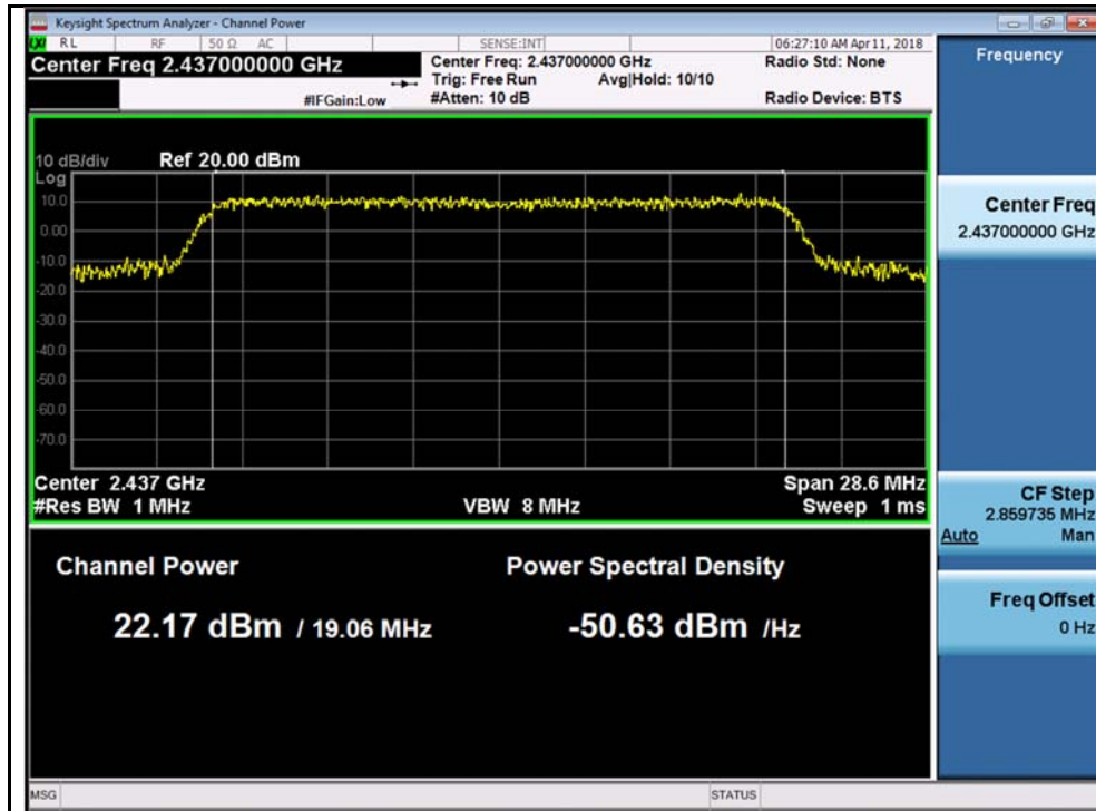
802.11ax20 2437MHz Chain 0
