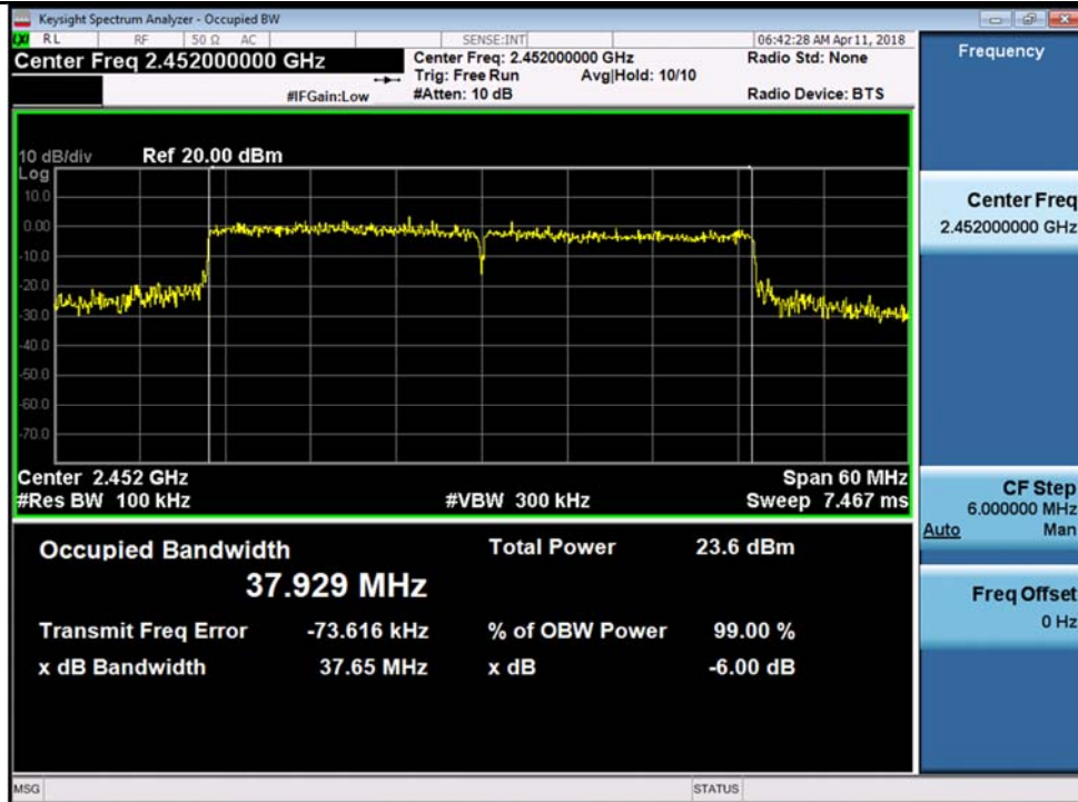
802.11ax40-2452MHz
