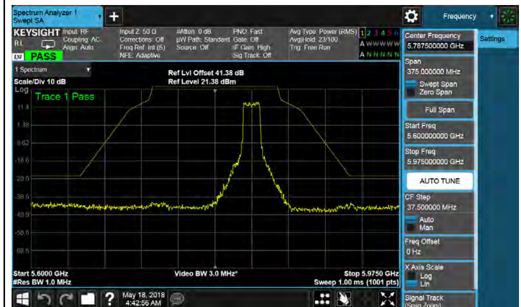
802.11a-5825M
