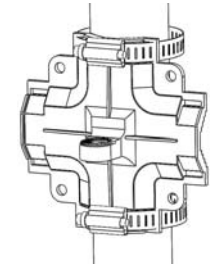
Figure 4: Hanger mount on a vertical pole
