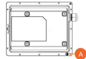
Figure 9: Connect good earth ground to AP here
