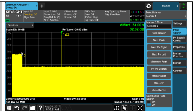
Radar at beginning of CAC – VHT80 – 5530MHz
