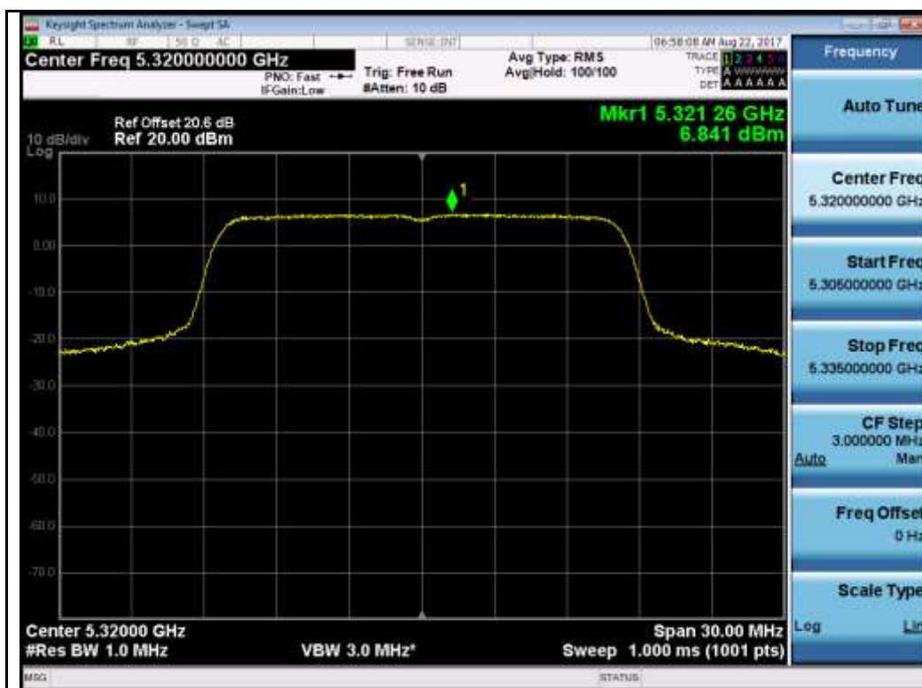
802.11a-5320M
