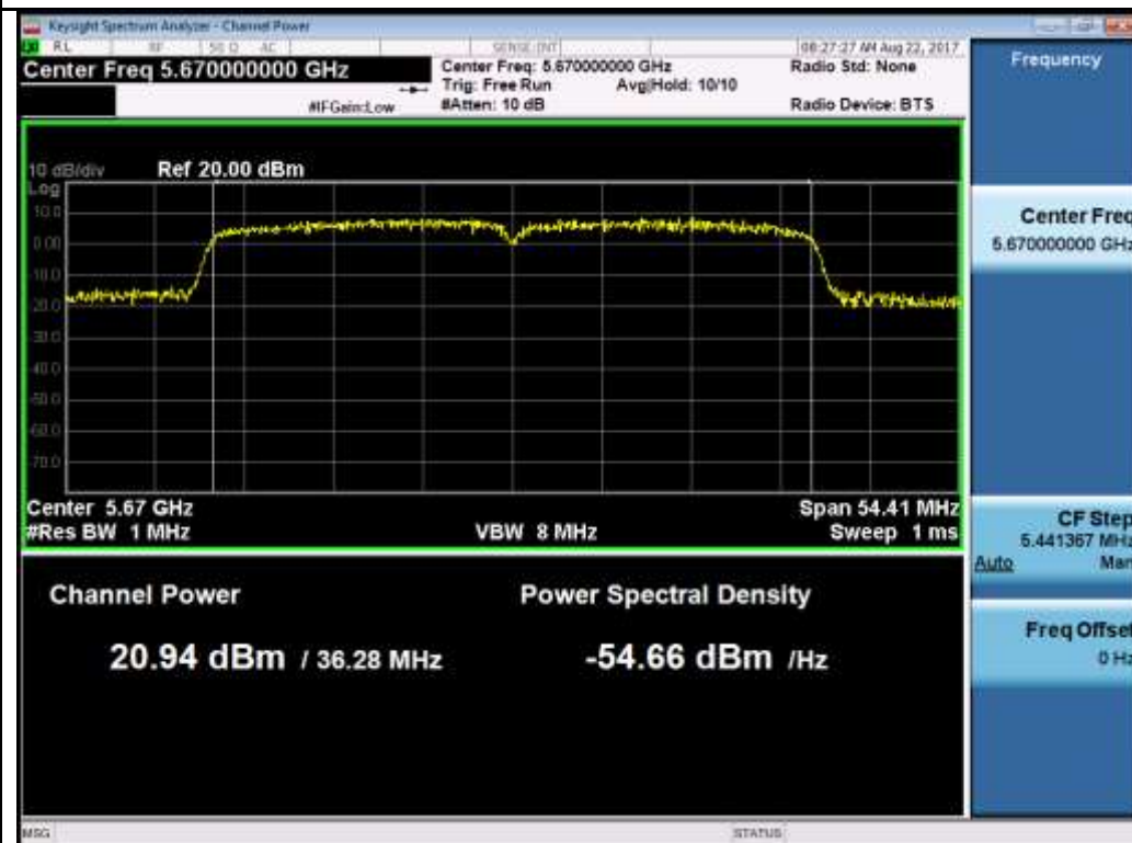
802.11n-HT40 5670M
