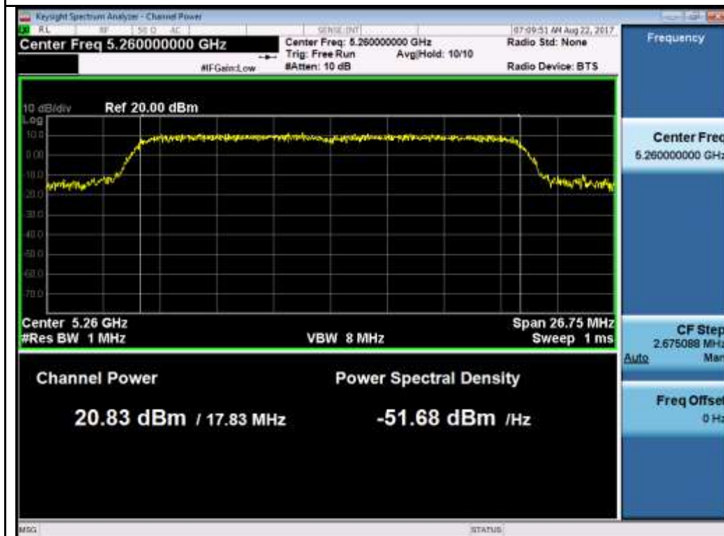
802.11n-HT20 5260M
