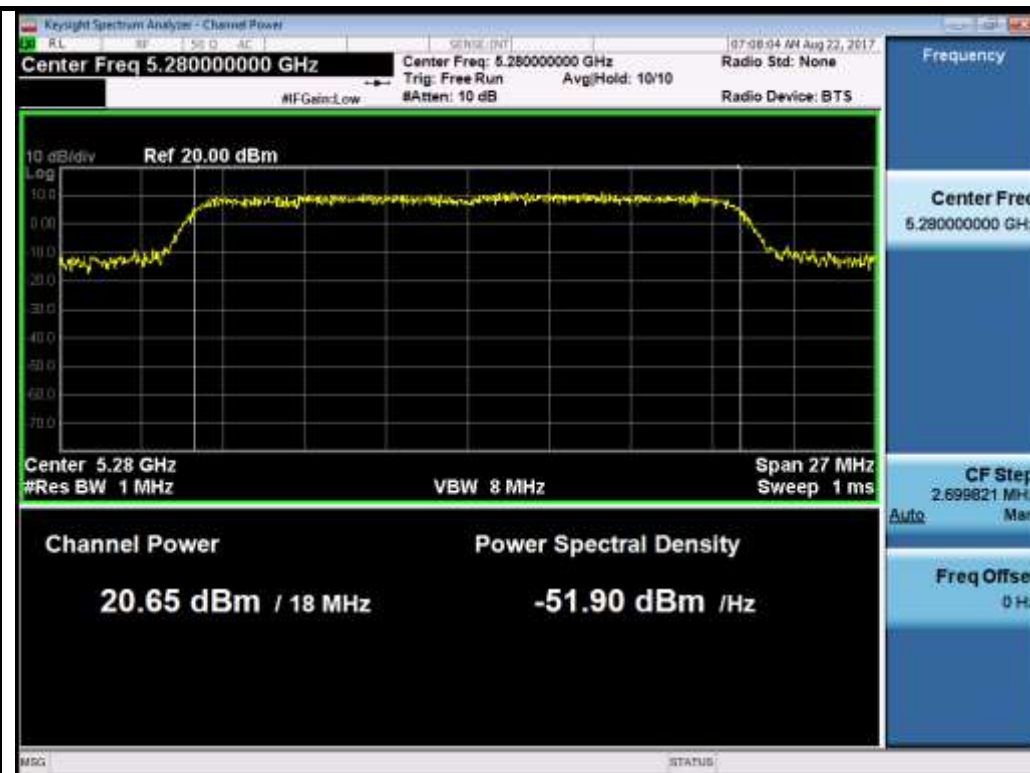
802.11n-HT20 5280M
