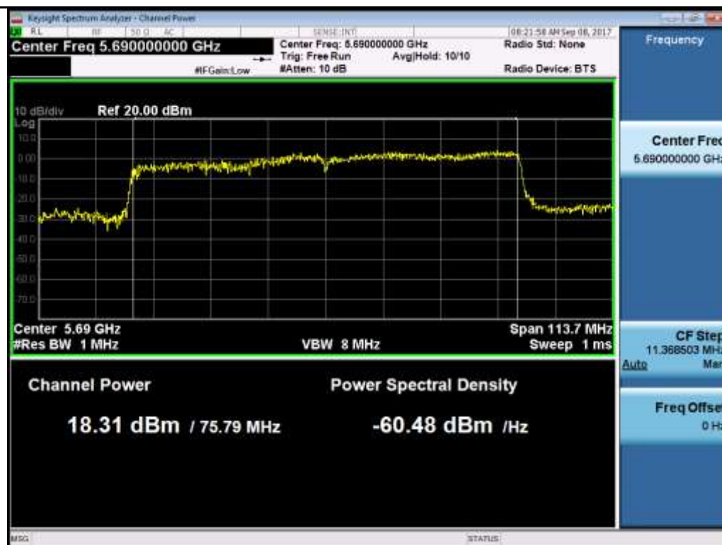
802.11ac-VHT80 5690M
