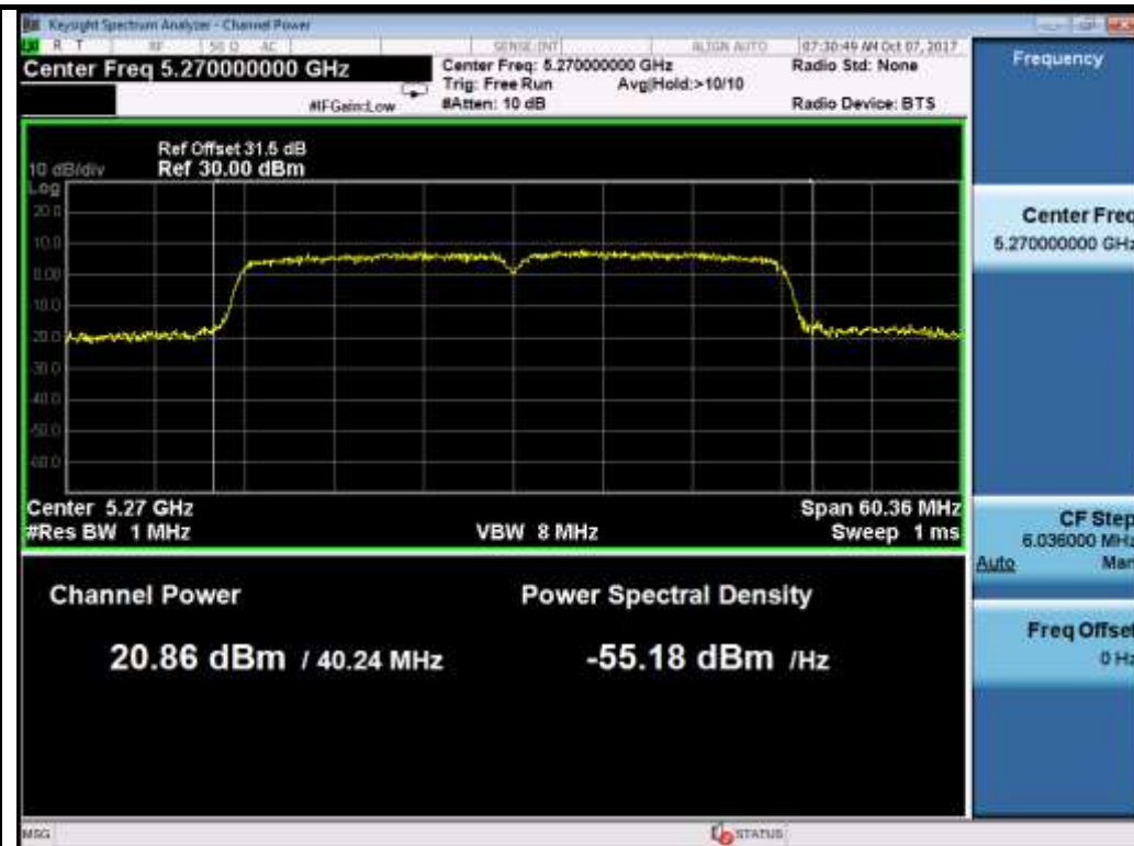
802.11n-HT40 5270M
