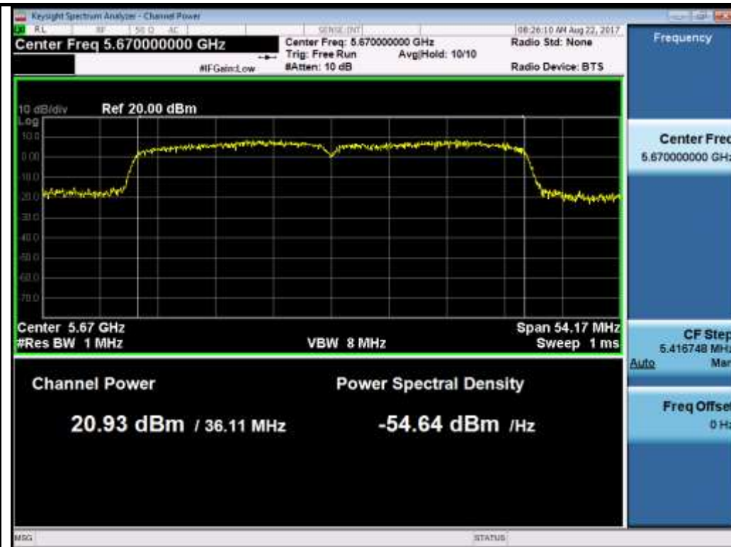
802.11n-HT40 5670M
