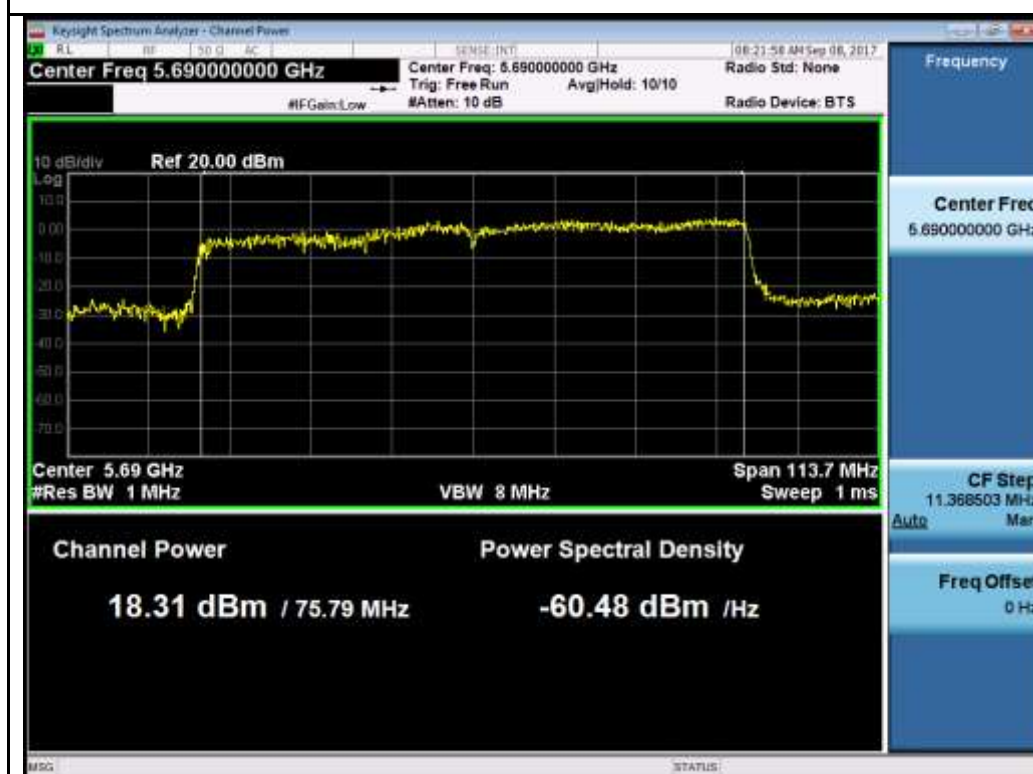
802.11ac-VHT80 5690M
