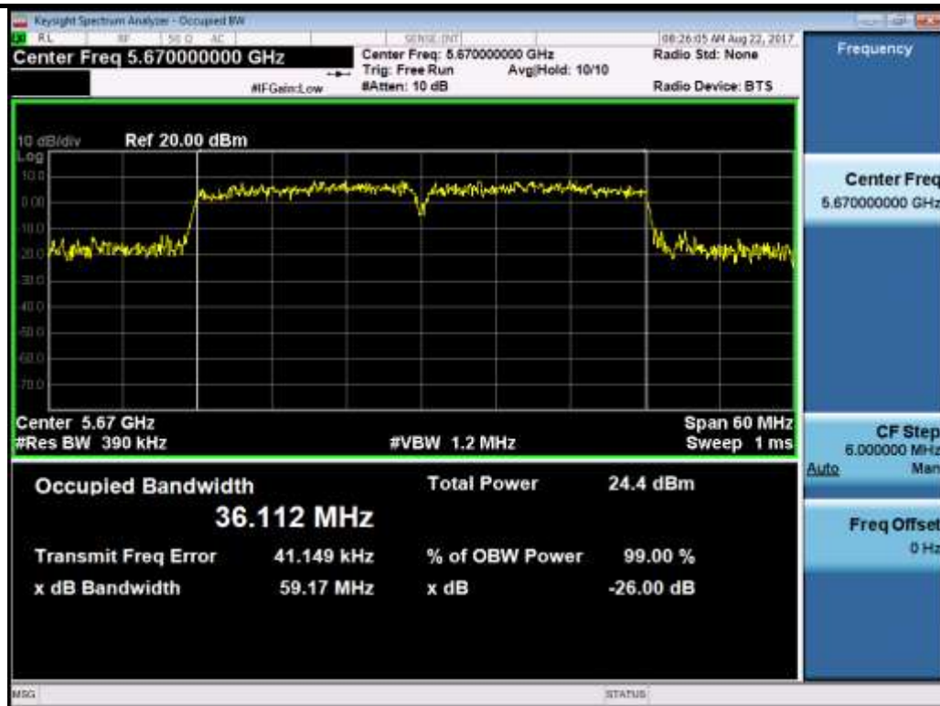
802.11n-HT40-5670MHz
