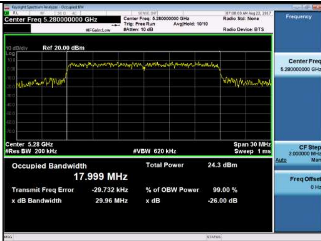
802.11n-HT20-5280MHz
