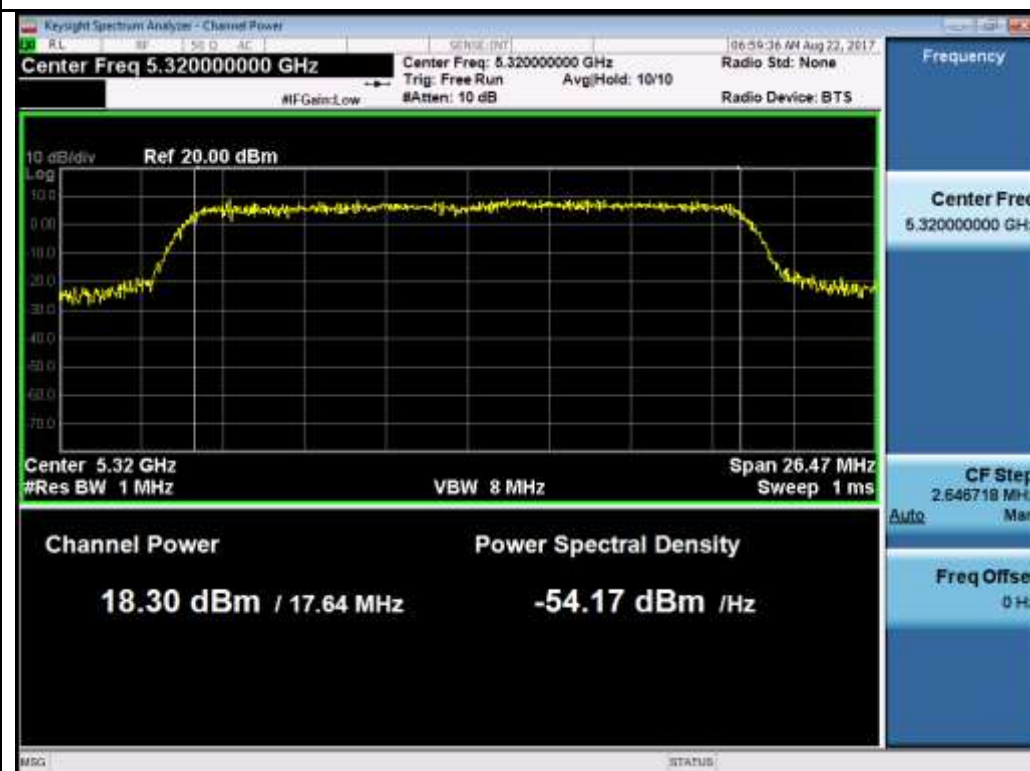
802.11n-HT20 5320M
