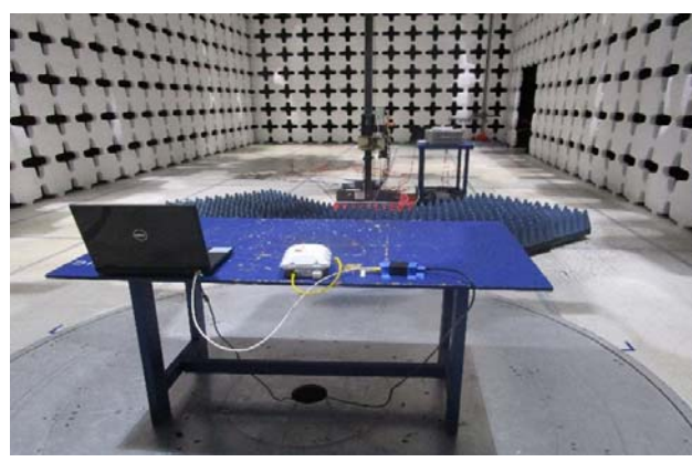
Radiated Emissions (>1GHz) – Rear View
