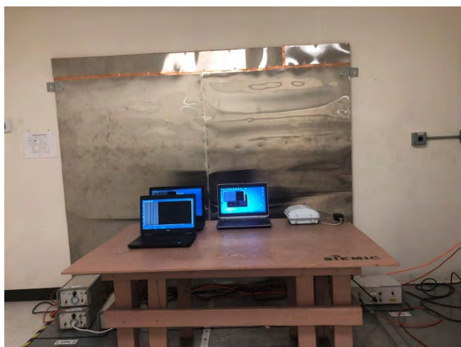
Conducted Emissions - P.O.E Mode – Front View
