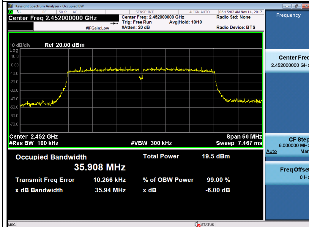
802.11n-HT40-2452MHz
