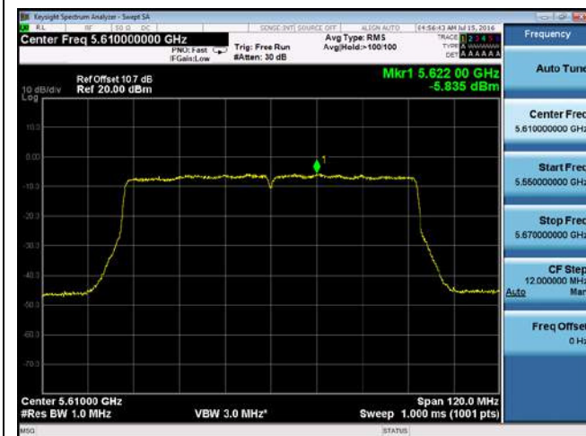
PSD-802.11ac-80M-5610M-chain1
