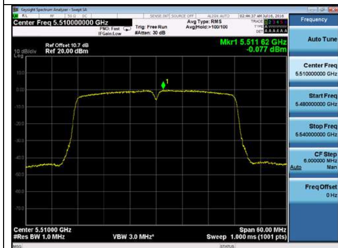
PSD-802.11n-40M-5510M-chain3
