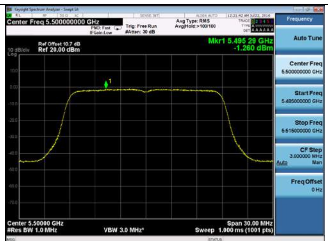
PSD-802.11n-20M-5500M-chain4
