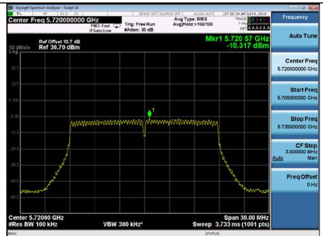
PSD-802.11n-20M-CROSS-5720M-chain2
