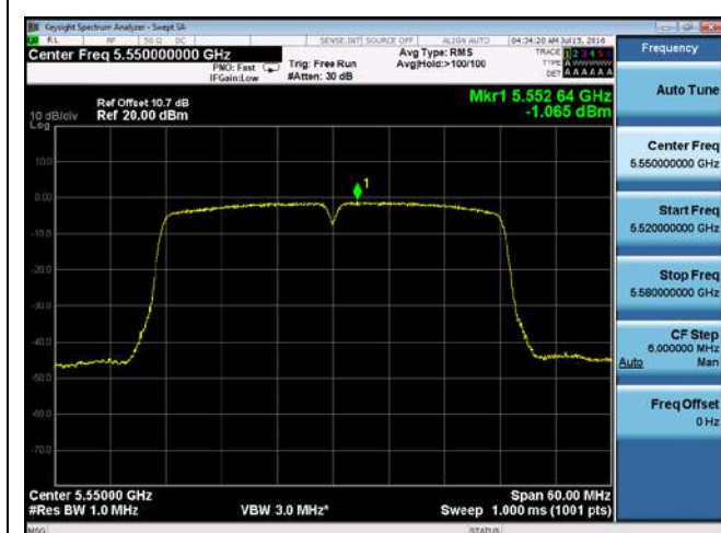
PSD-802.11n-40M-5550M-chain1
