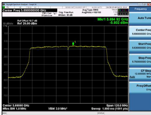
PSD-802.11ac-CROSS-5690M-chain1
