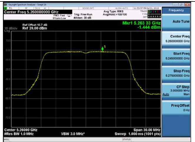
PSD-802.11a-5260M-chain2
