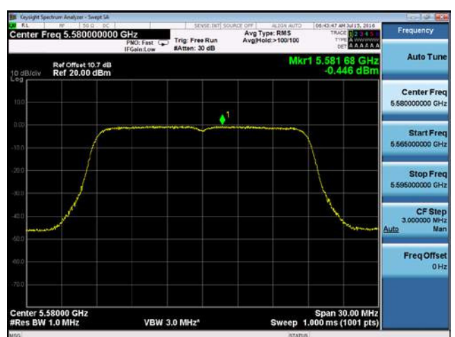
PSD-802.11n-20M-5580M-chain2
