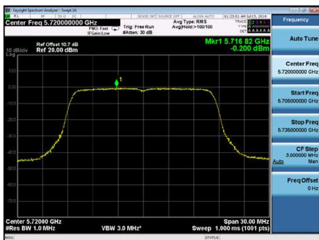
PSD-802.11a-CROSS-5720M-chain1
