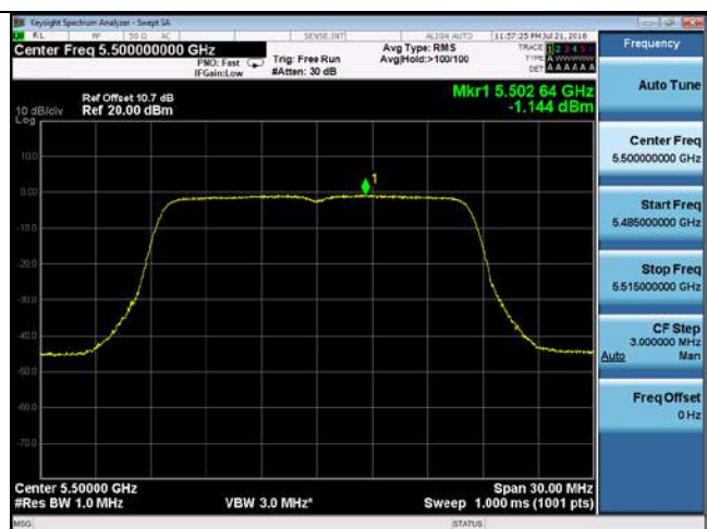
PSD-802.11a-5500M-chain2
