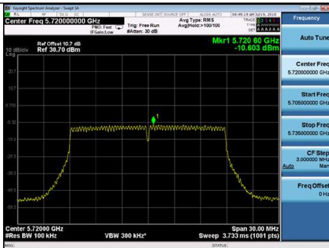
PSD-802.11n-20M-CROSS-5720M-chain1
