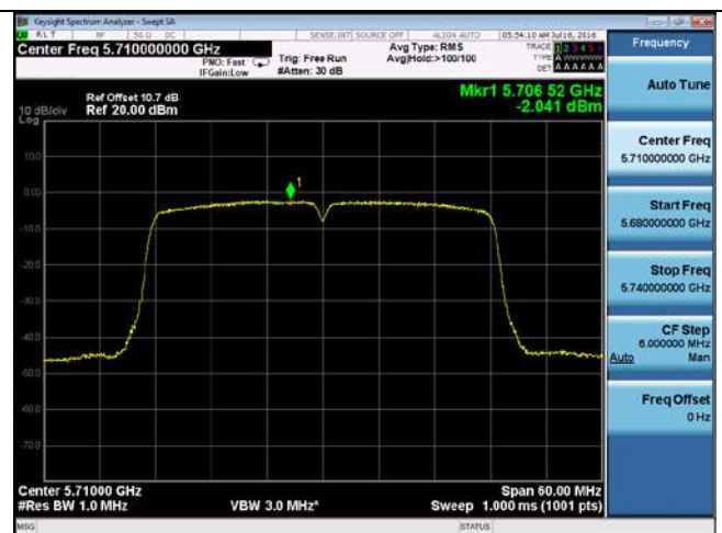
PSD-802.11n-40M-CROSS-5710M-chain4
