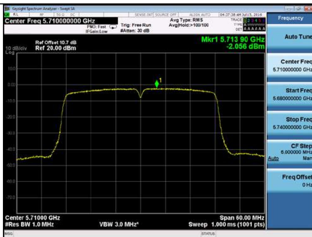
PSD-802.11n-40M-CROSS-5710M-chain1
