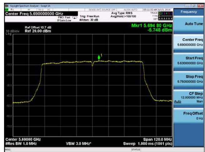
PSD-802.11ac-CROSS-5690M-chain2
