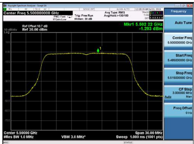
PSD-802.11a-5500M-chain4
