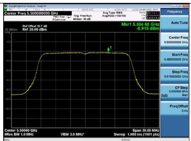
PSD-802.11n-20M-5500M-chain2
