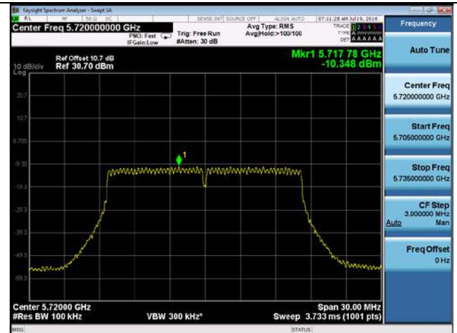
PSD-802.11a-CROSS-5720M-chain4
