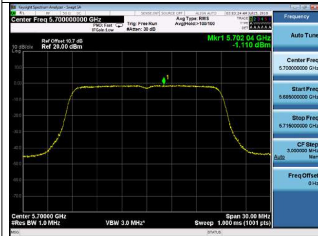
PSD-802.11n-20M-5700M-chain1
