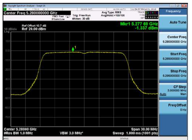
PSD-802.11a-5280M-chain2
