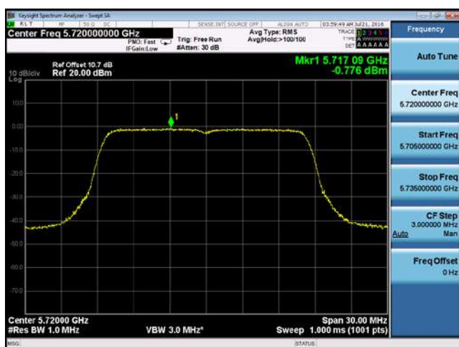
PSD-802.11a-CROSS-5720M-chain3
