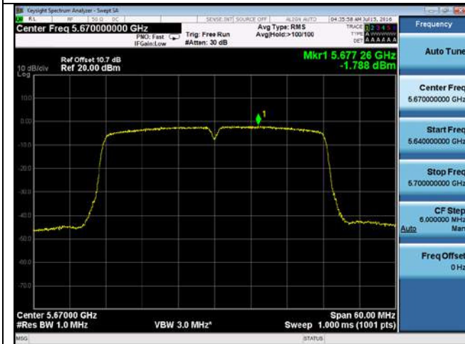
PSD-802.11n-40M-5670M-chain1
