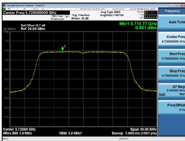
PSD-802.11n-20M-CROSS-5720M-chain3
