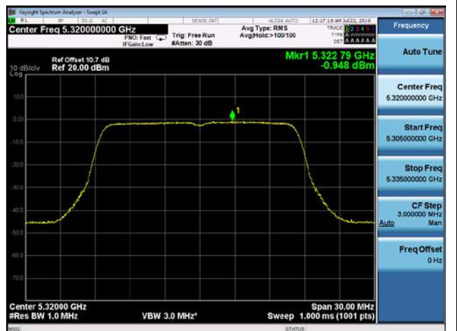
PSD-802.11a-5320M-chain4
