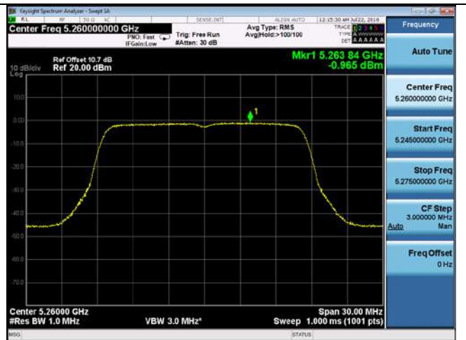
PSD-802.11a-5260M-chain4
