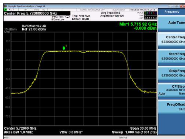
PSD-802.11a-CROSS-5720M-chain4
