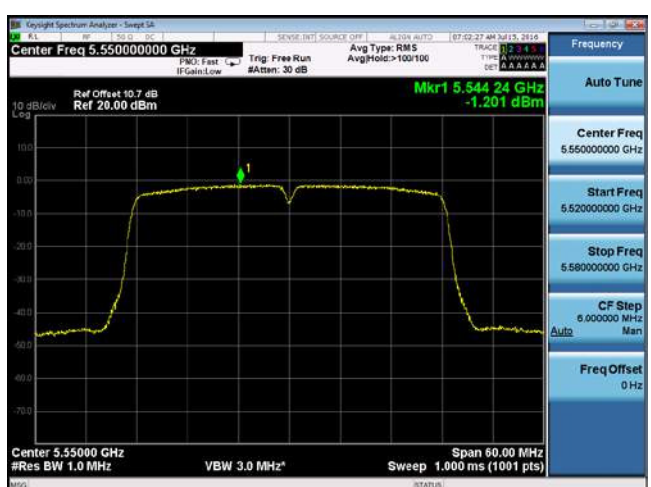
PSD-802.11n-40M-5550M-chain2
