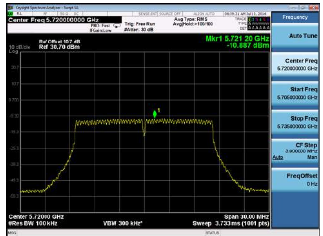
PSD-802.11a-CROSS-5720M-chain2
