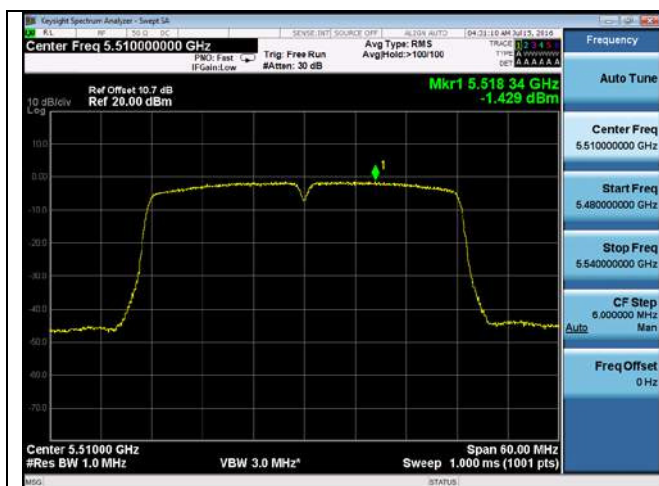
PSD-802.11n-40M-5510M-chain1
