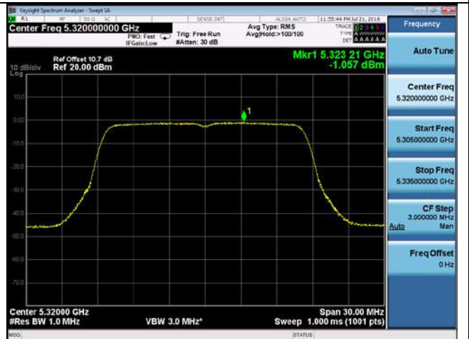
PSD-802.11a-5320M-chain2
