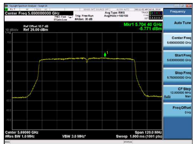
PSD-802.11ac-CROSS-5690M-chain4
