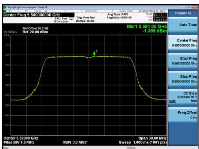
PSD-802.11a-5580M-chain2
