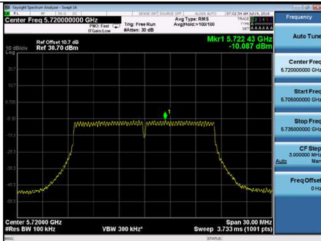
PSD-802.11a-CROSS-5720M-chain3
