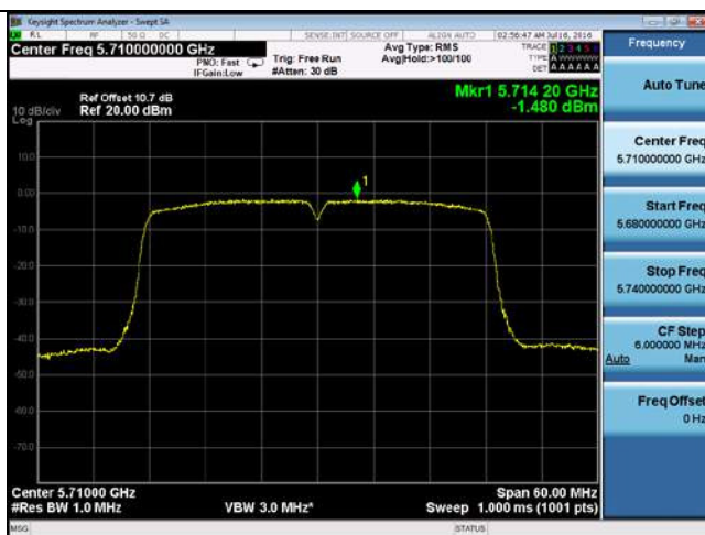
PSD-802.11n-40M-CROSS-5710M-chain3
