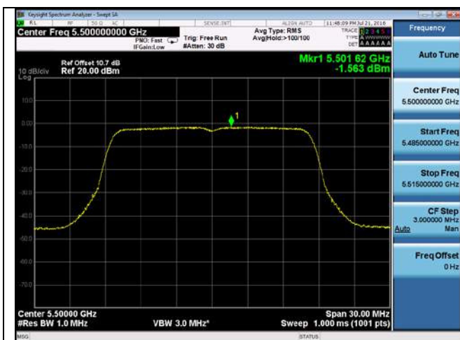
PSD-802.11a-5500M-chain1
