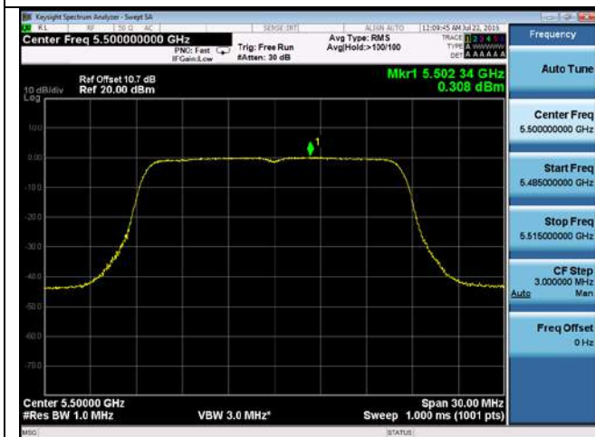
PSD-802.11a-5500M-chain3
