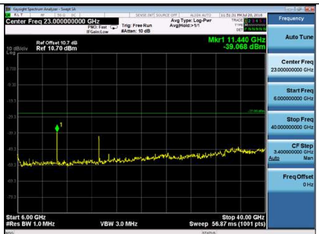
CUE-802.11n20-5720M -chain1(6GHz-40GHz)
