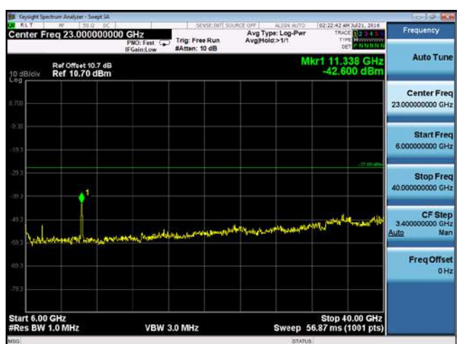
CUE-802.11ac80-5690M -chain4 (6GHz-40GHz)
