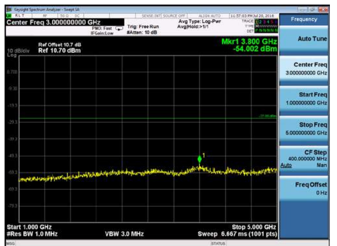
CUE-802.11n-40-5550M-chain1(1GHz-5GHz)
