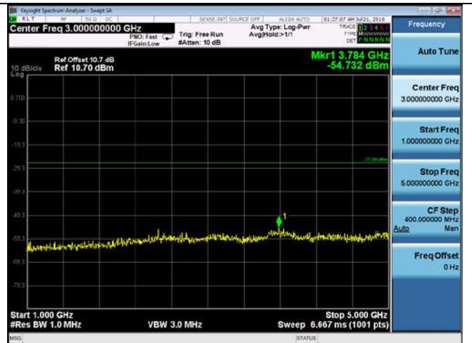
CUE-802.11ac-80-5610M-chain3(1GHz-5GHz)
