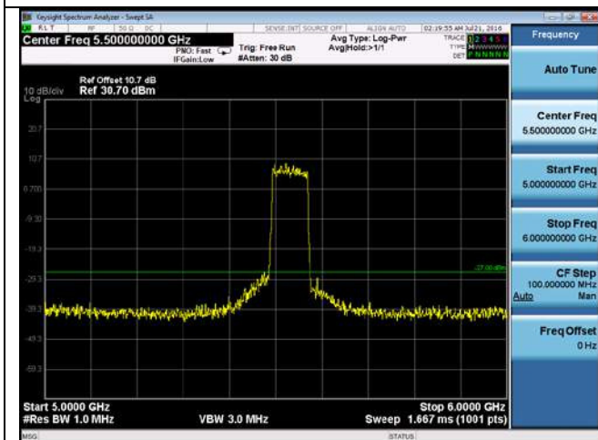
CUE-802.11ac-80-5530M-chain4(5GHz-6GHz)
