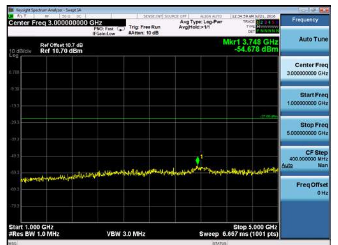
CUE-802.11n-40-5510M-chain2(1GHz-5GHz)
