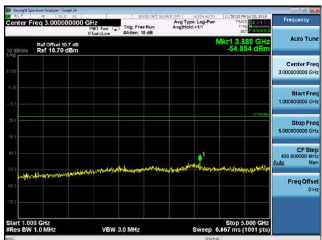
CUE-802.11n40-5710M -chain1(1GHz-5GHz)
