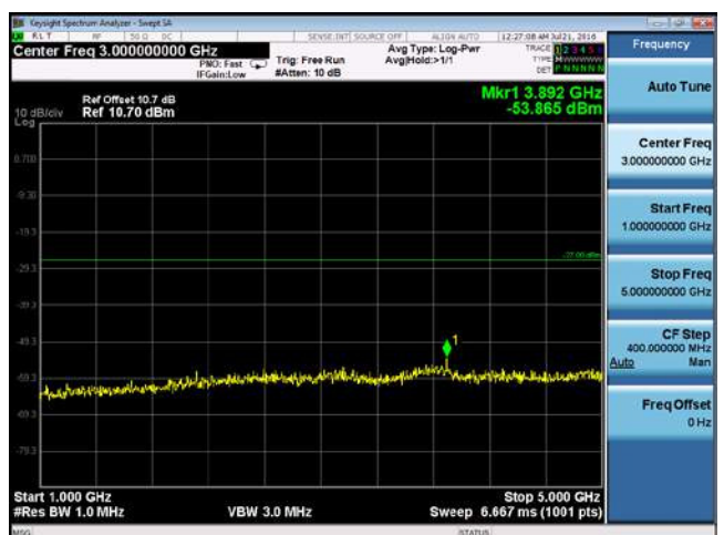
CUE-802.11n20-5720M -chain2(1GHz-5GHz)
