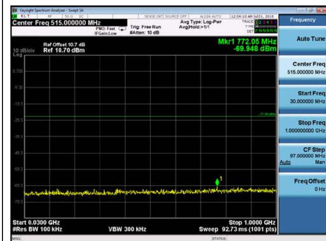
CUE-802.11ac-80-5610M-chain1(30MHz-1GHz)
