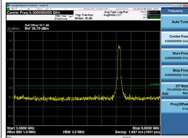
CUE-802.11a-5720M -chain4 (5GHz-6GHz)
