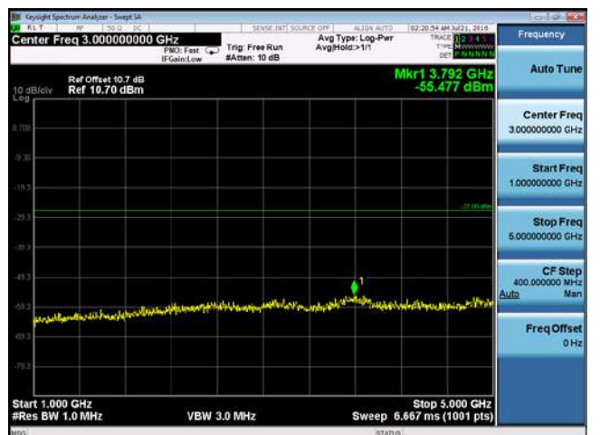
CUE-802.11ac-80-5610M-chain4(1GHz-5GHz)
