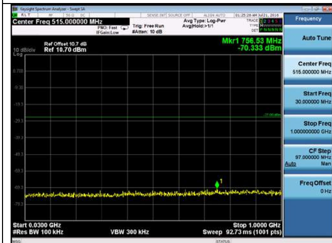
CUE-802.11n-40-5510M-chain3(30MHz-1GHz)
