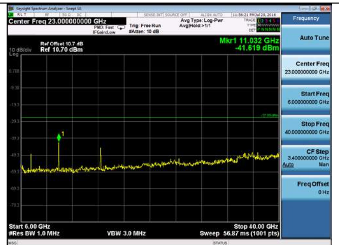
CUE-802.11n-40-5510M-chain1(6GHz-40GHz)
