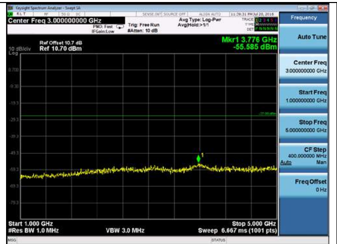
CUE-802.11a-5720M -chain1(1GHz-5GHz)
