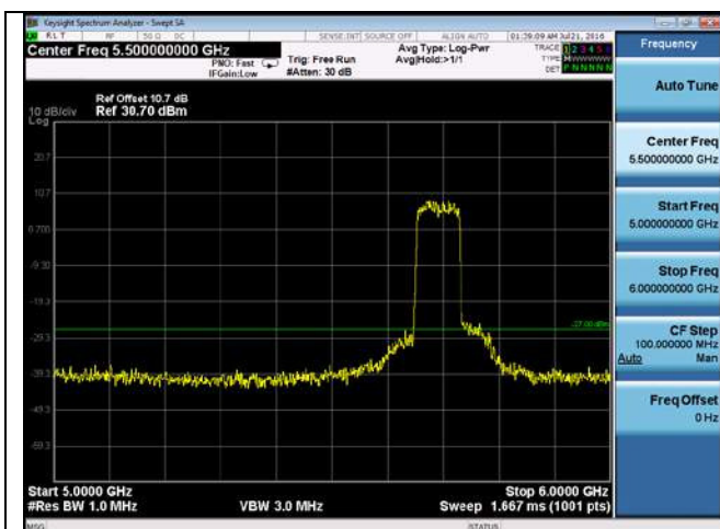
CUE-802.11ac80-5690M -chain3 (5GHz-6GHz)
