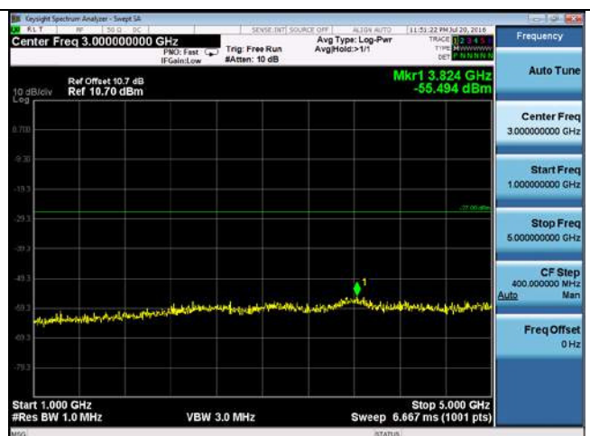
CUE-802.11n20-5720M -chain1(1GHz-5GHz)
