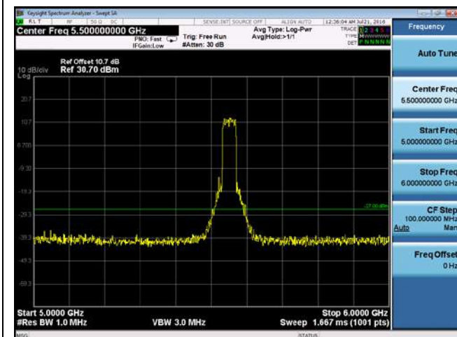
CUE-802.11n-40-5550M-chain2(5GHz-6GHz)
