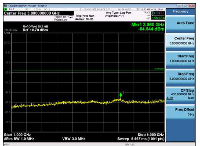
CUE-802.11n-40-5550M-chain4(1GHz-5GHz)
