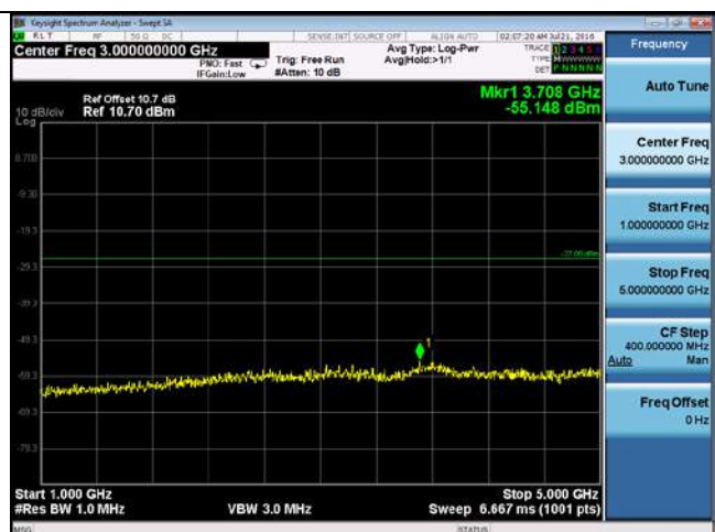
CUE-802.11n20-5720M -chain4(1GHz-5GHz)
