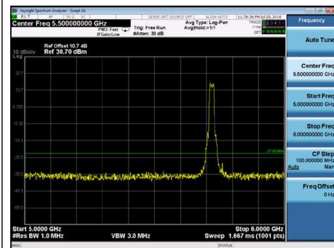
CUE-802.11a-5720M -chain1(5GHz-6GHz)
