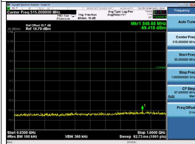
CUE-802.11a-5720M -chain4 (30MHz-1GHz)
