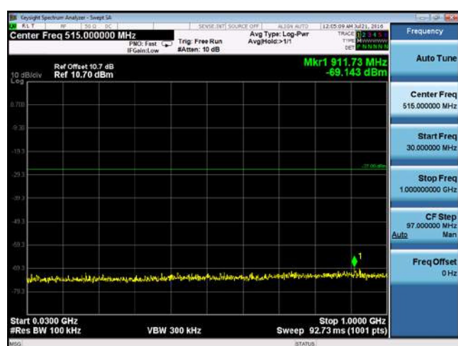
CUE-802.11ac80-5690M -chain1 (30MHz-1GHz)
