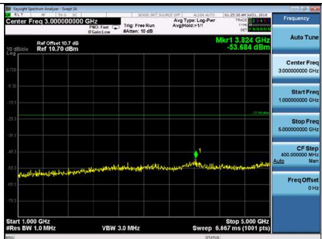
CUE-802.11n-40-5510M-chain3(1GHz-5GHz)
