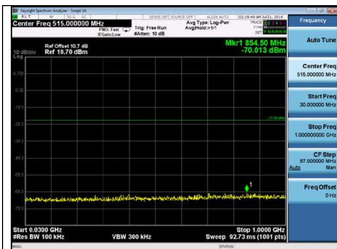
CUE-802.11ac-80-5530M-chain4(30MHz-1GHz)
