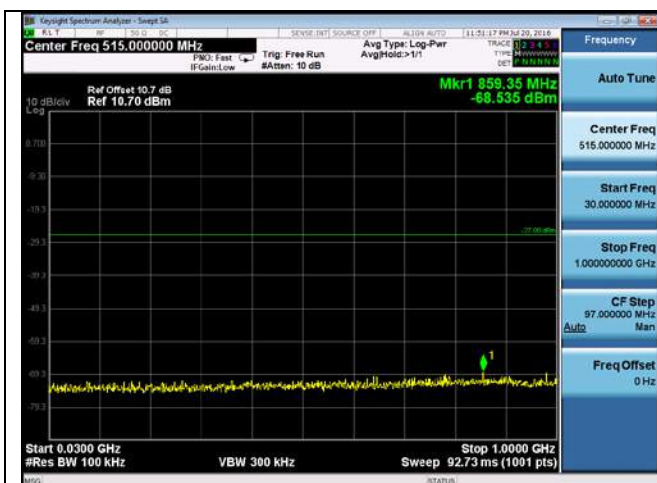
CUE-802.11n20-5720M -chain1(30MHz-1GHz)
