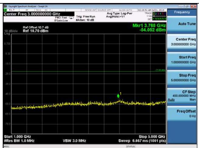
CUE-802.11ac-80-5530M chain4(1GHz-5GHz)
