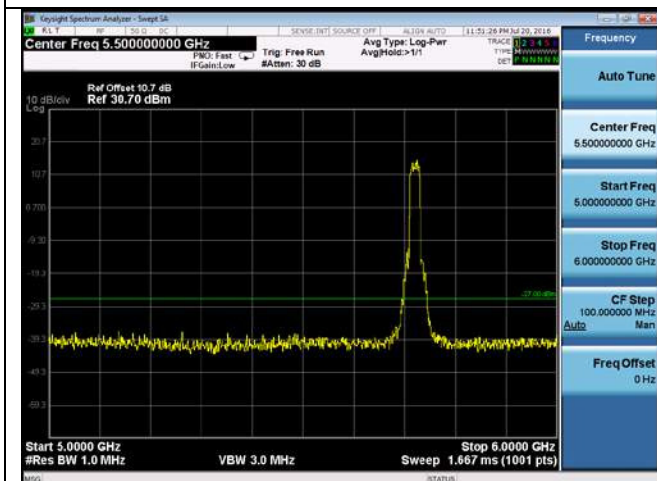
CUE-802.11n20-5720M -chain1(5GHz-6GHz)
