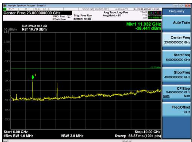
CUE-802.11n-40-5510M-chain3(6GHz-40GHz)
