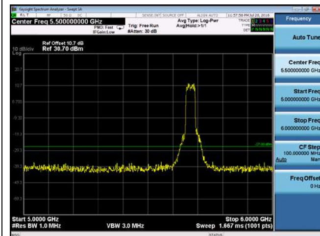
CUE-802.11n-40-5670M-chain 1(5GHz-6GHz)
