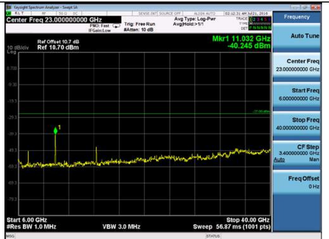
CUE-802.11n-40-5510M-chain4(6GHz-40GHz)
