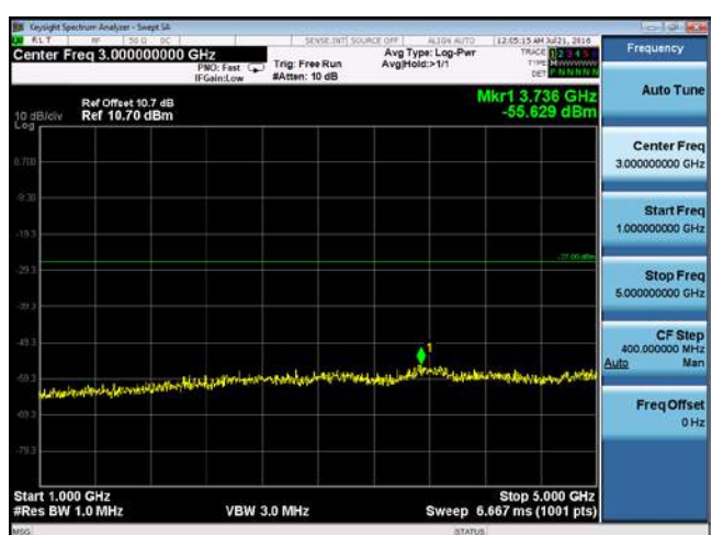
CUE-802.11ac80-5690M -chain1 (1GHz-5GHz)
