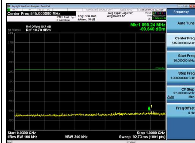
CUE-802.11n40-5710M -chain1(30MHz-1GHz)
