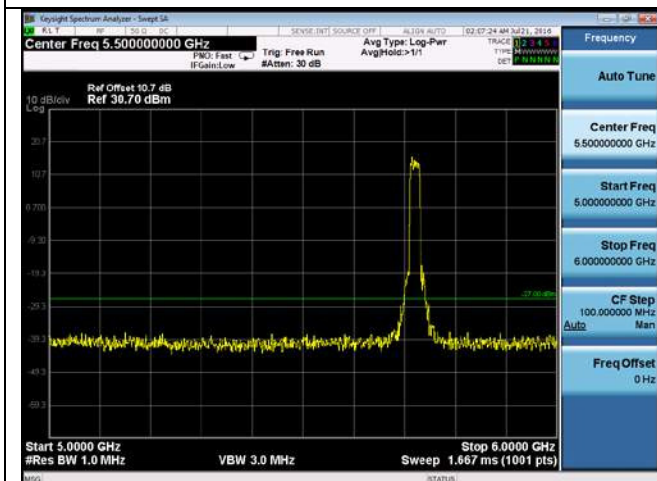
CUE-802.11n20-5720M -chain4(5GHz-6GHz)
