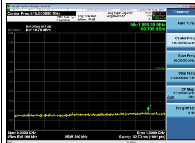
CUE-802.11n20-5720M -chain2(30MHz-1GHz)
