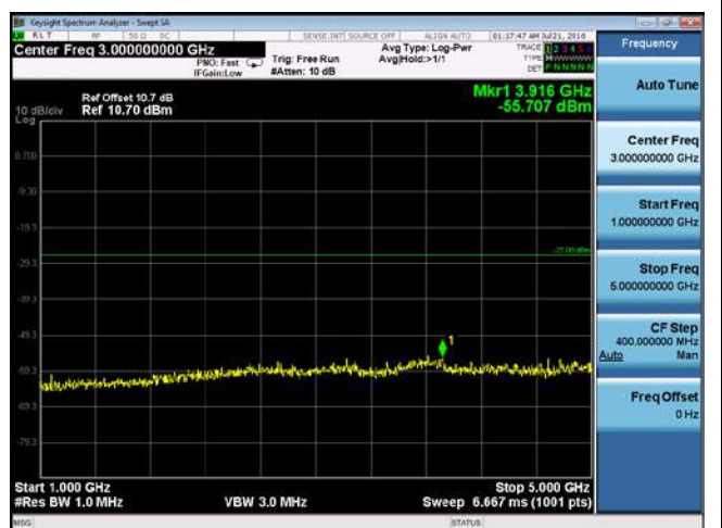
CUE-802.11n20-5720M -chain3(1GHz-5GHz)
