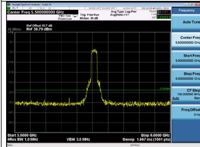
CUE-802.11n-40-5510M-chain4(5GHz-6GHz)
