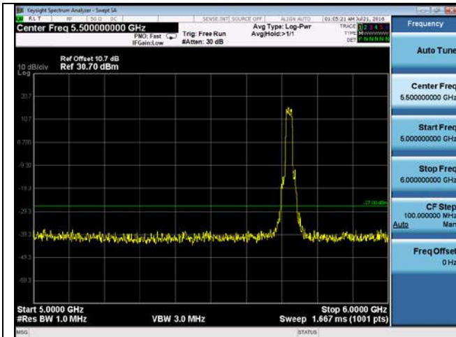
CUE-802.11a-5720M -chain3 (5GHz-6GHz)
