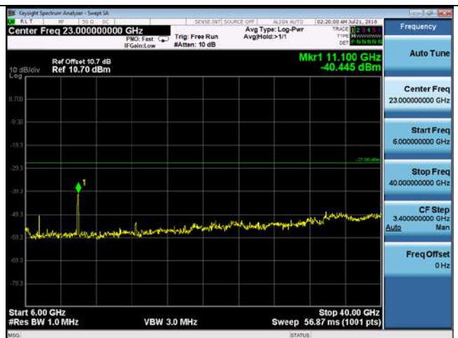
CUE-802.11ac-80-5530M-chain4(6GHz-40GHz)
