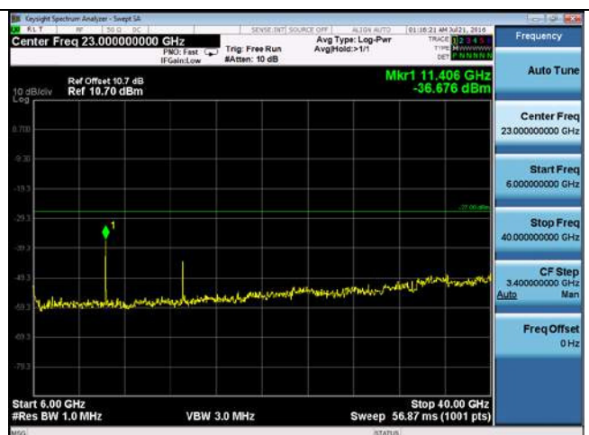
CUE-802.11n-20-5700M -chain 3(6GHz-40GHz)
