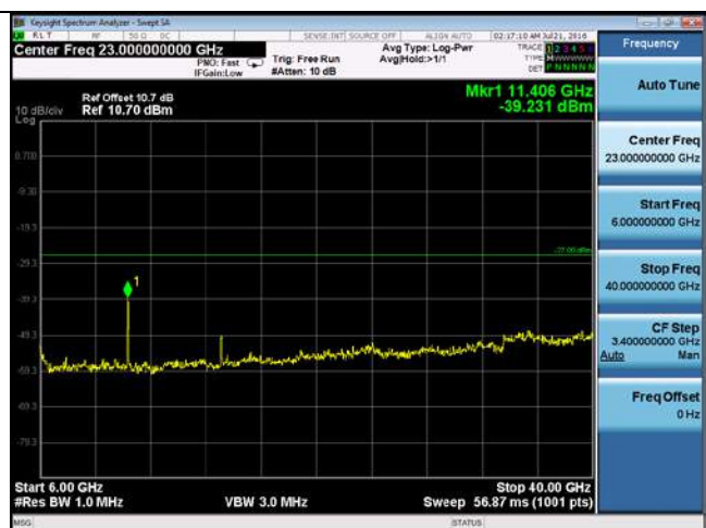
CUE-802.11n40-5710M -chain4 (6GHz-40GHz)
