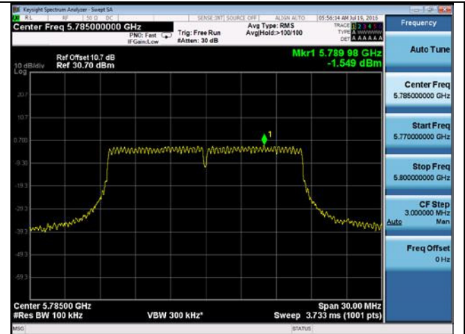
PSD-802.11a-5785M-chain4
