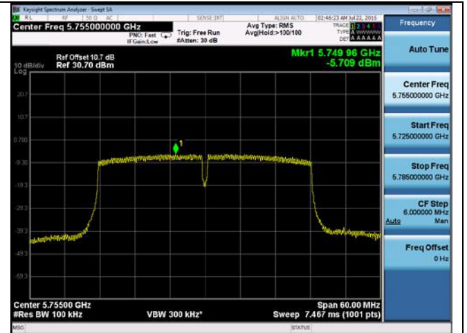
PSD-802.11n-40M-5755M-chain2
