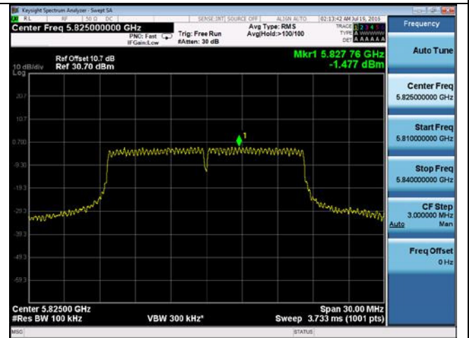
PSD-802.11a-5825M-chain2
