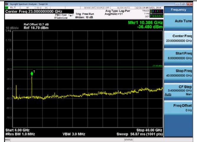
CUE-802.11n-40-5190M chain2(6GHz-40GHz)
