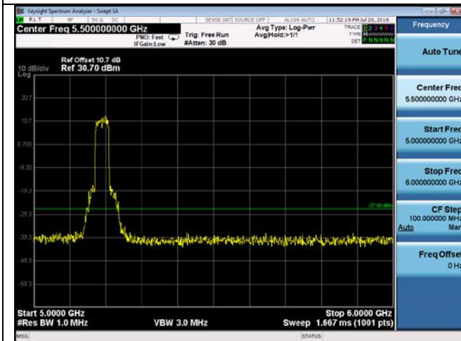
CUE-802.11n-40-5190M-chain1(5GHz-6GHz)
