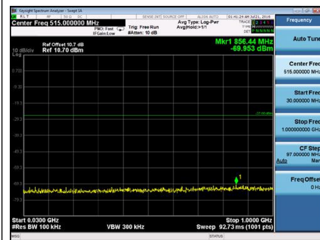
CUE-802.11a-5200M-chain4(30MHz-1GHz)
