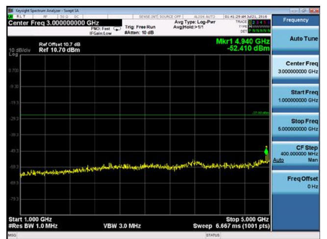
CUE-802.11a-5200M-chain4(1GHz-5GHz)
