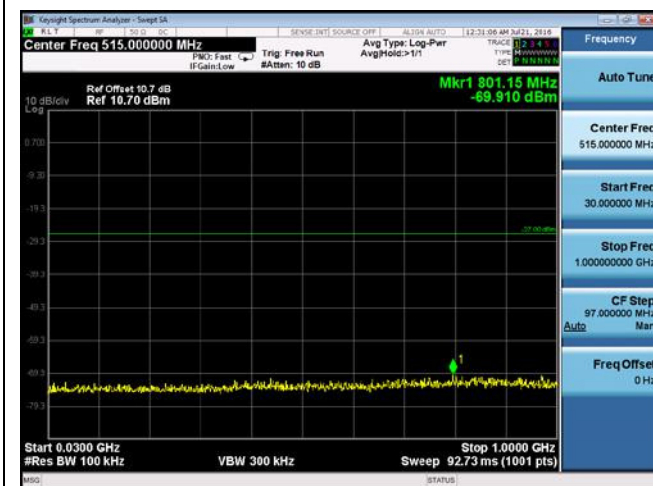
CUE-802.11n-40-5190M-chain2(30MHz-1GHz)
