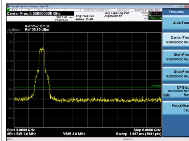
CUE-802.11n-40-5190M -chain3(5GHz-6GHz)
