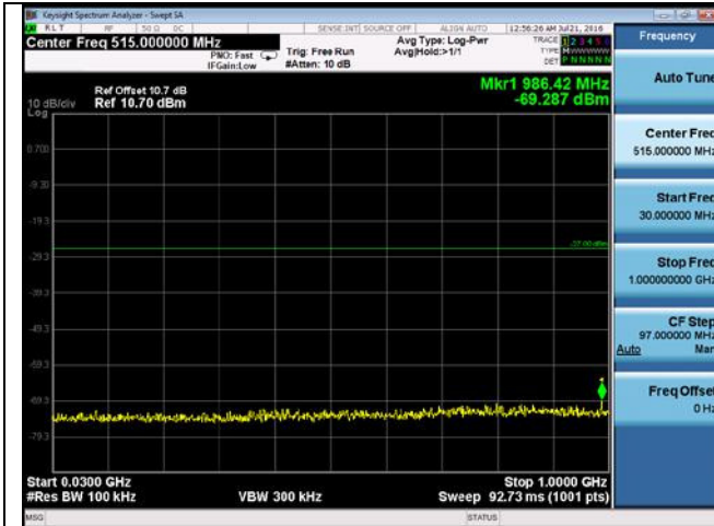
CUE-802.11a-5200M-chain3(30MHz-1GHz)
