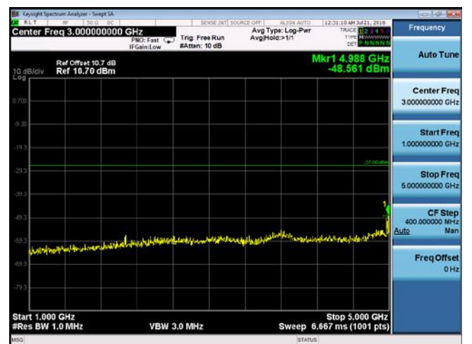
CUE-802.11n-40-5190M-chain2(1GHz-5GHz)
