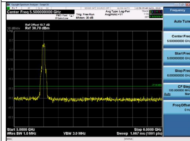
CUE-802.11a-5200M-chain3(5GHz-6GHz)
