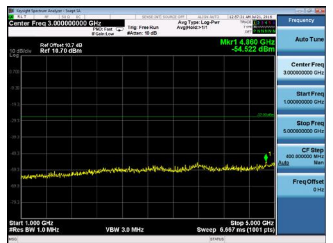
CUE-802.11a-5240M-chain 3(1GHz-5GHz)
