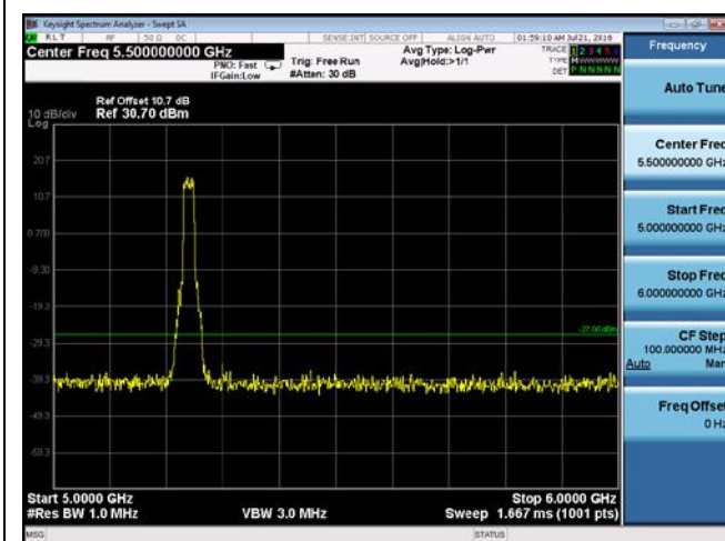
CUE-802.11n-20-5240M-chain 4(5GHz-6GHz)
