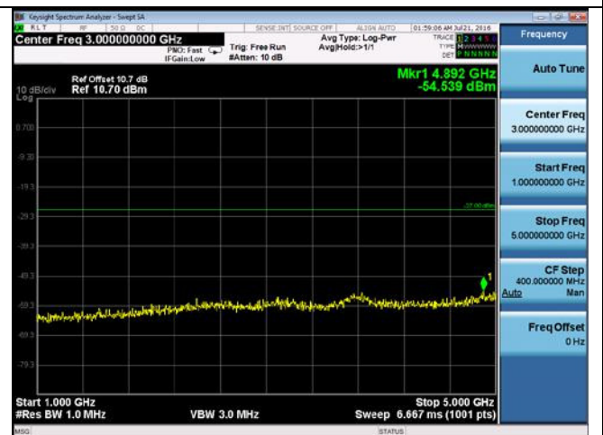
CUE-802.11n-20-5240M-chain 4(1GHz-5GHz)
