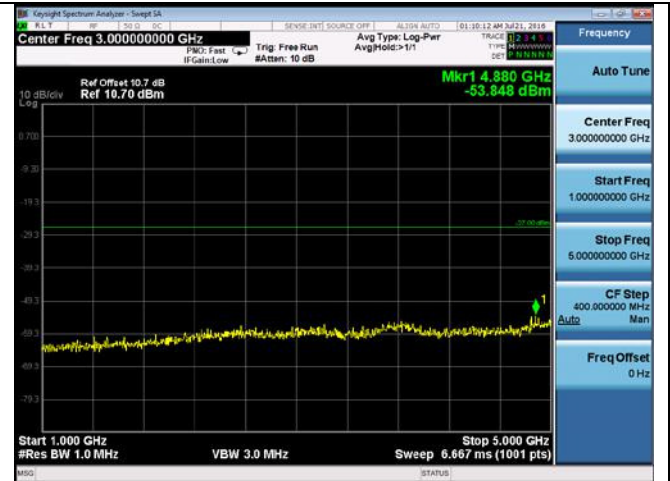
CUE-802.11n-20-5200M-chain3(1GHz-5GHz)
