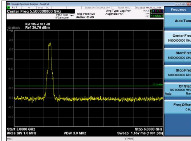
CUE-802.11n-20-5240M-chain 3(5GHz-6GHz)
