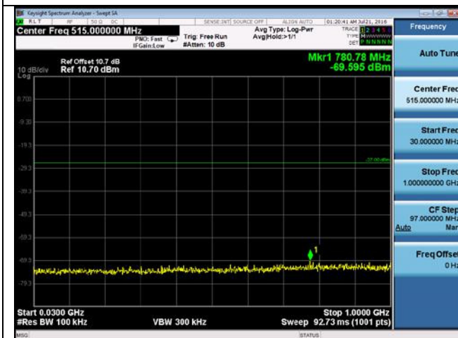
CUE-802.11n-40-5190M -chain3(30MHz-1GHz)
