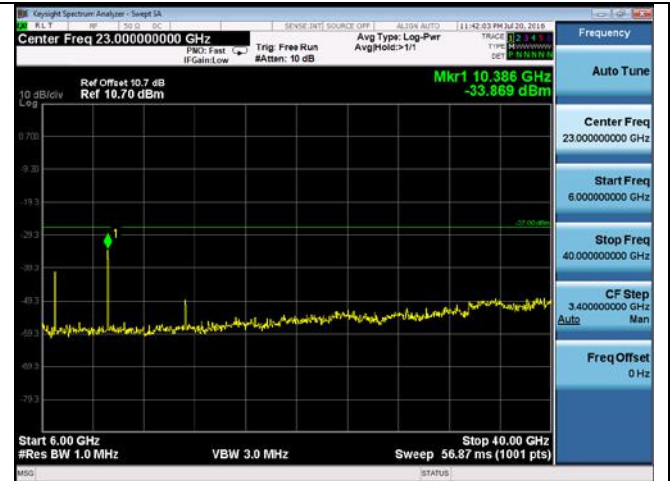
CUE-802.11n-20-5200M-chain1(6GHz-40GHz)
