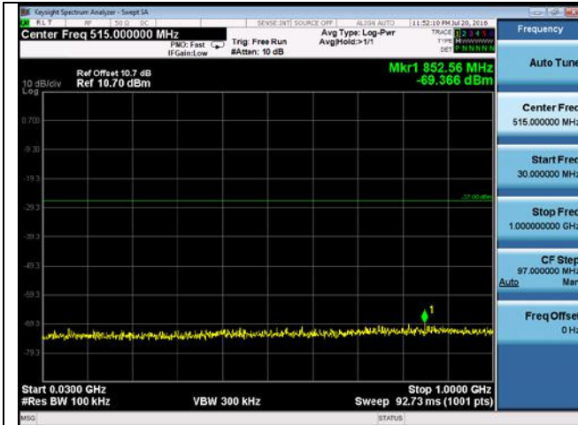
CUE-802.11n-40-5190M-chain1(30MHz-1GHz)
