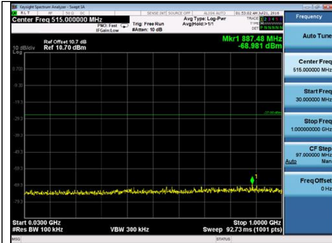
CUE-802.11a-5745M-chain4(30MHz-1GHz)
