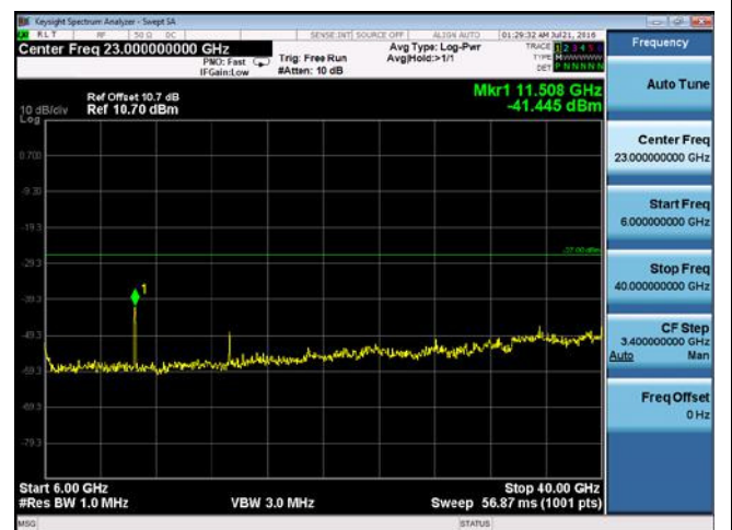
CUE-802.11n-40-5755M -chain3(6GHz-40GHz)
