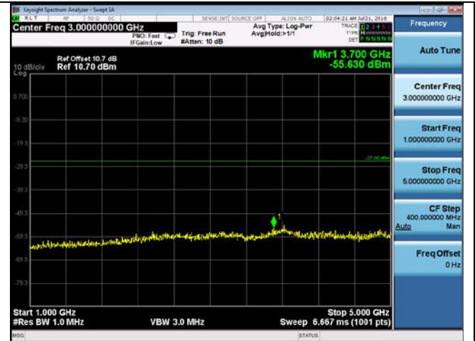
CUE-802.11n-20-5745M-chain4(1GHz-5GHz)
