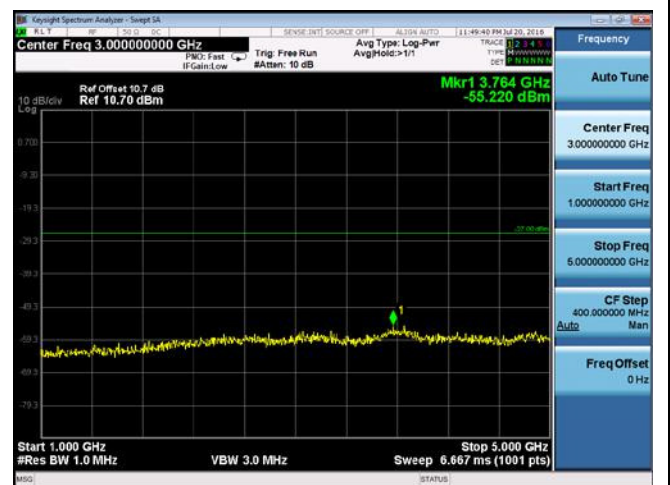
CUE-802.11n-20-5785M-chain1(1GHz-5GHz)
