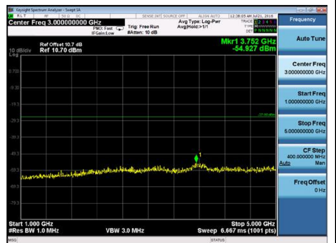
CUE-802.11n-40-5755M-chain2(1GHz-5GHz)
