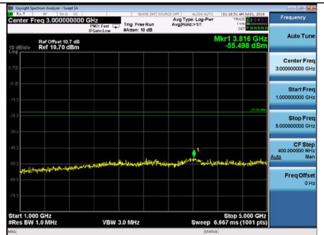
CUE-802.11n-20-5745M -chain3(1GHz-5GHz)
