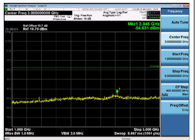
CUE-802.11n-20-5745M-chain2(1GHz-5GHz)
