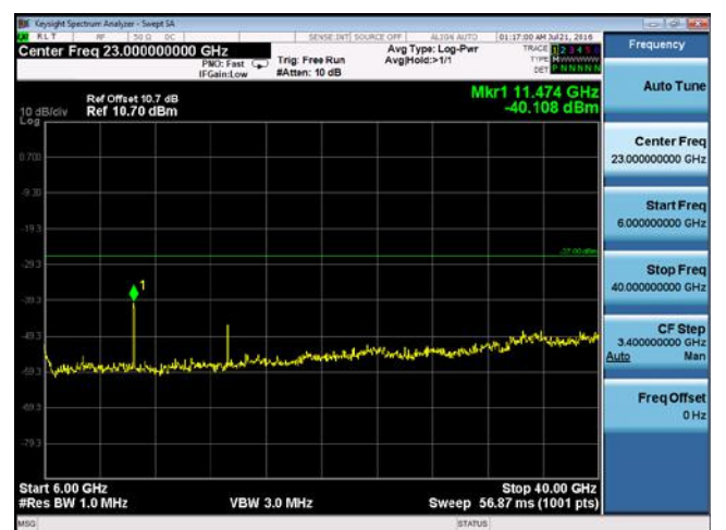
CUE-802.11n-20-5745M chain3(6GHz-40GHz)
