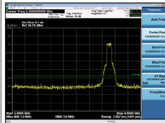
CUE-802.11n-40-5755M -chain3(5GHz-6GHz)
