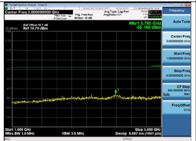
CUE-802.11a-5825M-chain 1(1GHz-5GHz)
