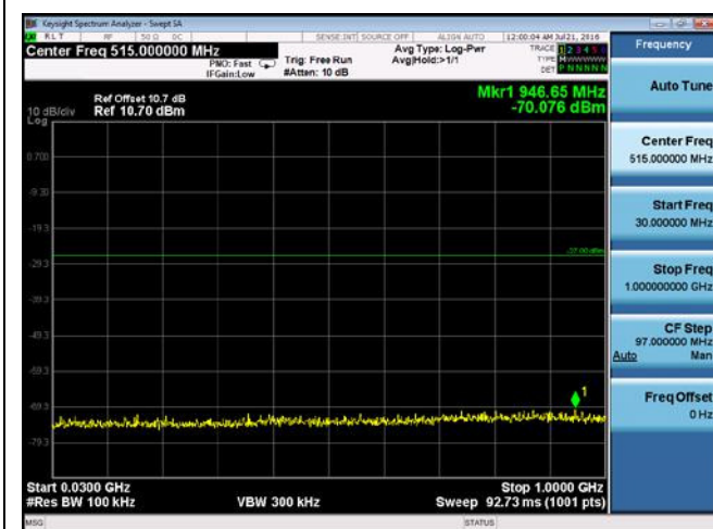
CUE-802.11n-40-5795M-chain1(30MHz-1GHz)
