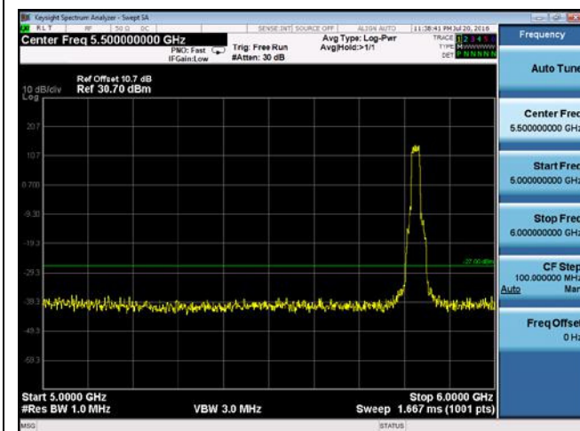
CUE-802.11a-5825M-chain 1(5GHz-6GHz)
