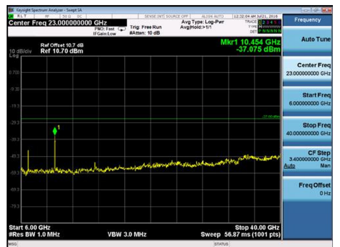
CUE-802.11n-40-5230M -chain2(6GHz-40GHz)
