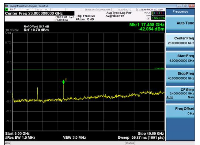
CUE-802.11a-5825M-chain 1(6GHz-40GHz)
