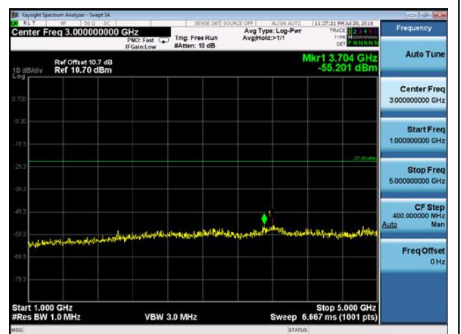
CUE-802.11a-5785M-chain1(1GHz-5GHz)
