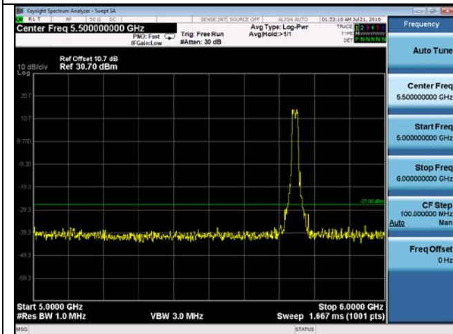
CUE-802.11a-5745M-chain4(5GHz-6GHz)
