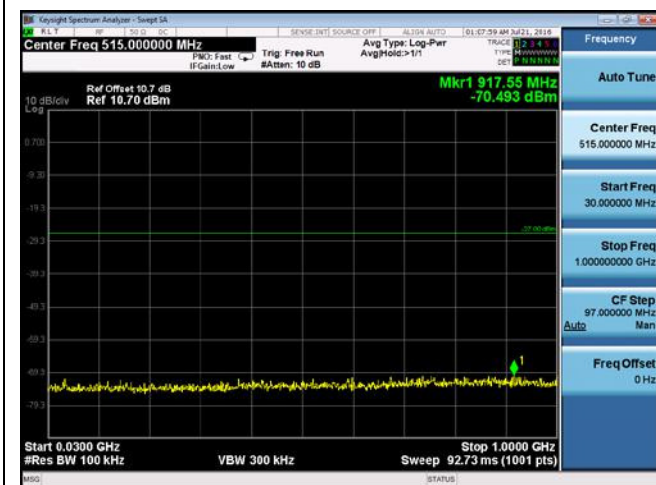
CUE-802.11a-5825M chain 3(30MHz-1GHz)
