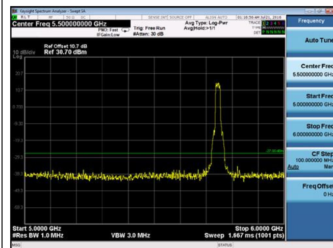
CUE-802.11n-20-5745M -chain3(5GHz-6GHz)
