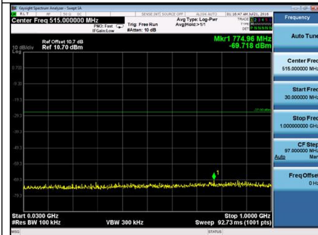
CUE-802.11n-20-5745M -chain3(30MHz-1GHz)
