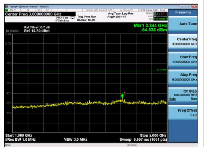
CUE-802.11n-40-5795M-chain1(1GHz-5GHz)
