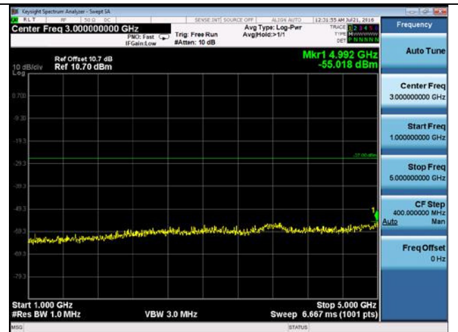
CUE-802.11n-40-5230M chain2(1GHz-5GHz)
