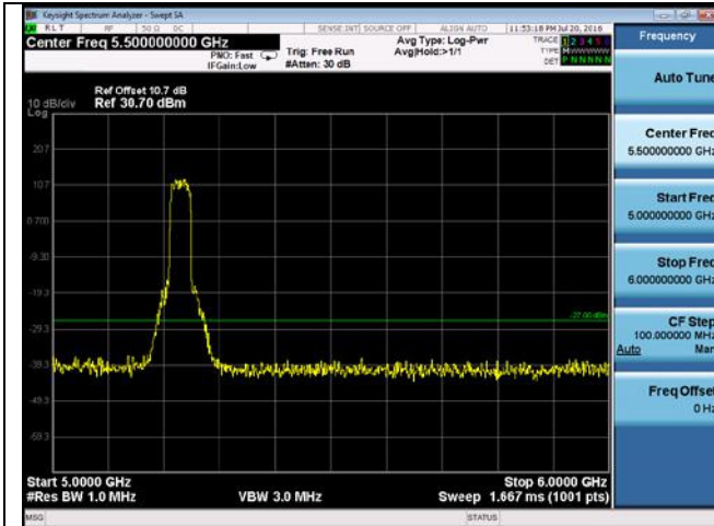
CUE-802.11n-40-5230M -chain1(5GHz-6GHz)
