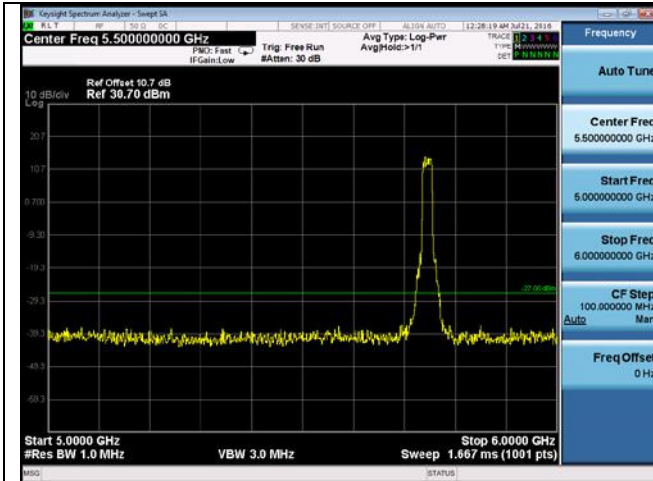
CUE-802.11n-20-5745M -chain2(5GHz-6GHz)
