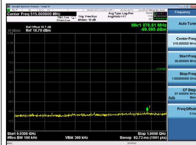
CUE-802.11a-5785M-chain1(30MHz-1GHz)
