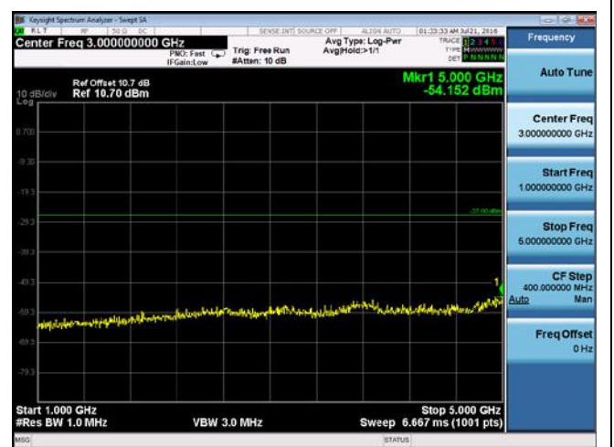
CUE-802.11ac-80-5210M -chain 3(1GHz-5GHz)
