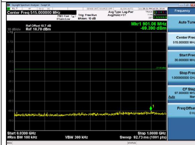
CUE-802.11a-5825M-chain 1(30MHz-1GHz)
