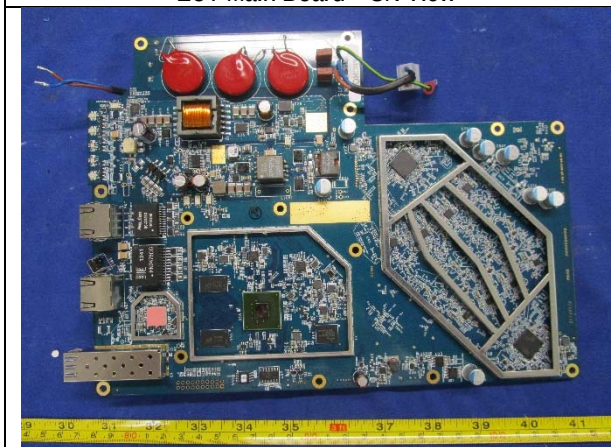
EUT Main Board without Shielding – Bottom View
