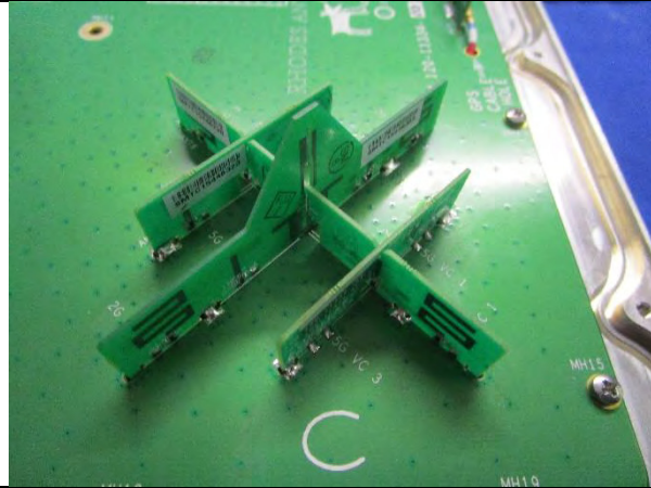
EUT Antennas – Group C Antenna Assembly
