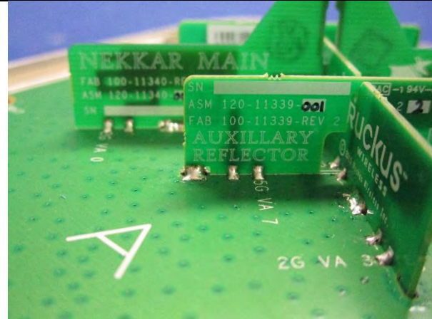
EUT Antenna Group A – PCB 2 of 4 – View 1
