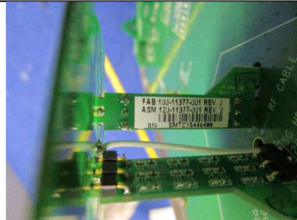
EUT Antenna Group D – PCB 4 of 4
