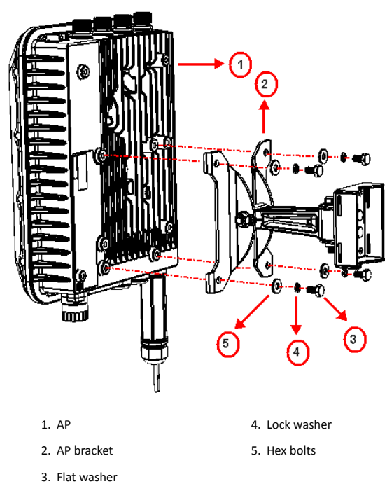
FIGURE 10 Attaching the AP bracket to the AP
