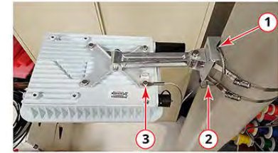
FIGURE 24 Attaching the security cable
