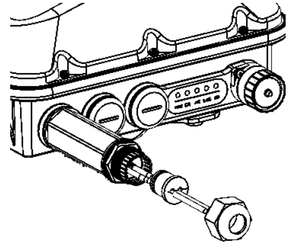
FIGURE 4 Zipcord grommet with cable
