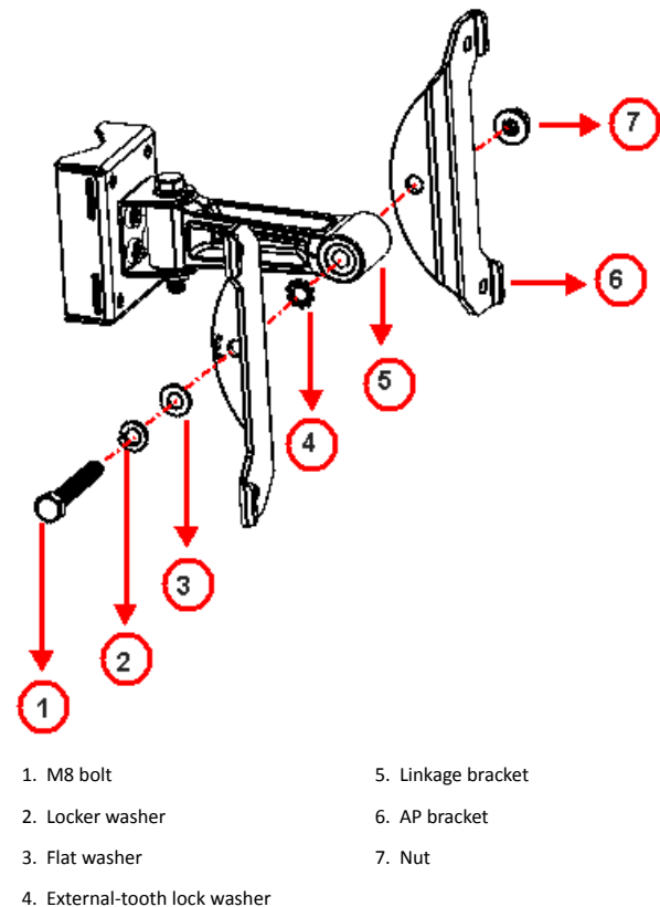
FIGURE 9 Attach the linkage bracket to the AP bracket
