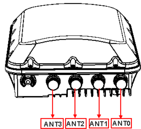
FIGURE 11 T750SE Rear View
