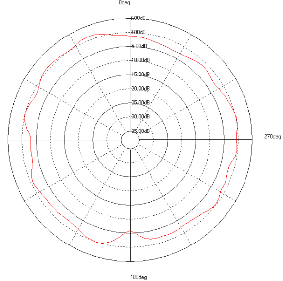
Horizontal Polarity Elevation Pattern 5150 – 5875 MHz:
