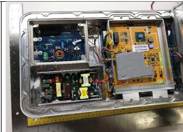
EUT Antenna-Borad Off View
