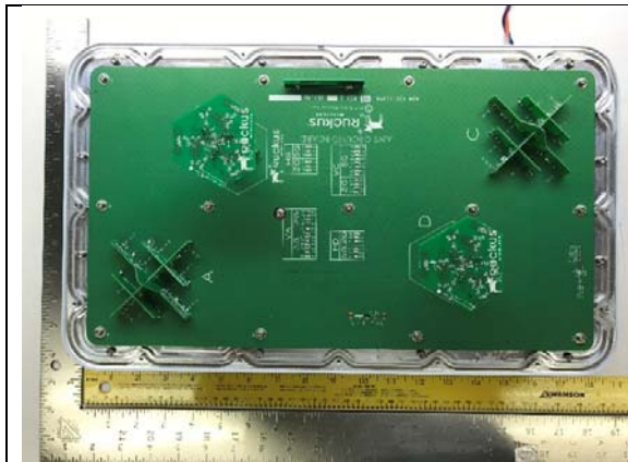
Antenna- Top View
