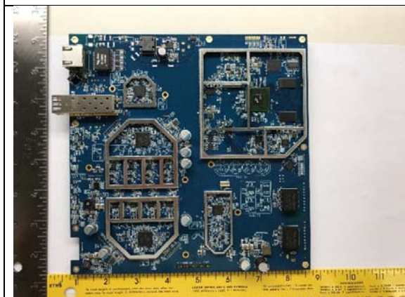
AP Board – Top View
