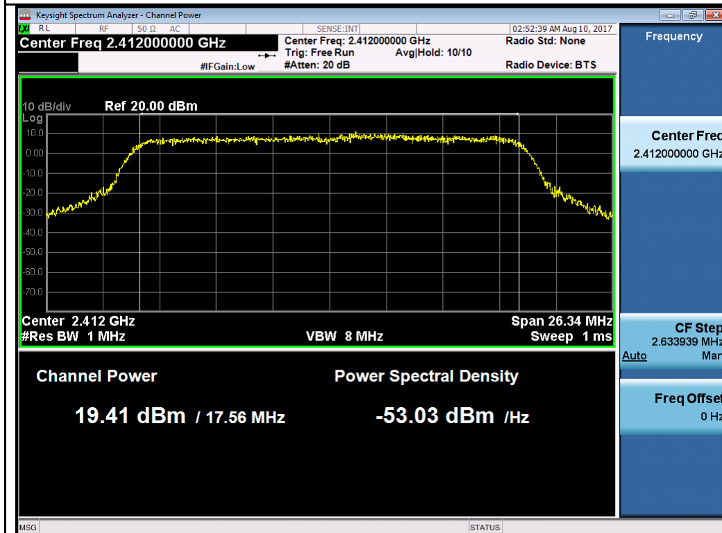
802.11n-HT20 2412MHz Chain 1
