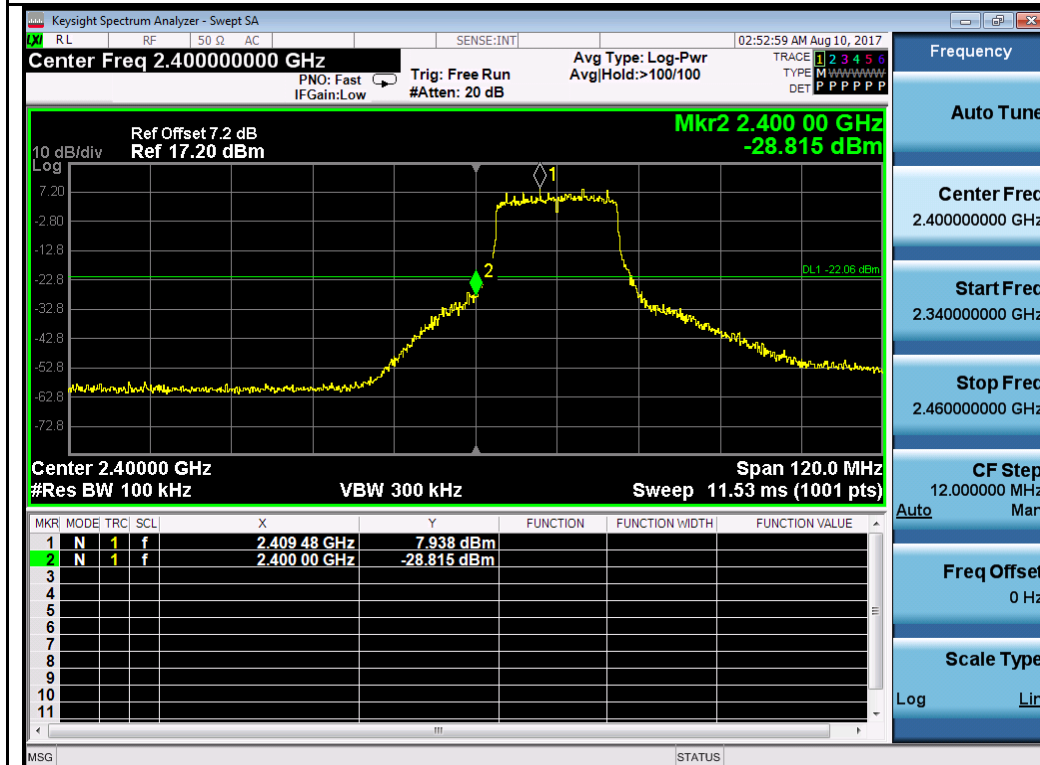
802.11n-HT20-2412MHz Chain 1
