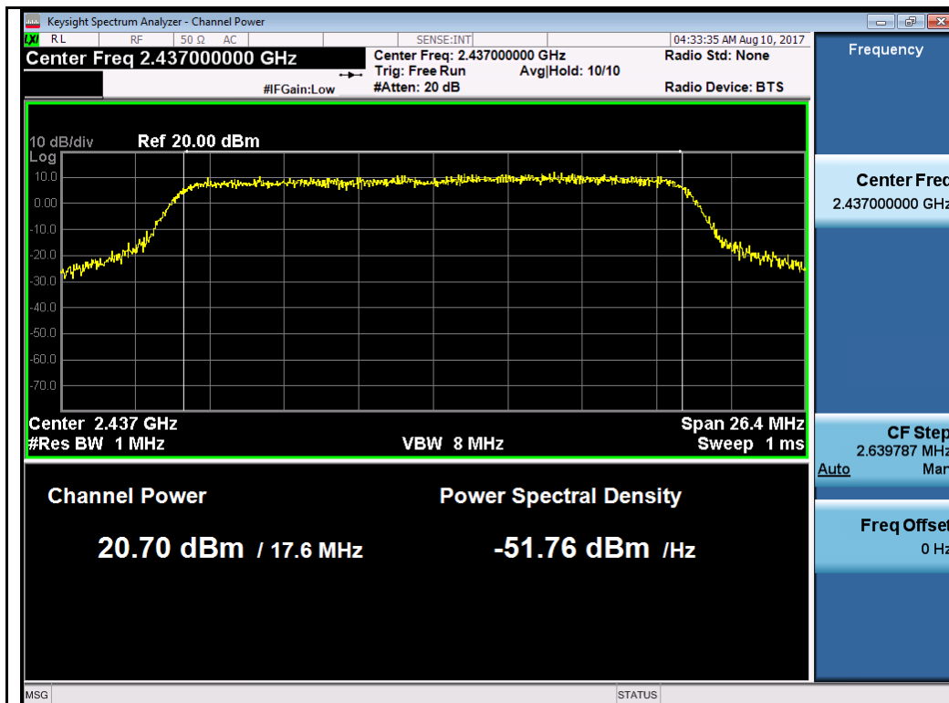
802.11n-HT20 2437MHz Chain 2
