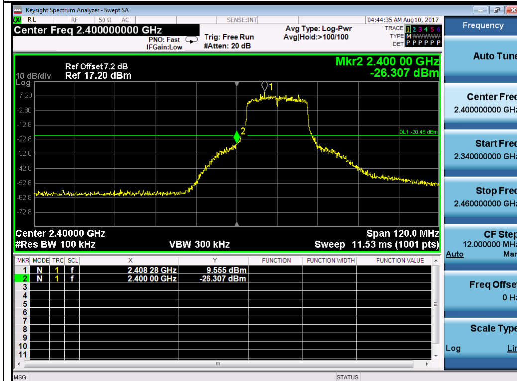
802.11n-HT20-2412MHz Chain 3
