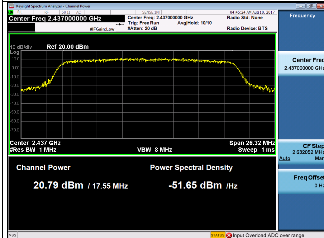
802.11n-HT20 2437MHz Chain 3
