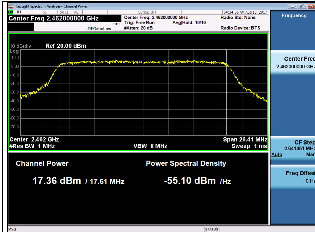
802.11n-HT20 2462MHz Chain 2
