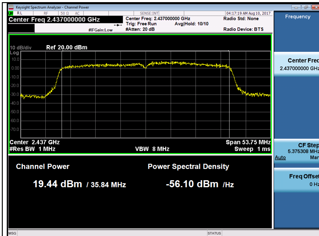
802.11n-HT40 2437MHz Chain 2
