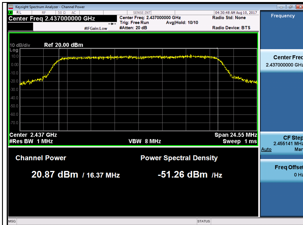
802.11g-2437MHz Chain 2
