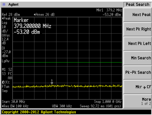
Chain 0 30MHz—1GHz
