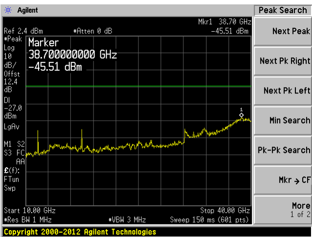
Chain 1 10GHz---40GHz
