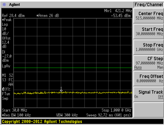
Chain 1 30MHz---1GHz
