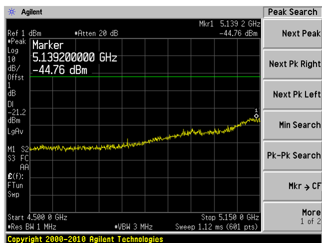
Chain 1 PEAK
