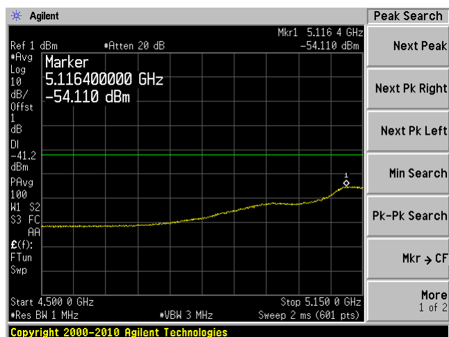
Chain 1 PEAK
