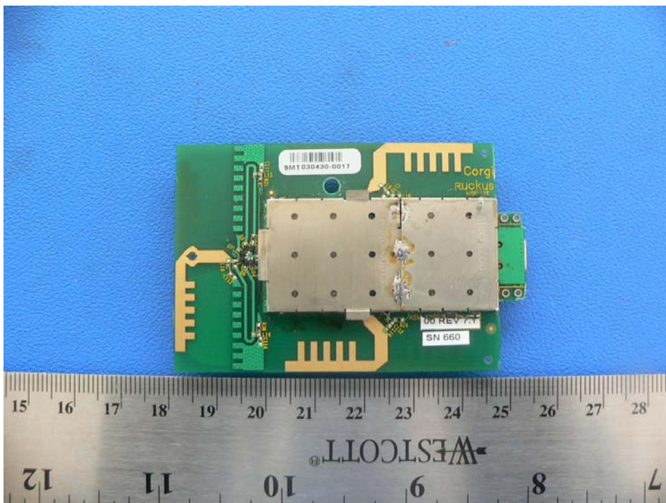
EUT – Main PCB Component Side with Shielding View
