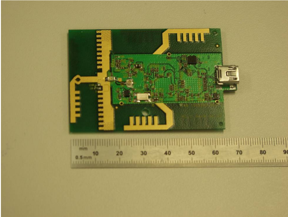
EUT – Main PCB Solder Side View 1
