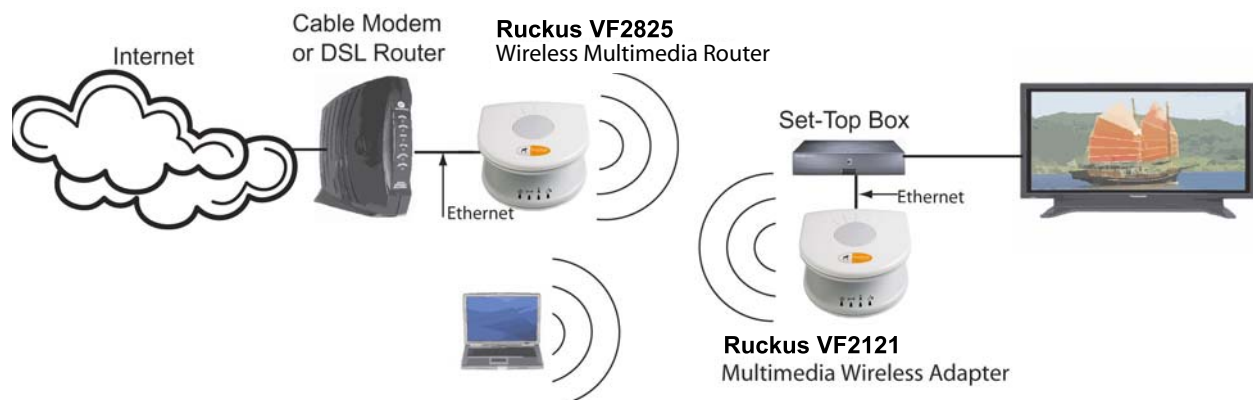
Figure 1 —The VideoFlex 2825 Wireless Multimedia Router in a Typical Home Network
