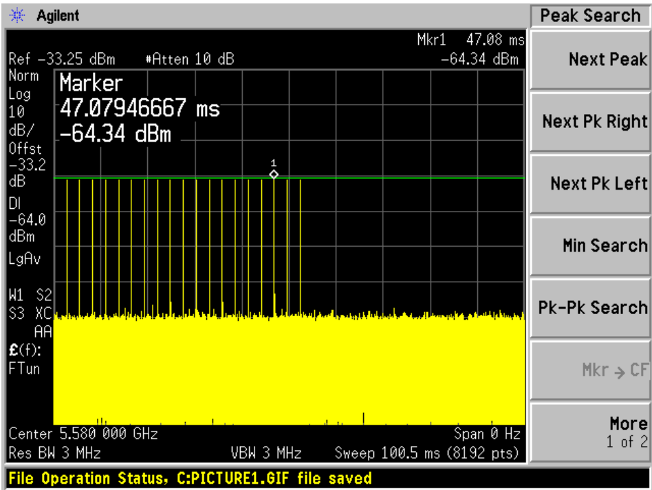
Radar Type 1B
