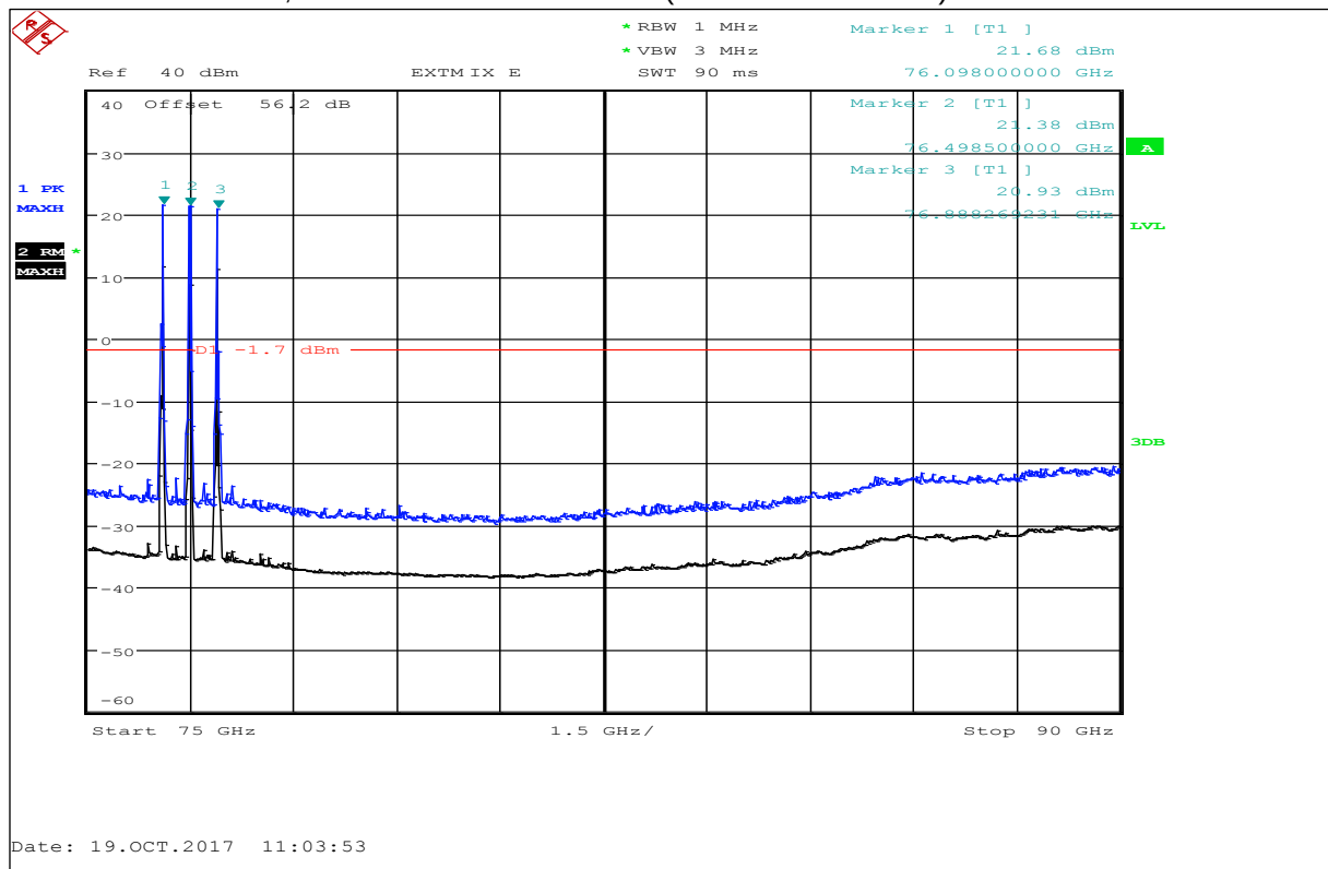
Plot 25: 75 GHz – 90 GHz, antenna vertical / horizontal (valid for all channels)
