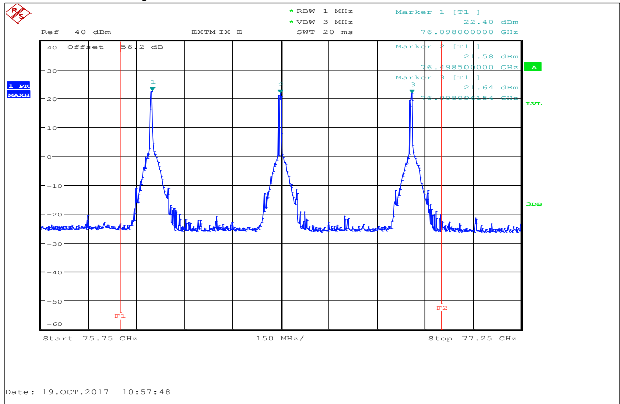
Plot 10: Low, Middle and High Channel, Peak detector, T_{\min} / V_{\min} - V_{\max}
