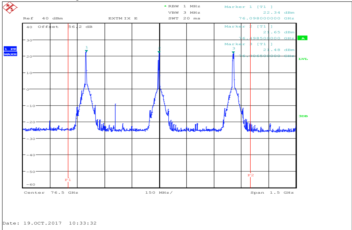
Plot 8: Low, Middle and High Channel, Peak detector, T_{nom} / V_{nom}
