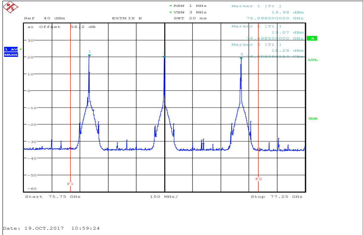
Plot 9: Low, Middle and High Channel, RMS detector, T_{\min} / V_{\min} - V_{\max}
