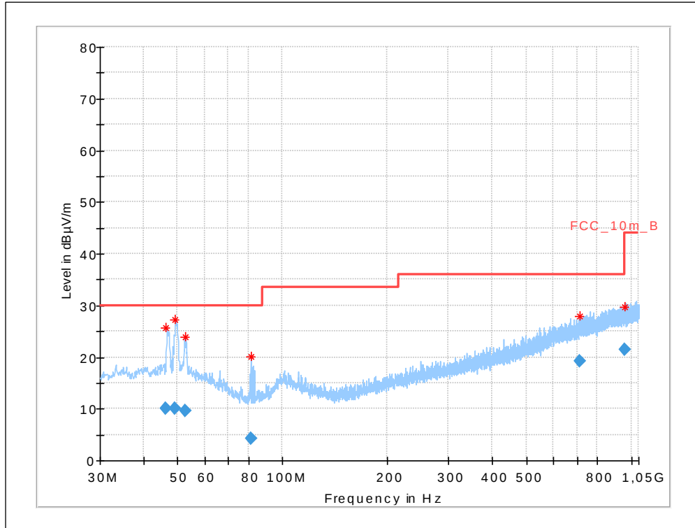
Plot 18: 30 MHz – 1 GHz, antenna vertical / horizontal (Middle channel)
