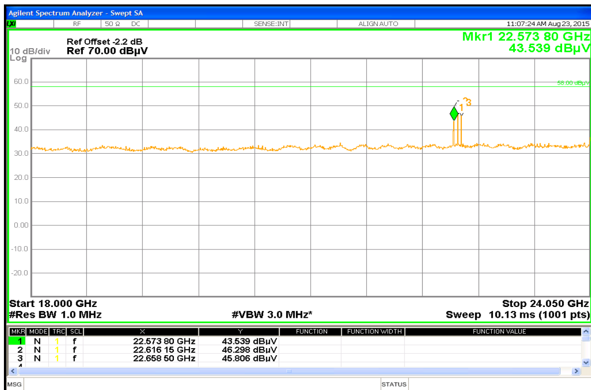
Plot No. 14: 18 GHz to 24.05 GHz, low/mid/high frequency, horizontal/vertical polarization
