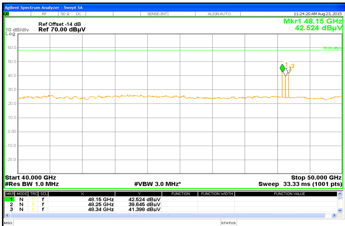
Plot No. 17: 40 GHz to 50 GHz, low/mid/high frequency, horizontal/vertical polarization
