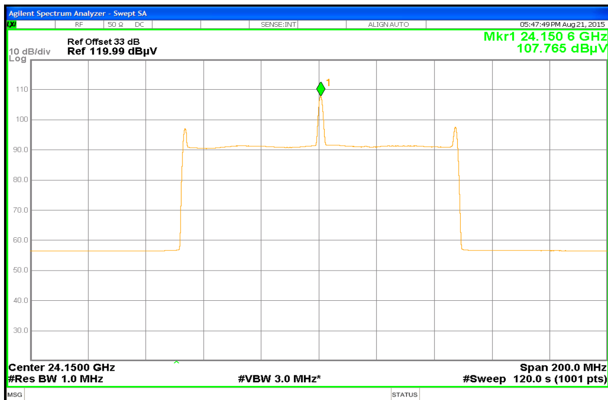
Plot No. 2: Average measurement, normal operation mode
