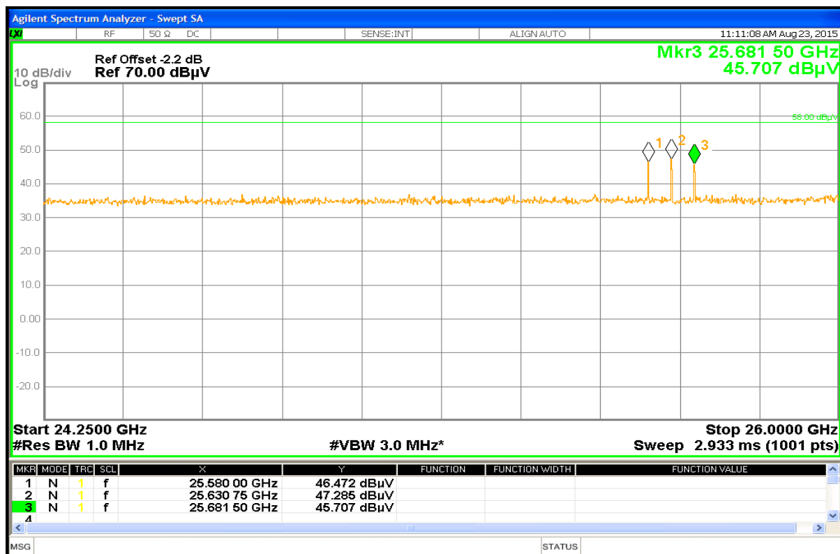
Plot No. 15: 24.25 GHz to 26 GHz, low/mid/high frequency, horizontal/vertical polarization
