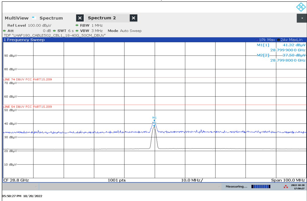
Plot 11: 28.8 GHz, antenna vertical / horizontal, valid for specified modes
