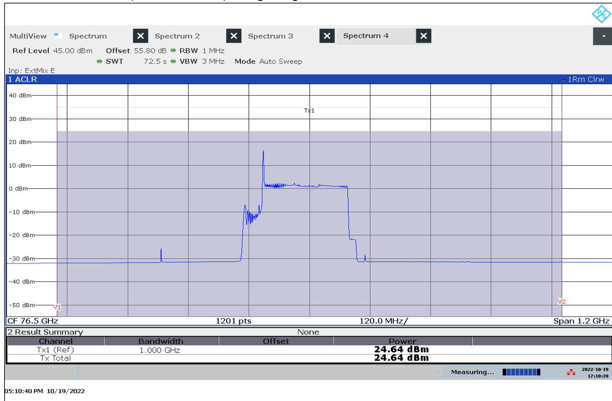
Plot 1: EIRP Mean Power (Channel Power), Long Range, T_{nom} / V_{nom}
