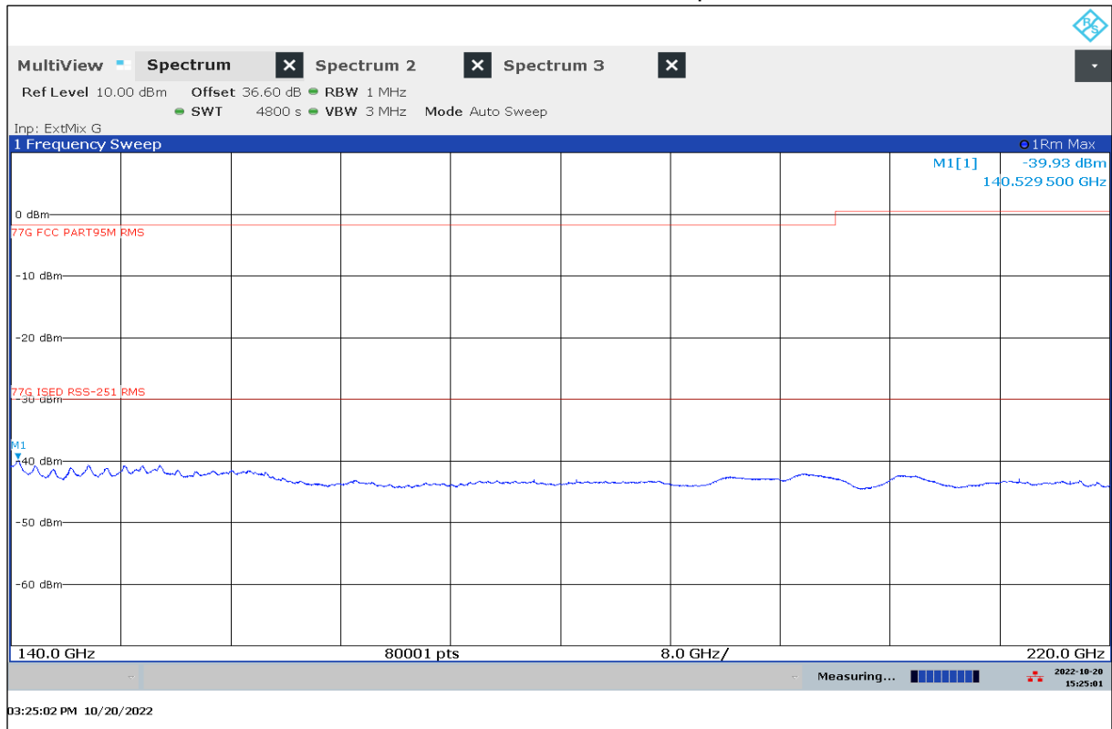
Plot 17: 140 GHz – 220 GHz, antenna vertical / horizontal, valid for specified modes
