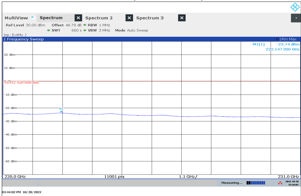
Plot 18: 220 GHz to 231 GHz, horizontal / vertical polarization, valid for specified modes
