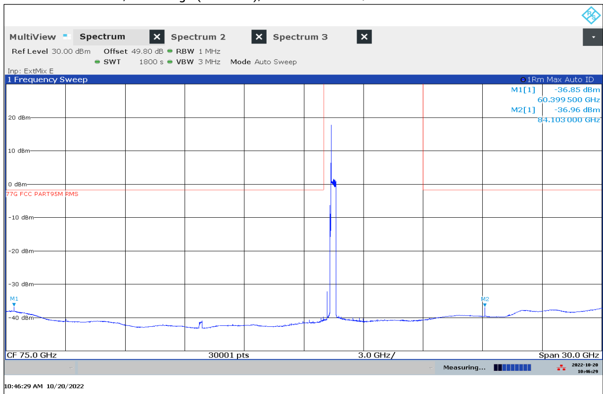
Plot 14: 60 GHz – 90GHz, Mid-Range (215 MHz), antenna vertical / horizontal
