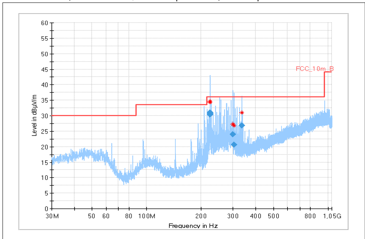
Plot 8: 30 MHz – 1 GHz, antenna vertical / horizontal polarization, valid for specified modes
