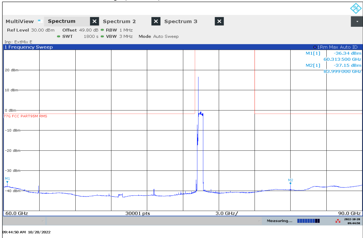
Plot 15: 60 GHz – 90GHz, Short Range (375 MHz), antenna vertical / horizontal
