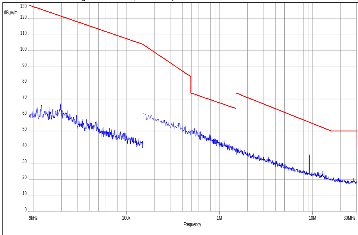
Plot 7: 9 kHz – 30 MHz, Magnetic antenna, valid for specified modes
