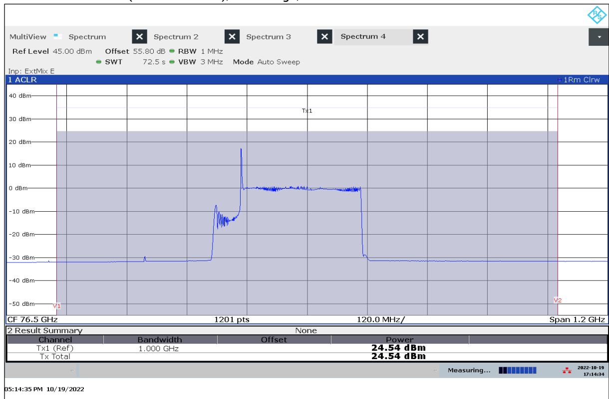
Plot 3: EIRP Mean Power (Channel Power), Mid Range, T_{nom} / V_{nom}
