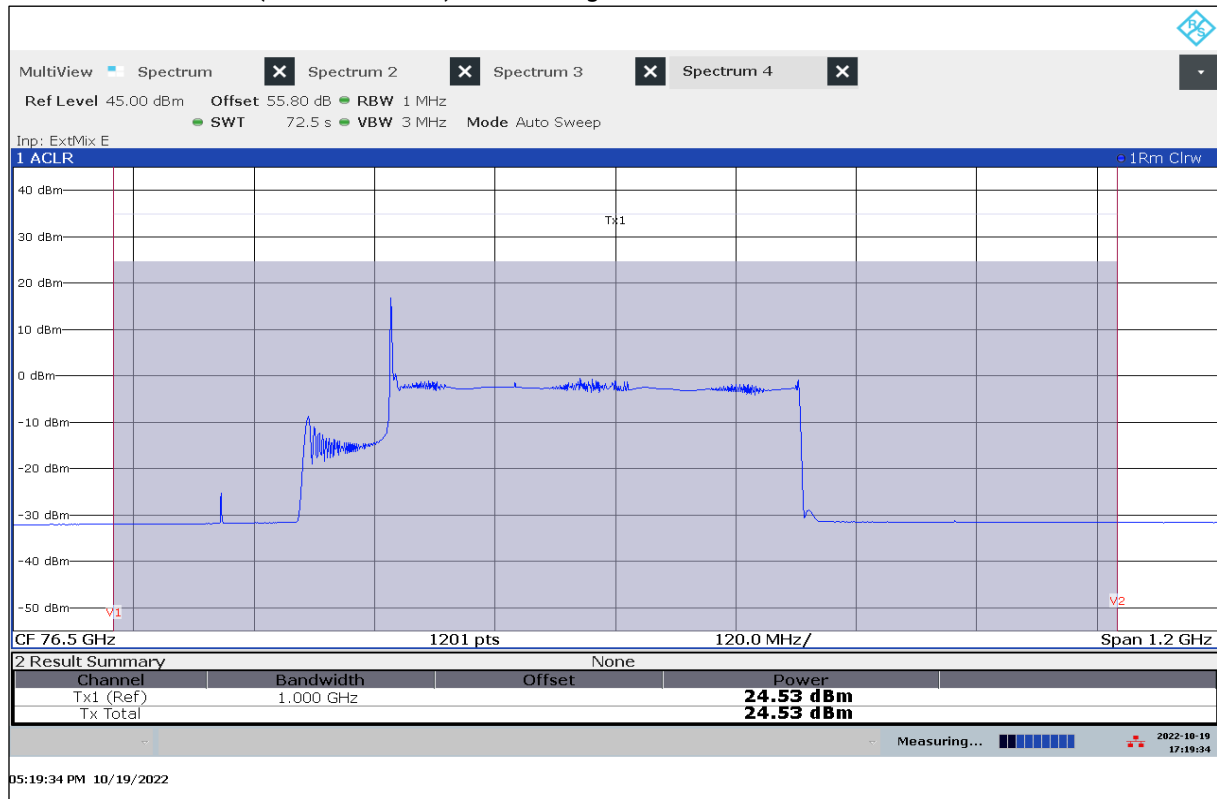
Plot 5: EIRP Mean Power (Channel Power), Short Range, T_{nom} / V_{nom}
