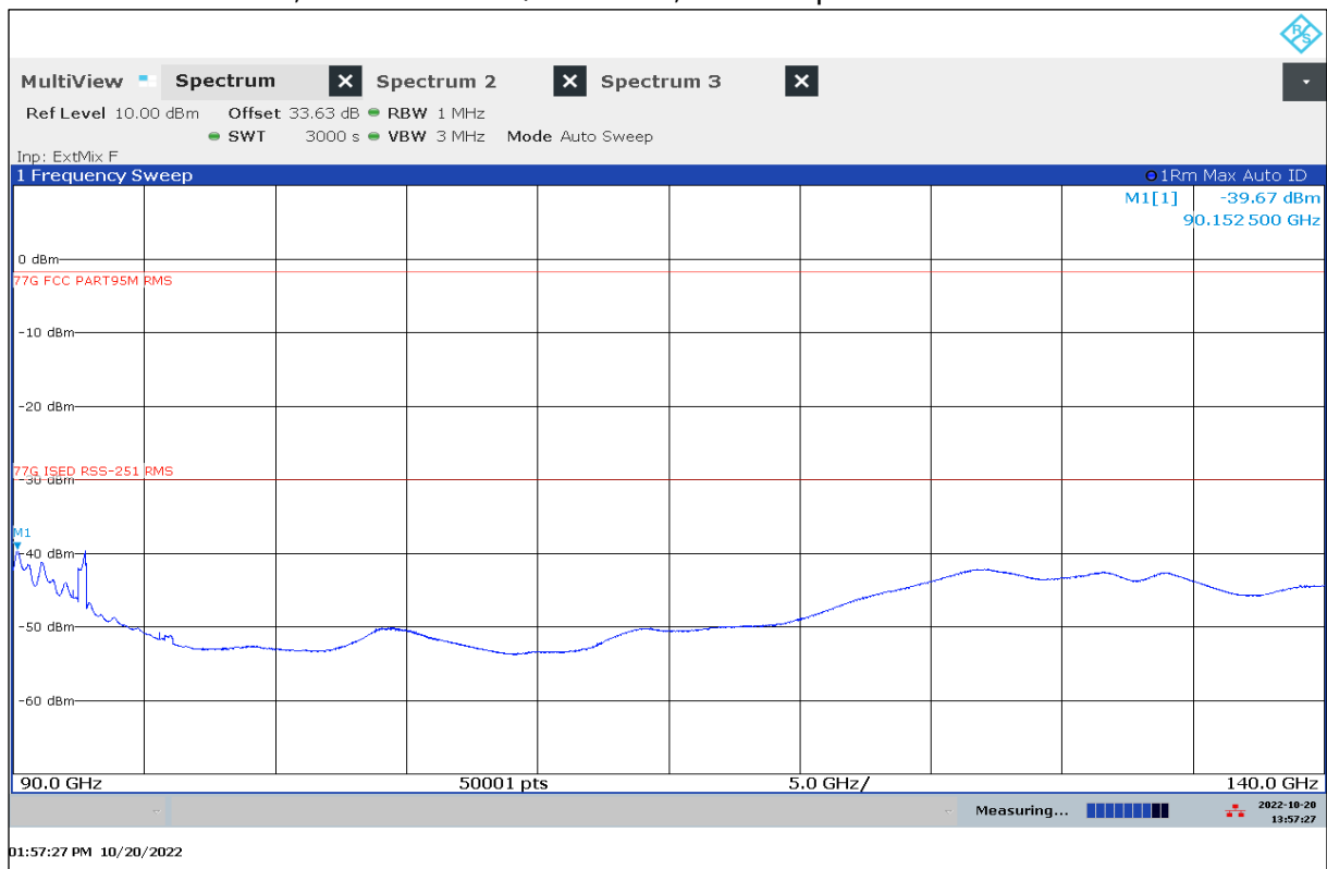
Plot 16: 90 GHz – 140 GHz, antenna vertical / horizontal, valid for specified modes
