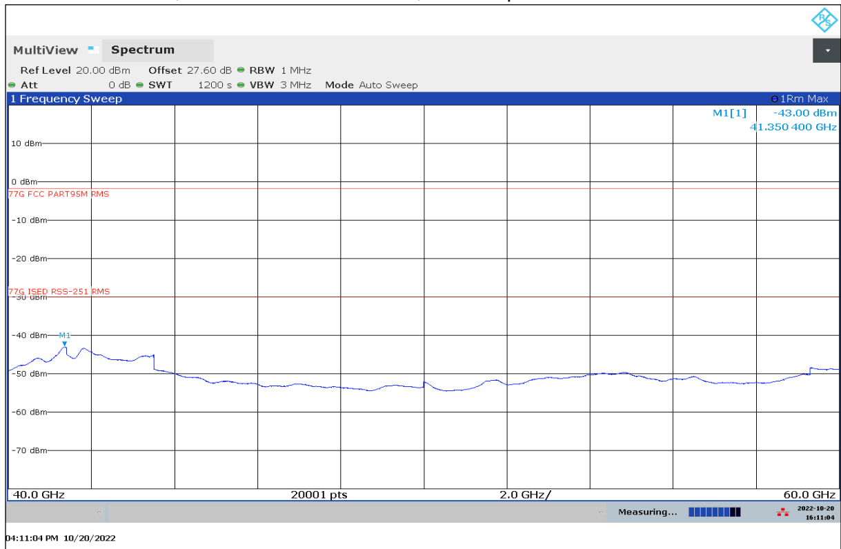
Plot 12: 40 GHz – 60 GHz, antenna vertical / horizontal, valid for specified modes
