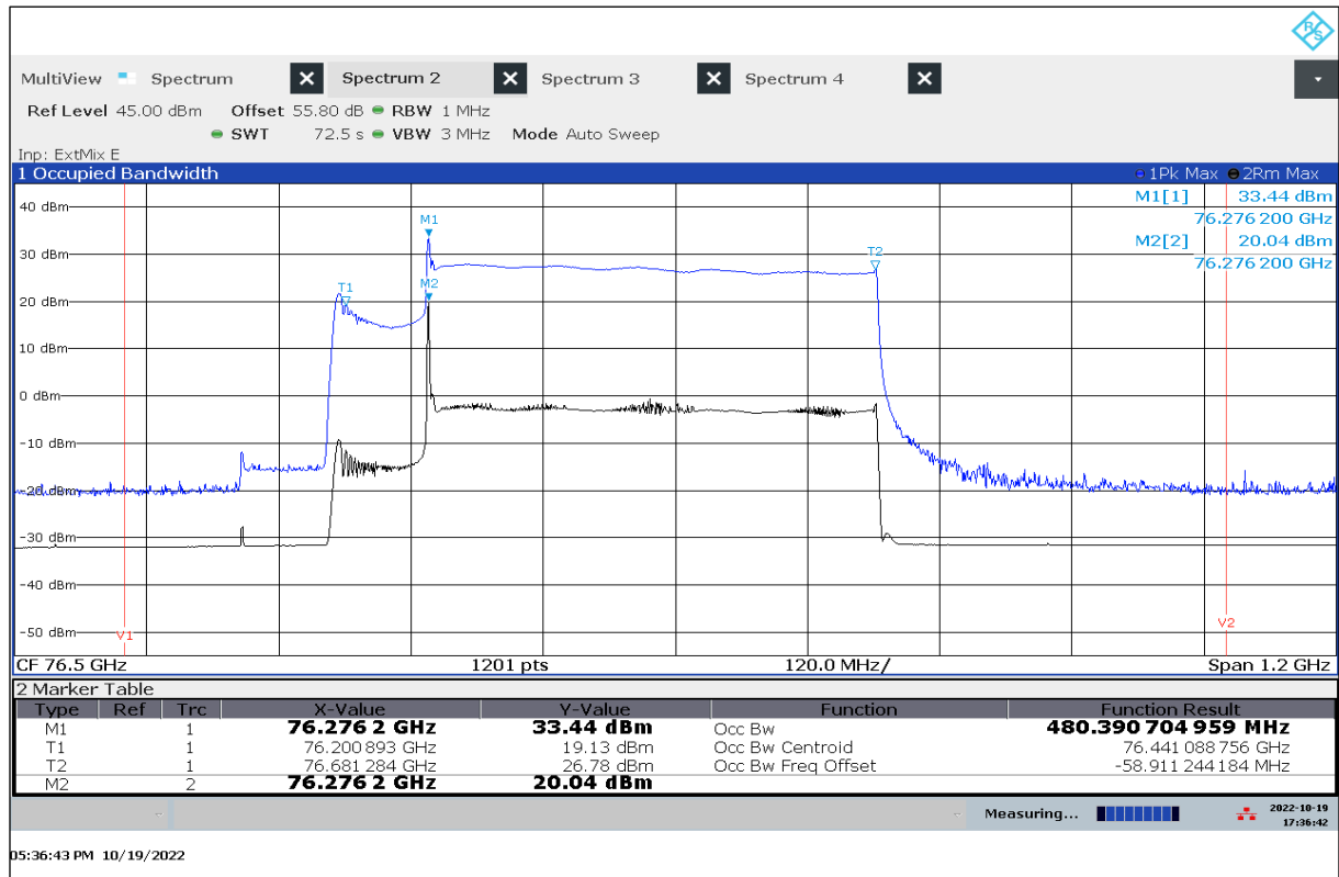
Plot 25: OBW, +30 °C / V_{nom}
