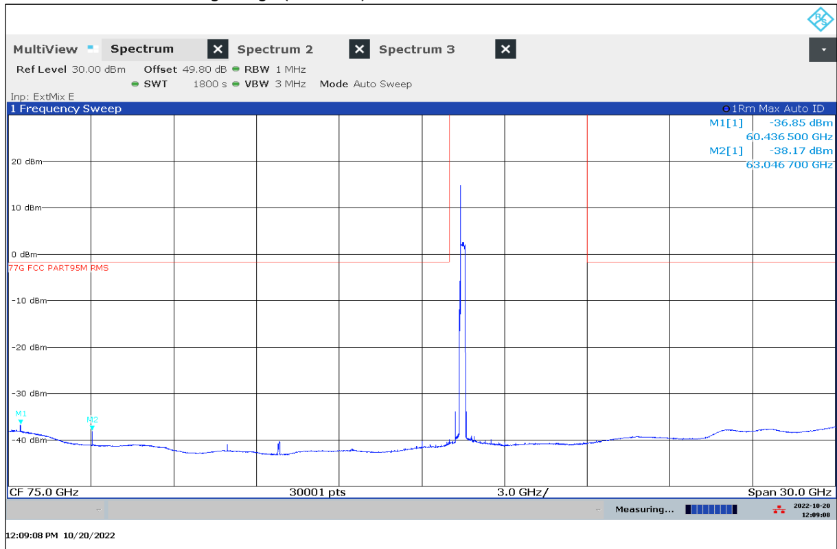
Plot 13: 60 GHz – 90GHz, Long Range (150 MHz), antenna vertical / horizontal
