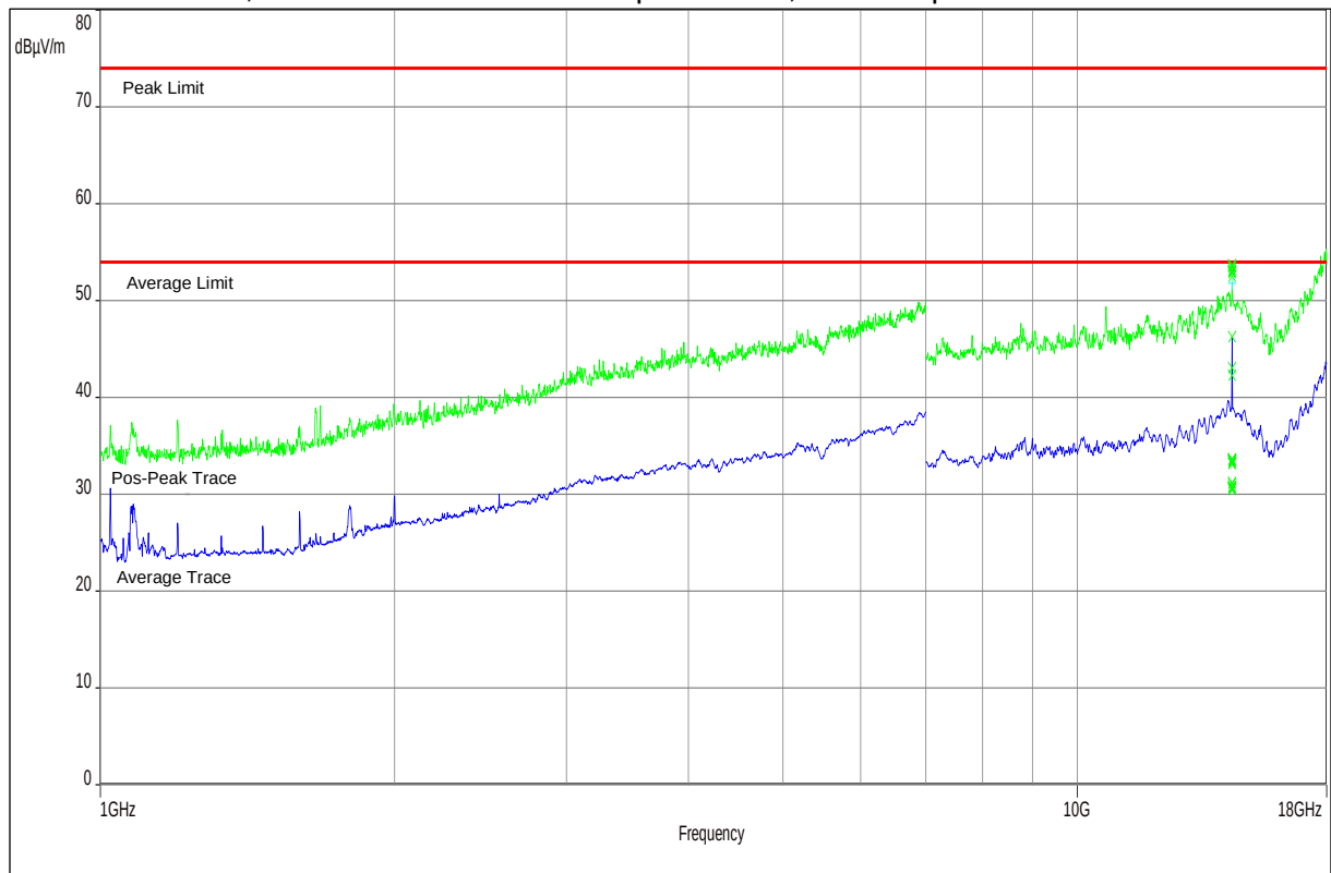
Plot 9: 1 GHz – 18 GHz, antenna vertical / horizontal polarization, valid for specified modes
