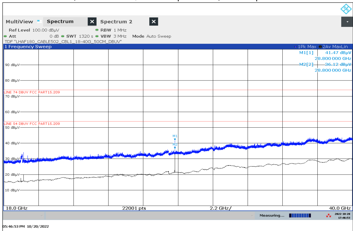
Plot 10: 18 GHz – 40 GHz, antenna vertical / horizontal polarization, valid for specified modes
