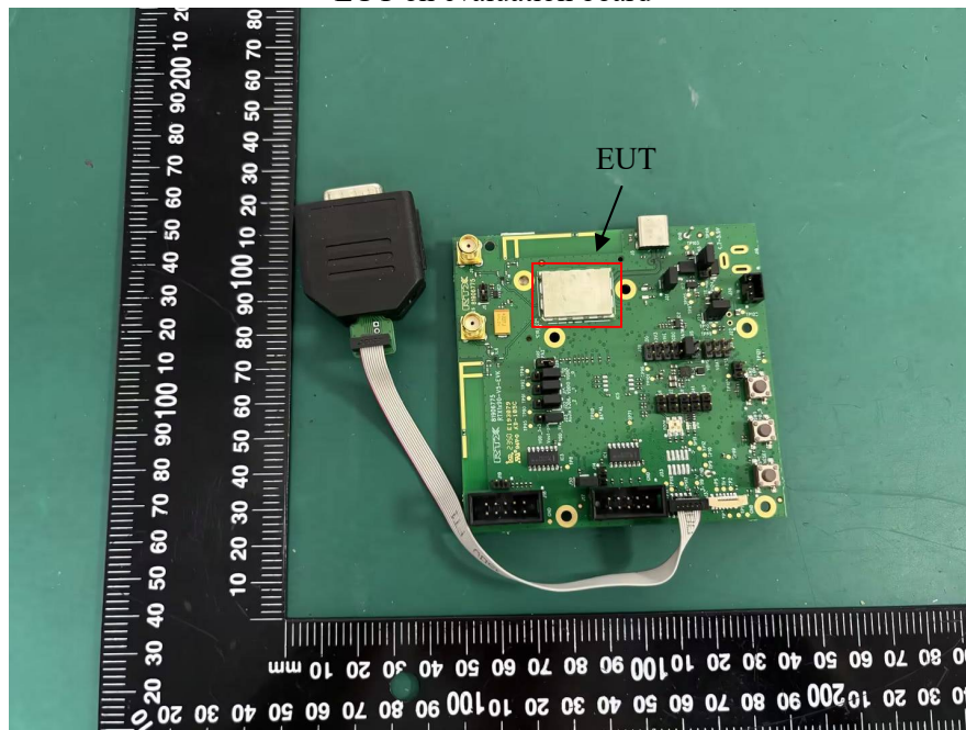
EUT on evaluation board
