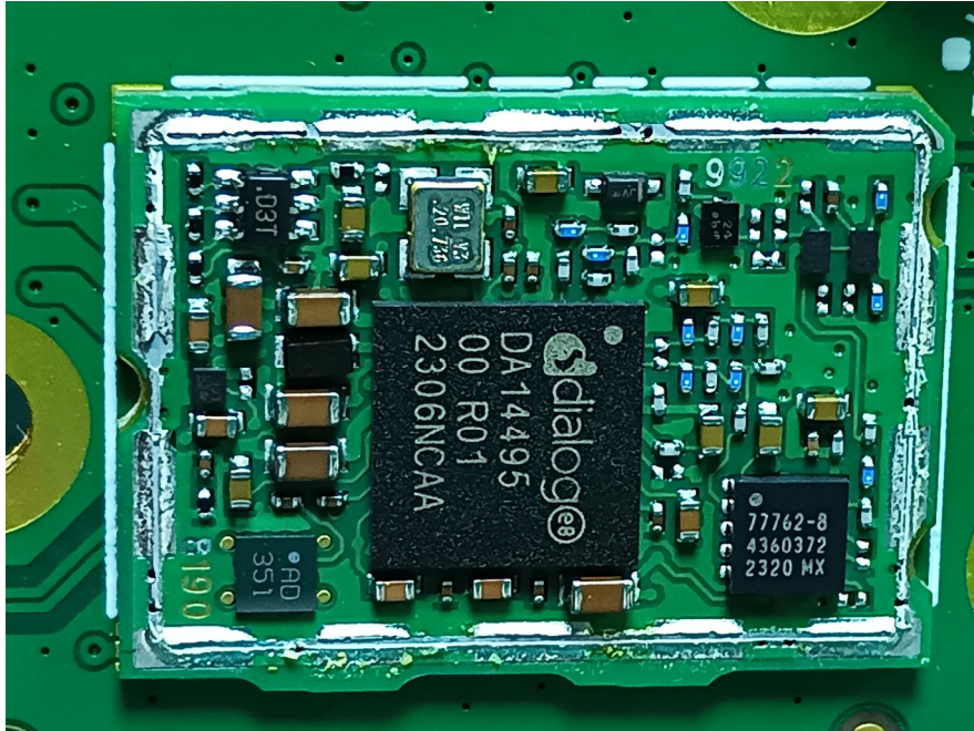
RTX1090R1 module shielding cover off
