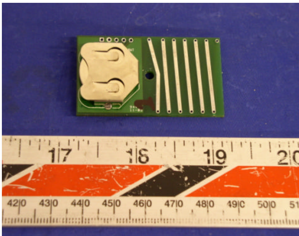
EUT – Solder View
