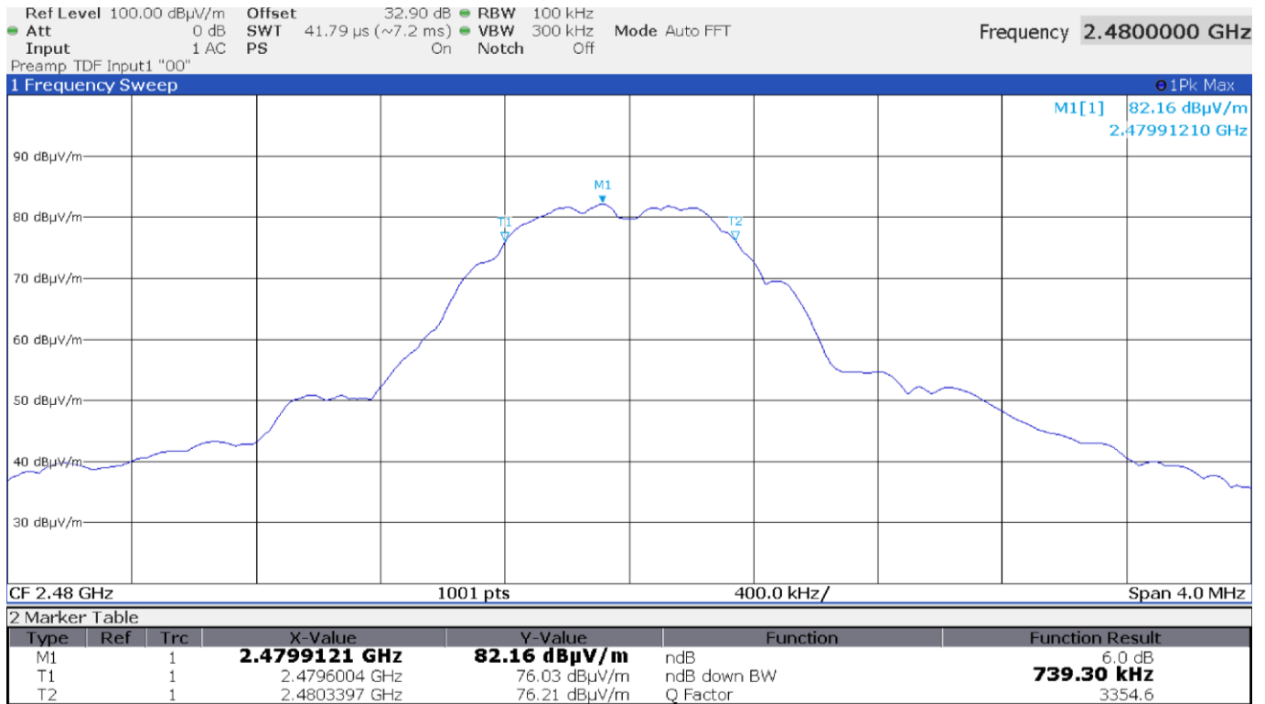
Figure 8.5-3: 6 dB bandwidth – high channel
