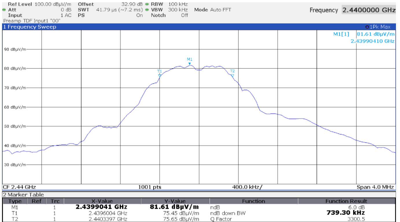
Figure 8.5-2: 6 dB bandwidth – mid channel
