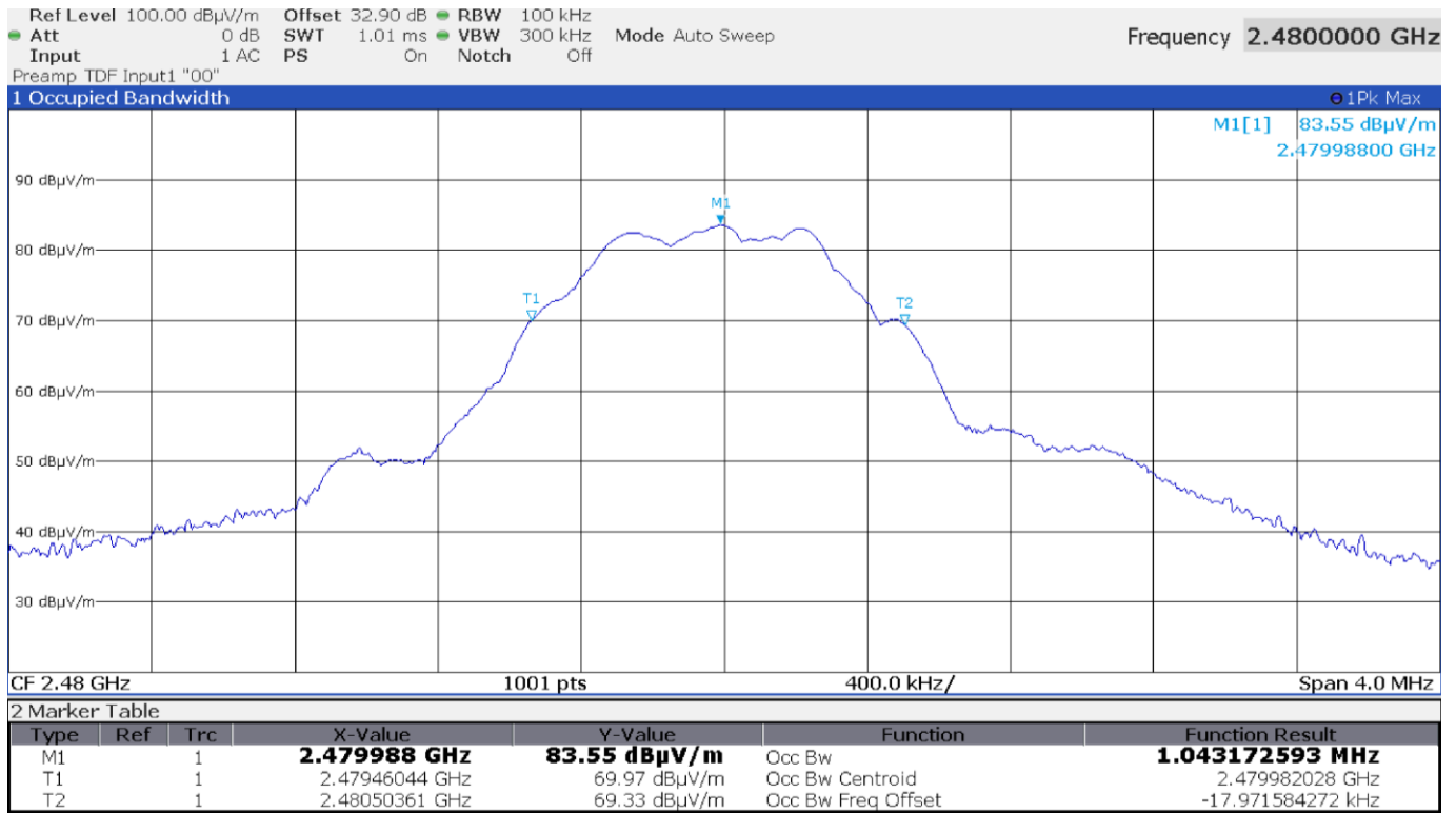
Figure 8.5-6: 99% bandwidth – high channel
