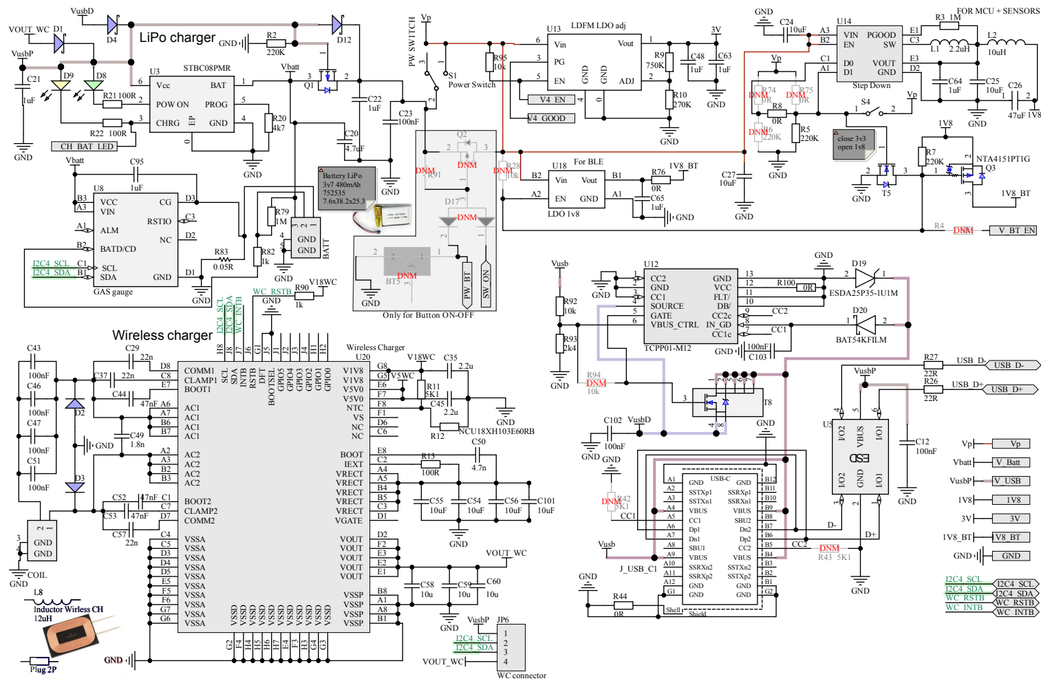
Figure 29. Sensortilebox_pro_Power
