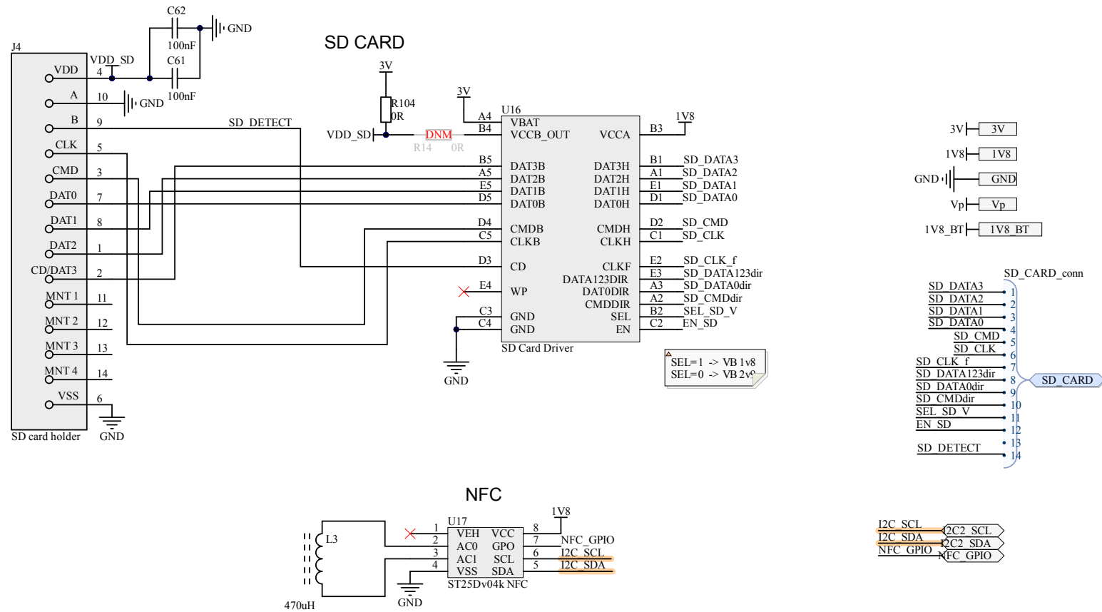
Figure 33. Sensortilebox_pro_Peripherals
