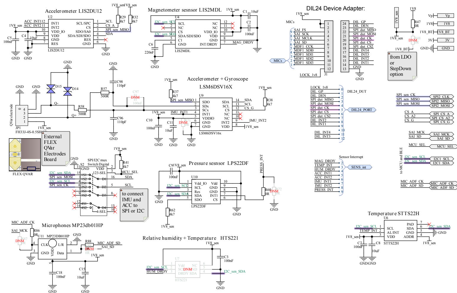
Figure 31. Sensortilebox_pro_sensors
