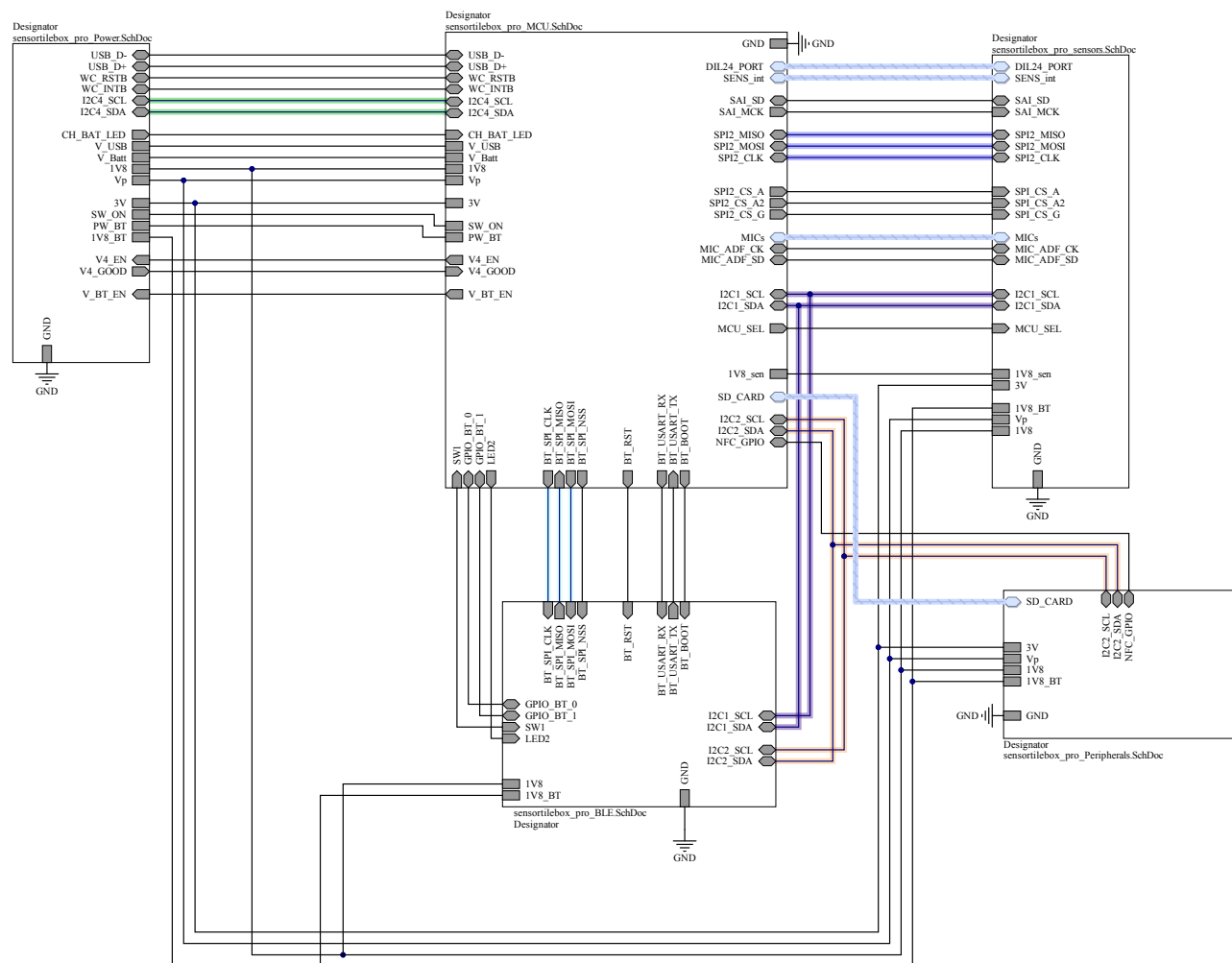
Figure 28. Sensortilebox_pro_main
