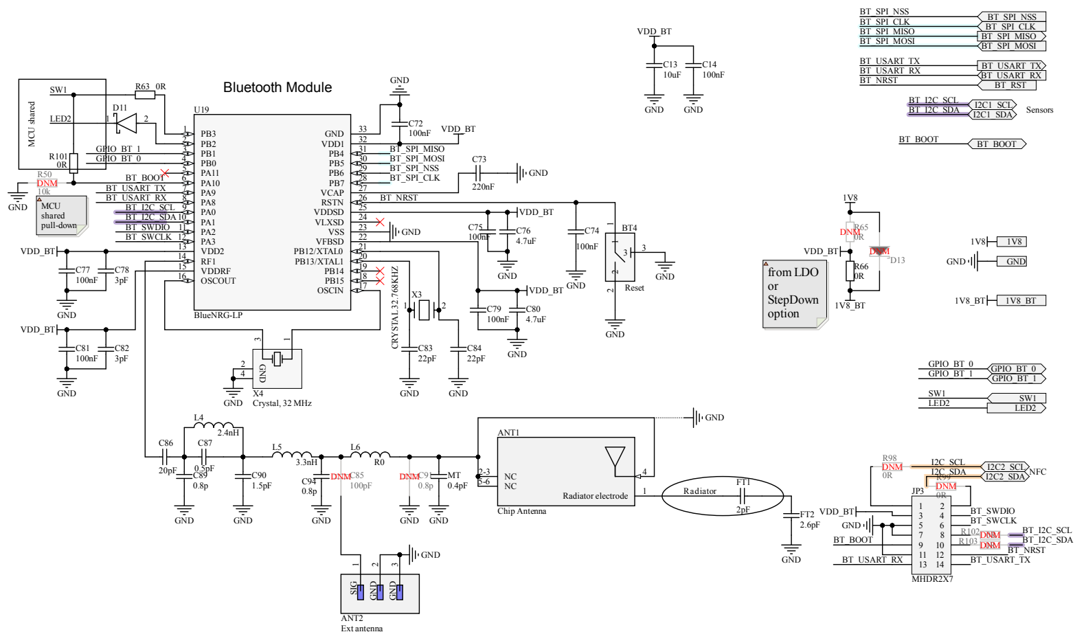
Figure 32. Sensortilebox_pro_BLE
