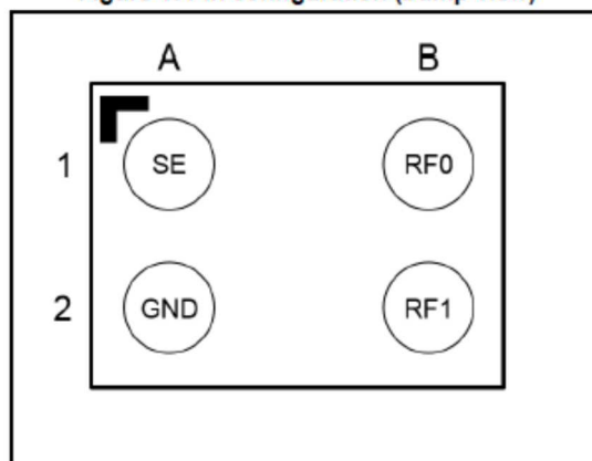
Figure 1: Pin configuration (bump view)
